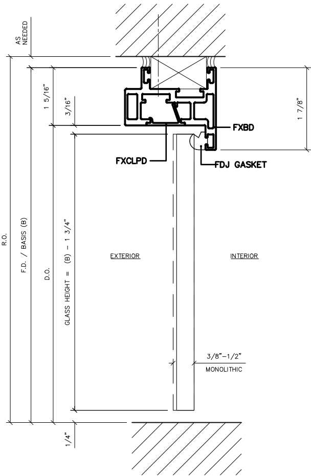
3 DOOR HEAD DETAIL W/O TRANSOM 1'-0" = 1'-0" ARCH REF: -/-
