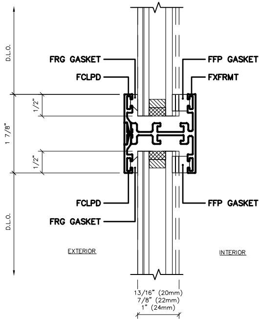
5 HORIZONTAL DETAIL @ FRAME XL 20-24.76 1'-0" = 1'-0" ARCH REF: -/-
