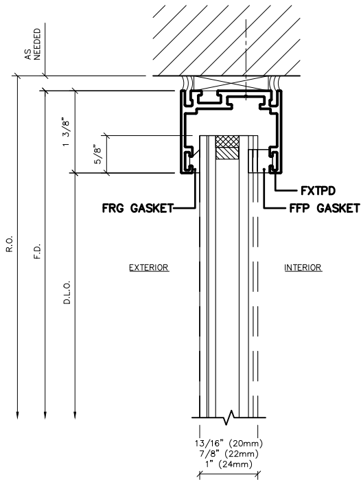
1 HEAD DETAIL @ FRAME XL 20-24.76 1'-0" = 1'-0" ARCH REF: -/-
