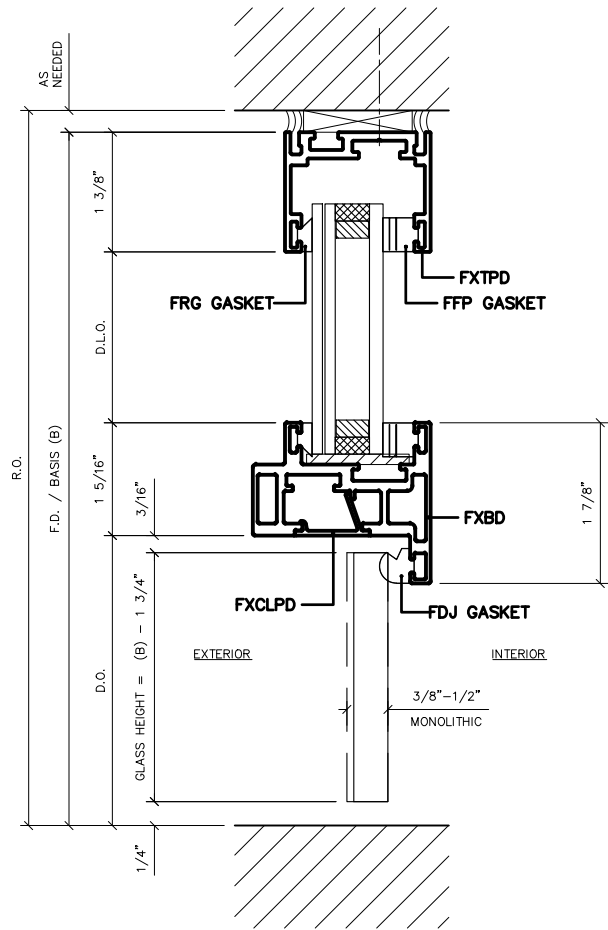
4 DOOR HEAD DETAIL W/ TRANSOM 1'-0" = 1'-0" ARCH REF: -/-
