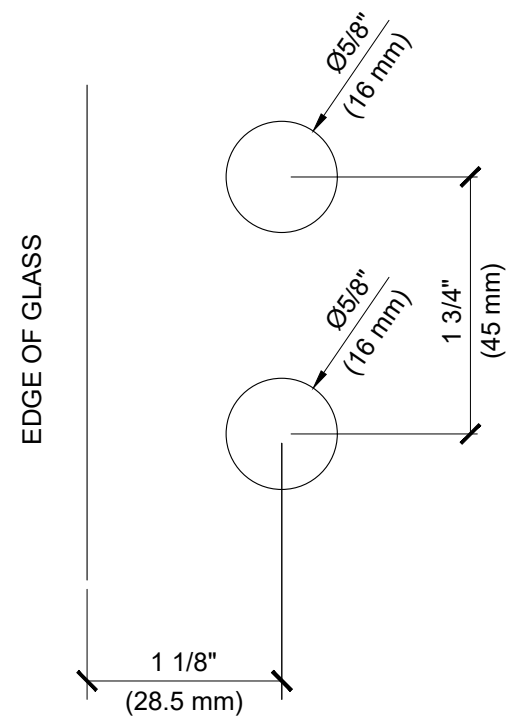
4 FDHDxx HINGE FDHSxx HINGE N.T.S. ARCH. REF.:
