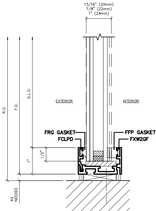
2 SILL DETAIL @ FRAME XL 20-24.76 1'-0" = 1'-0" ARCH REF: -/-
