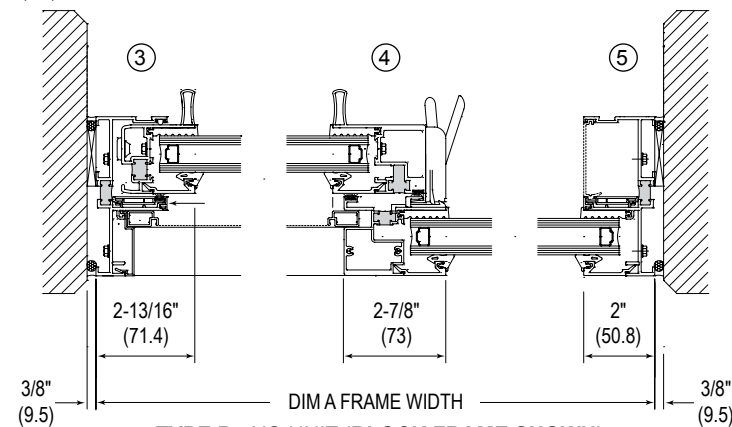
TYPE B XO UNIT (BLOCK FRAME SHOWN)
