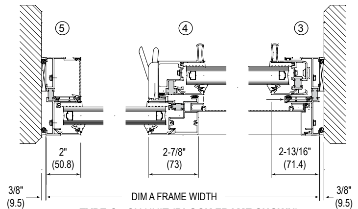
TYPE C OX UNIT (BLOCK FRAME SHOWN)
