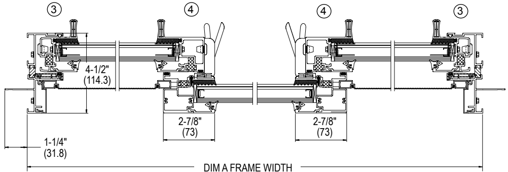
TYPE A XO UNIT (FIN FRAME SHOWN)
