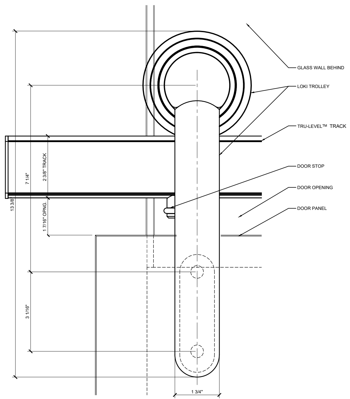
③ DOOR SLIDER ELEVATION ARCH REF: 1'-0"=1'-0"
