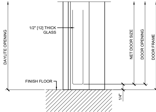
④ SWING IN DOOR SILL DETAIL ARCH REF: NONE 1'-0"=1'-0"
