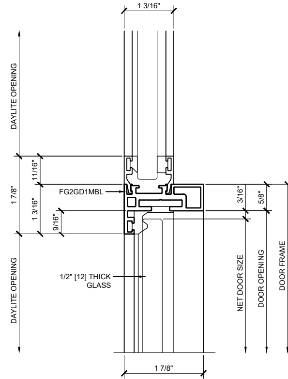
⑤ TRANSOM DETAIL ARCH REF: NONE 1'-0"=1'-0"
