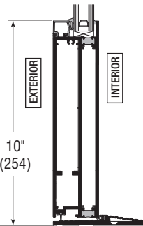
TYPE B 10" BOTTOM RAIL AND 1/2" LOW PROFILE THRESHOLD SHOWN
