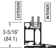
TYPE C STANDARD BOTTOM RAIL AND 1/2" LOW PROFILE THRESHOLD SHOWN
