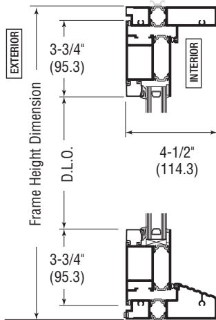
TYPE A STANDARD BOTTOM RAIL AND THRESHOLD SHOWN
