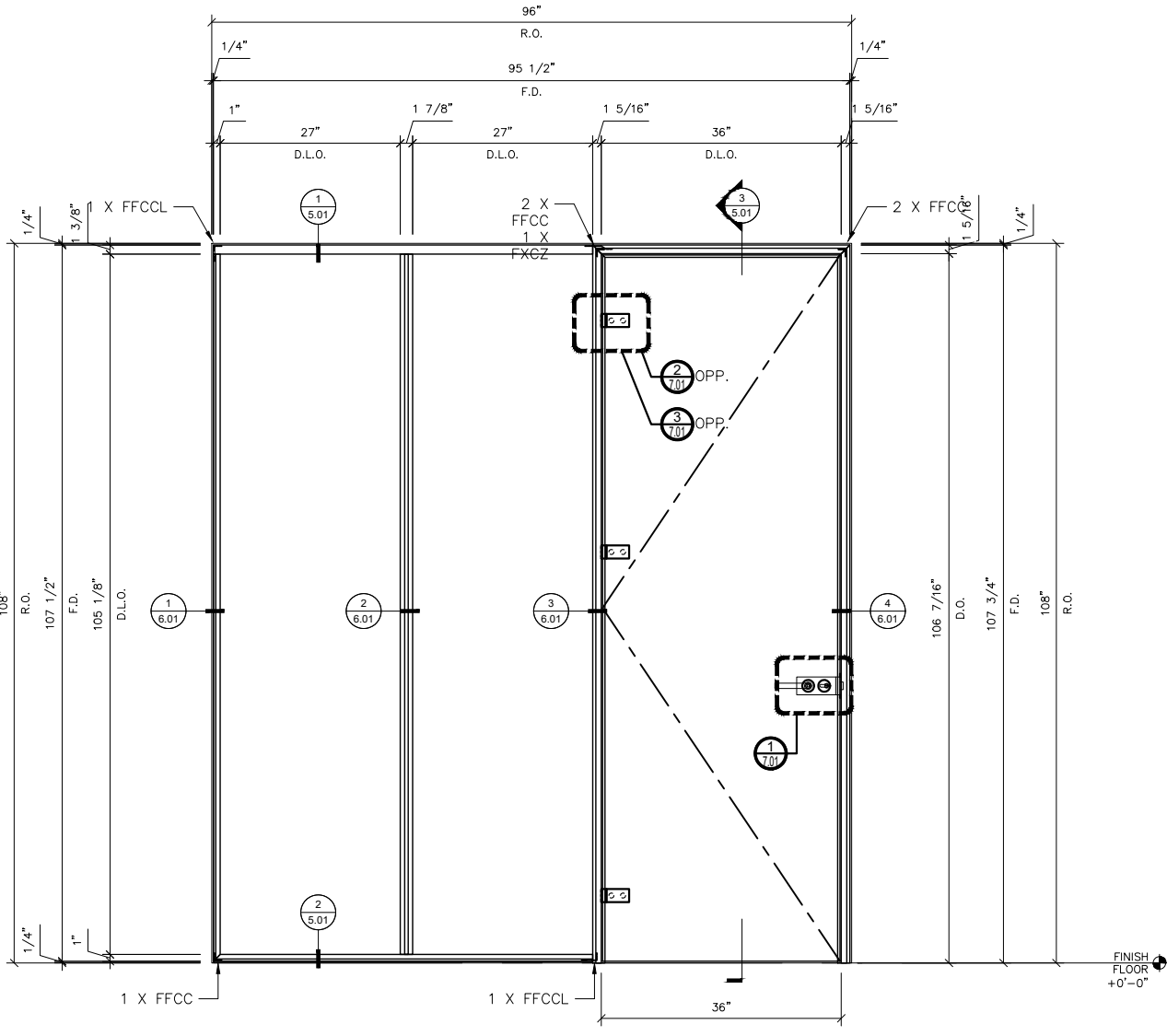
2 FALLBROOK XL SERIES ELEVATION W/O TRANSOM 1" = 1'-0" ARCH. REF: -/-
