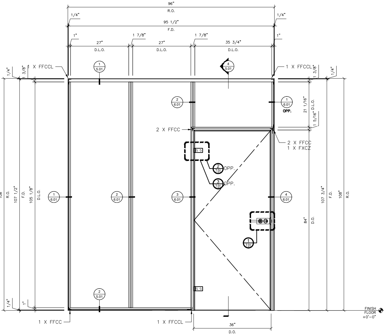
1 FALLBROOK XL SERIES ELEVATION W/ TRANSOM 1" = 1'-0" ARCH. REF: -/-
