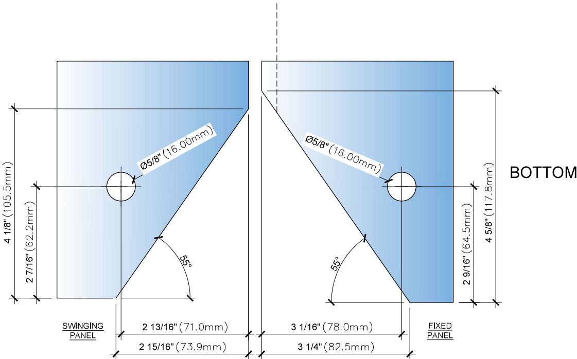
3A GLASS CUT OUT DETAIL - 1MM FIXED PANEL GAP ARCH REF: SCALE: 1'-0"=1'-0"
