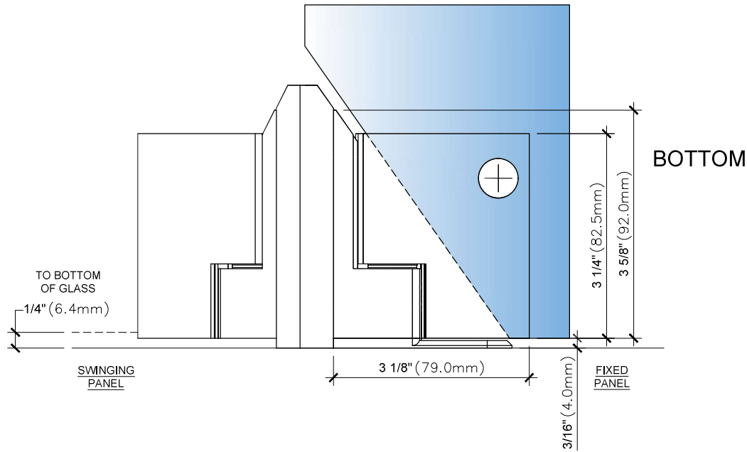
2A SIDE VIEW DETAIL @1MM FIXED PANEL GAP ARCH REF: SCALE: 1'-0"=1'-0"
