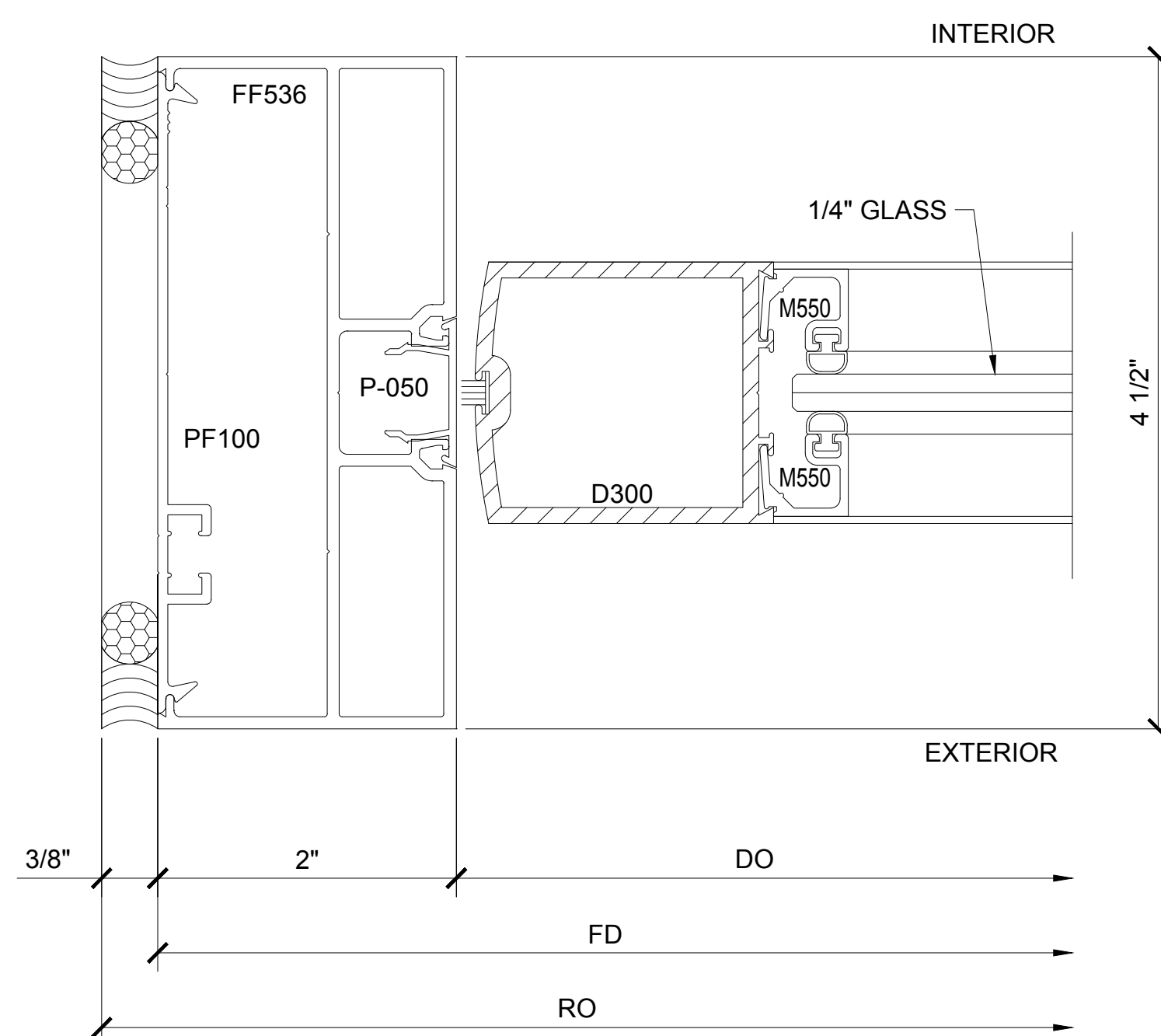
SECTION DETAIL AT DOOR JAMB
