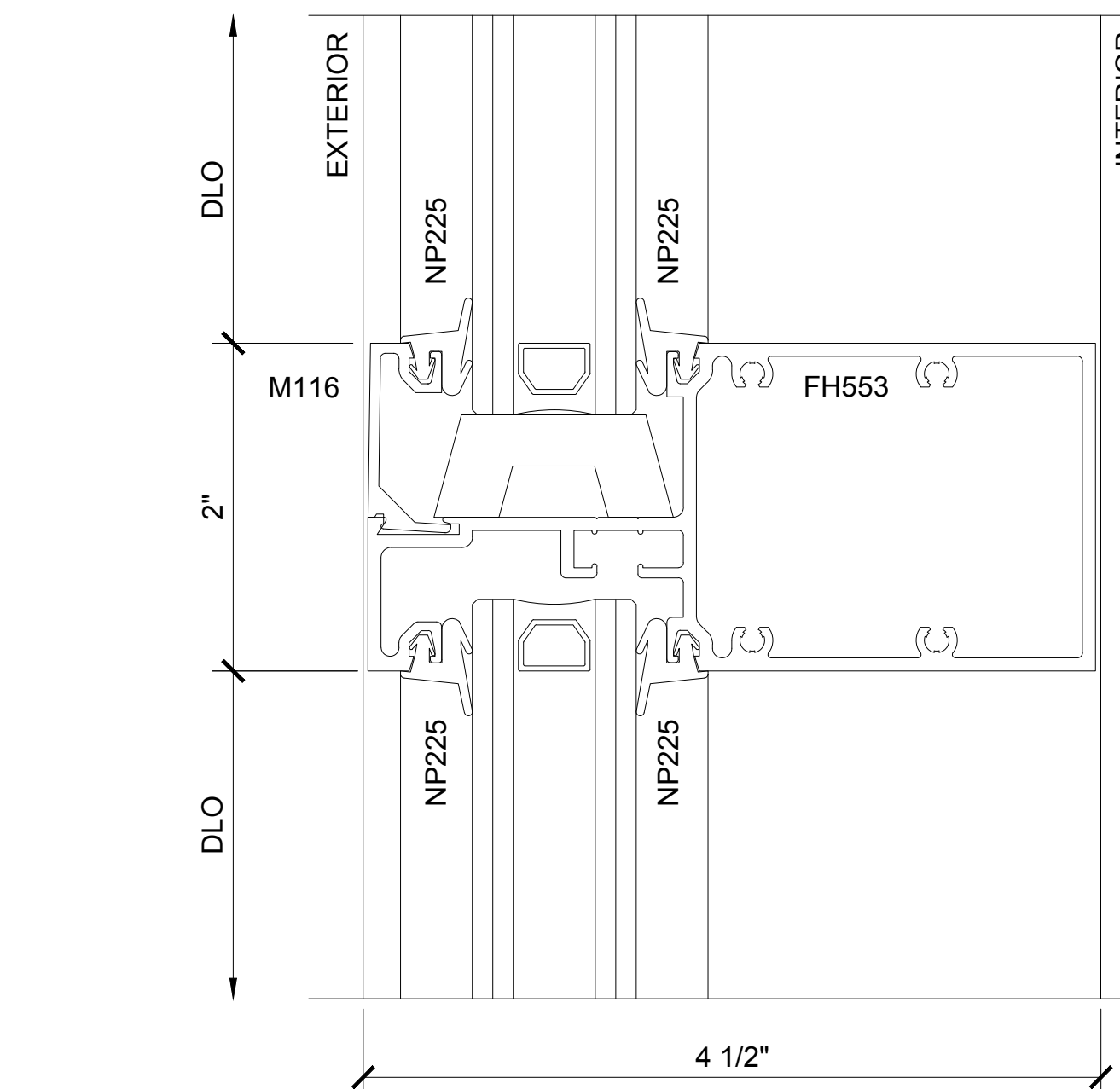
SECTION DETAIL AT INTERMEDIATE HORIZONTAL
