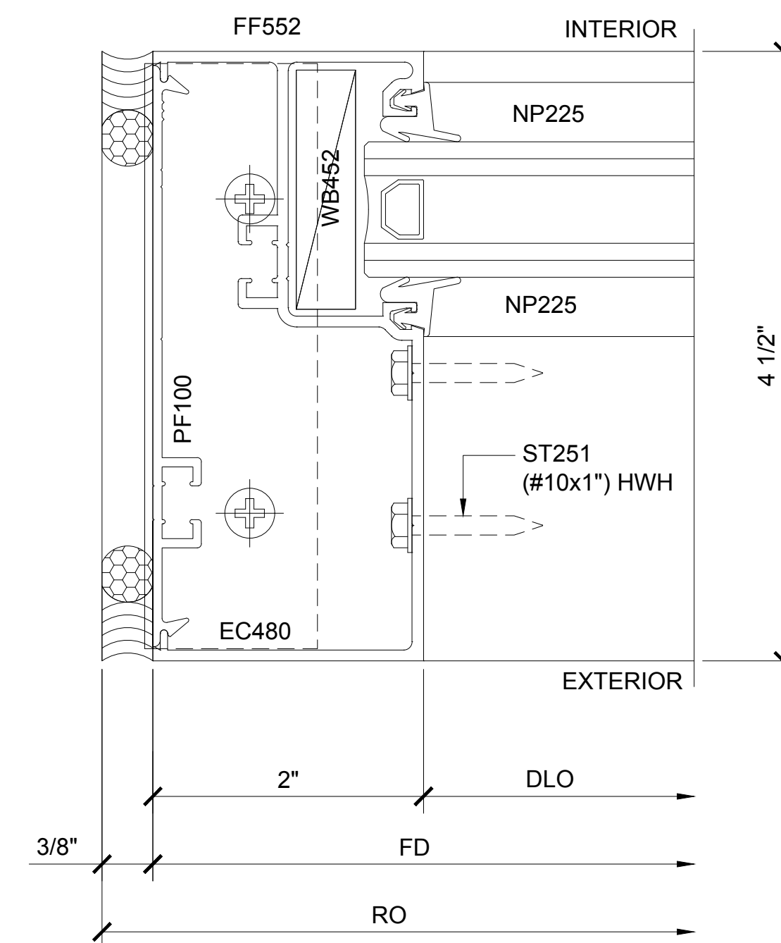
SECTION DETAIL AT JAMB
