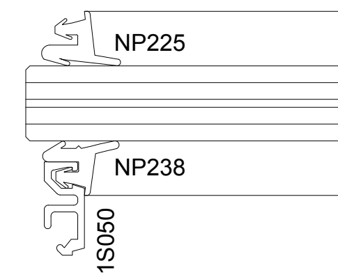
SECTION DETAIL AT FF451 - 9/16" GLASS (5)
