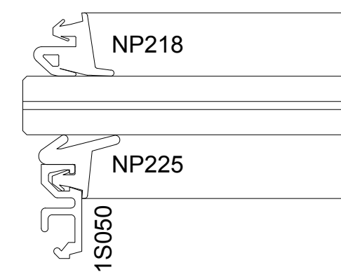
SECTION DETAIL AT FF451 - 7/16" GLASS (3)
