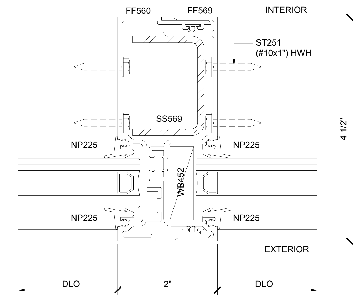
SECTION DETAIL AT EXPANSION VERTICAL
