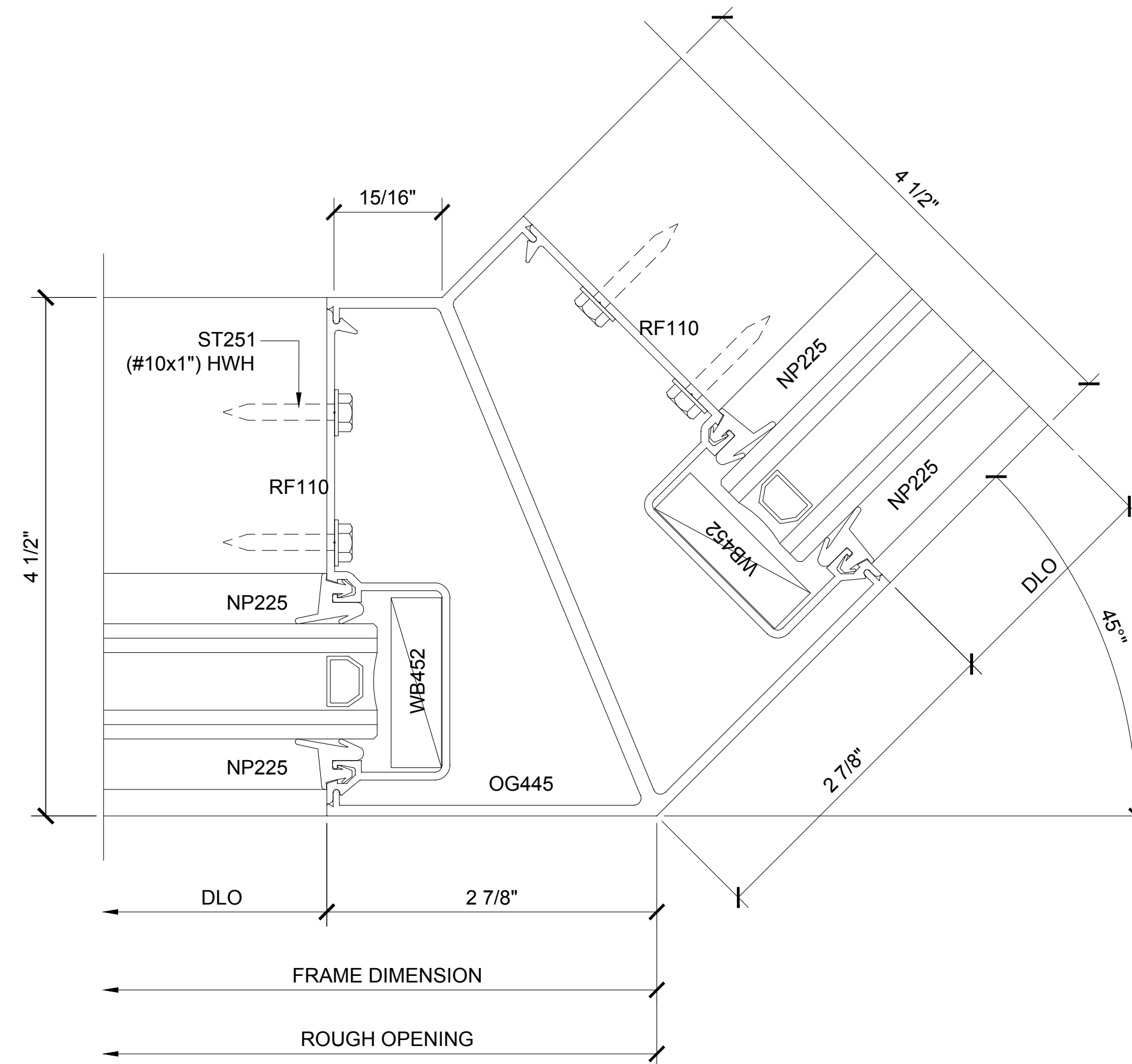
SECTION DETAIL @ JAMB - 135° ②
