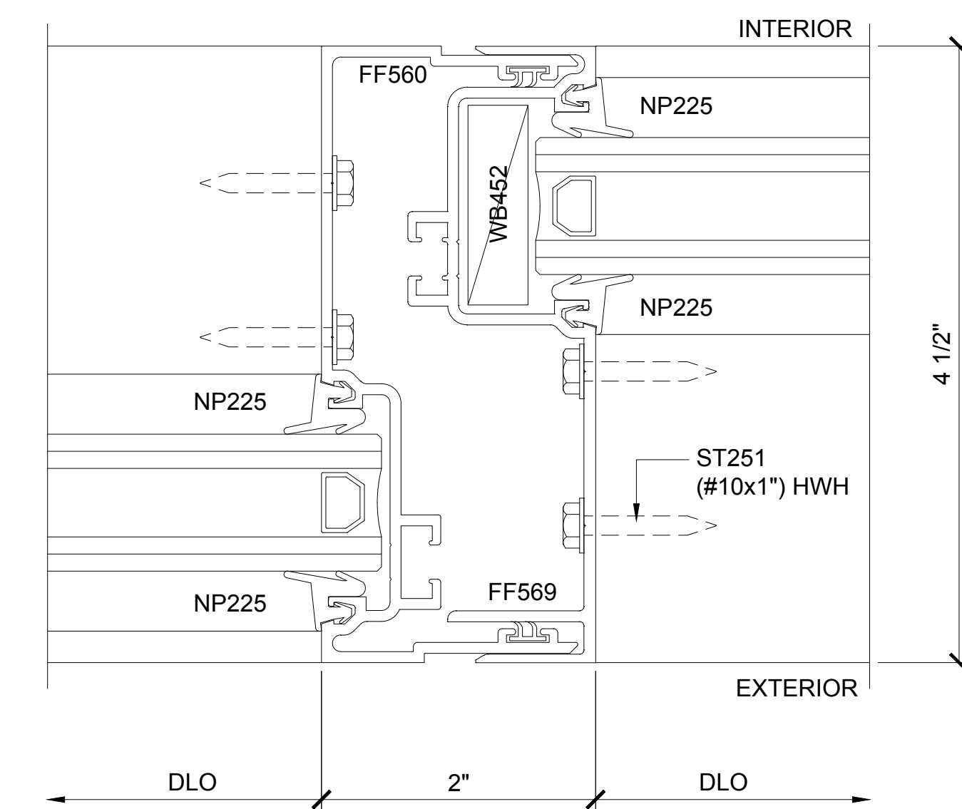
SECTION DETAIL AT EXPANSION VERTICAL
