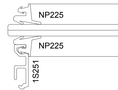
SECTION DETAIL AT FF451 - 1/4" GLASS
