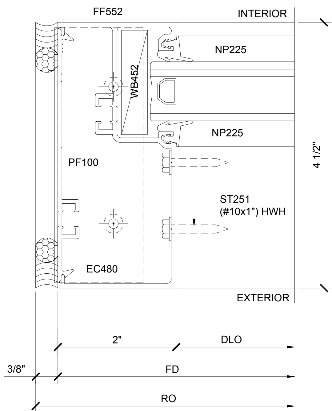
SECTION DETAIL AT JAMB 5
