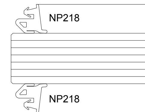
SECTION DETAIL AT FF451 - 7/8" GLASS (7)
