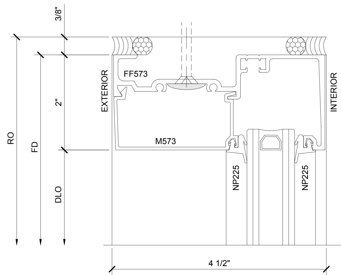
SECTION DETAIL AT HEAD 1
