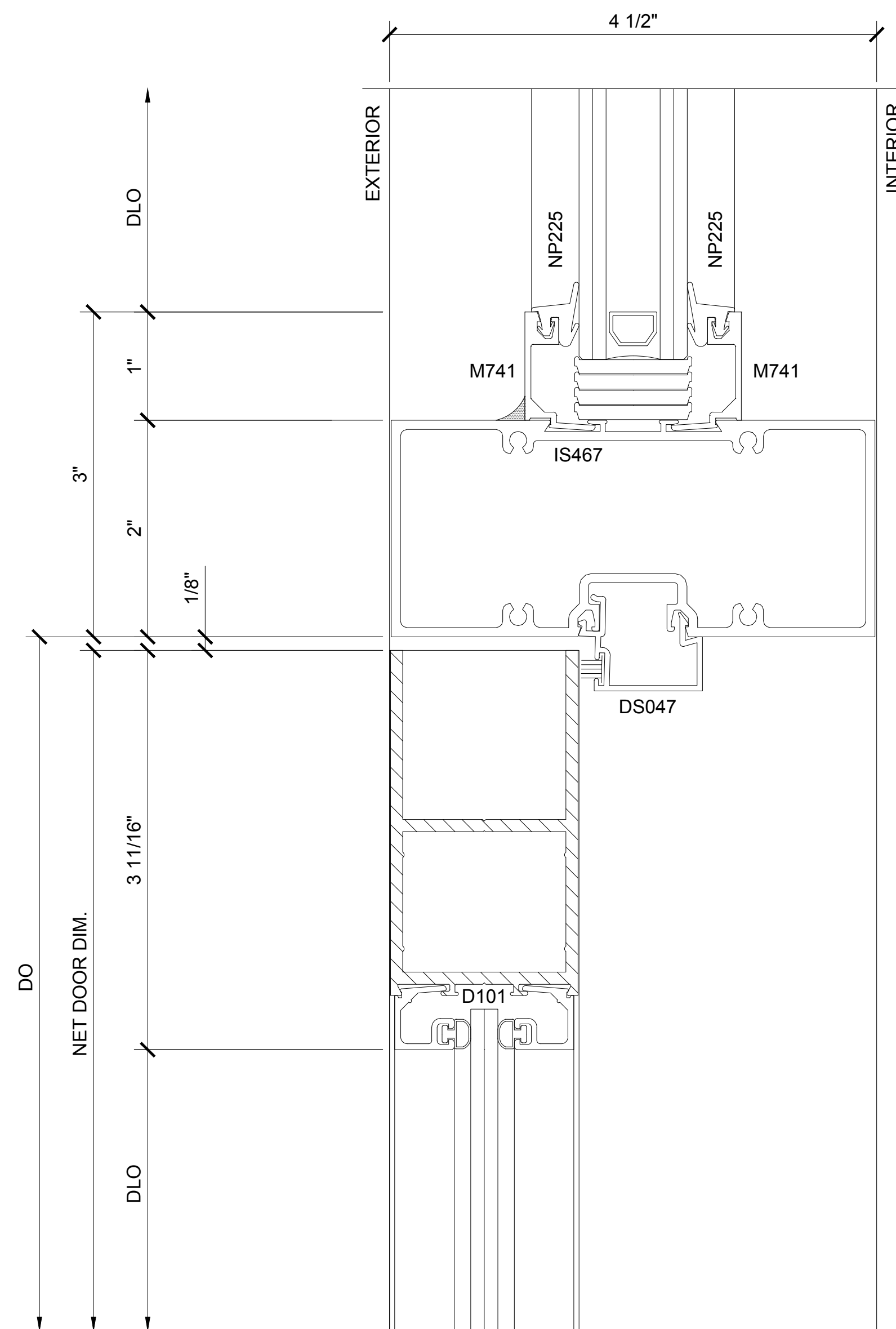
SECTION DETAIL AT DOOR HEAD
