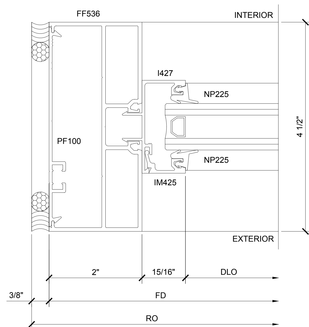
SECTION DETAIL AT JAMB
