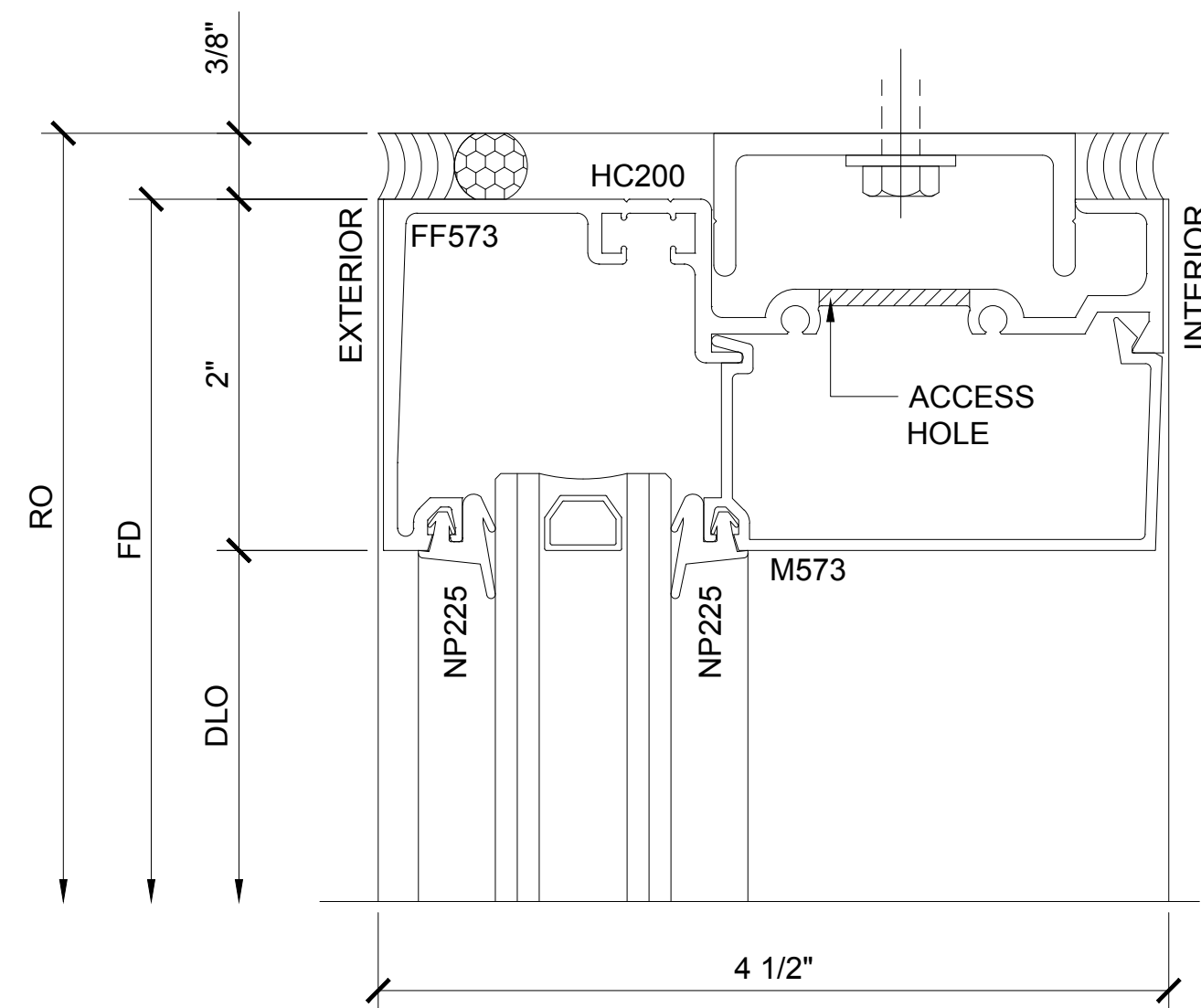
SECTION DETAIL AT HEAD
