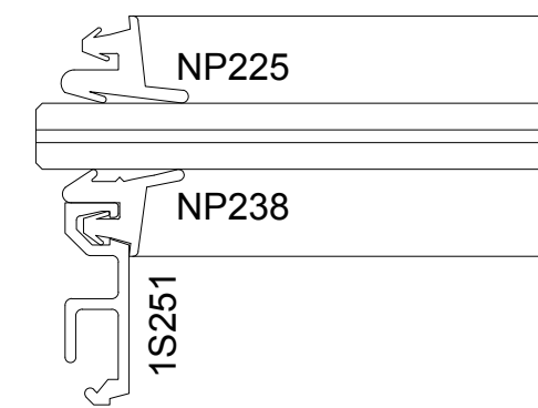
SECTION DETAIL AT FF451 - 5/16" GLASS (2)
