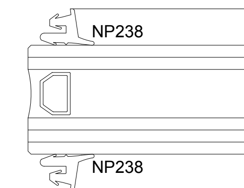
SECTION DETAIL AT FF451 - 1-1/8" GLASS (11)
