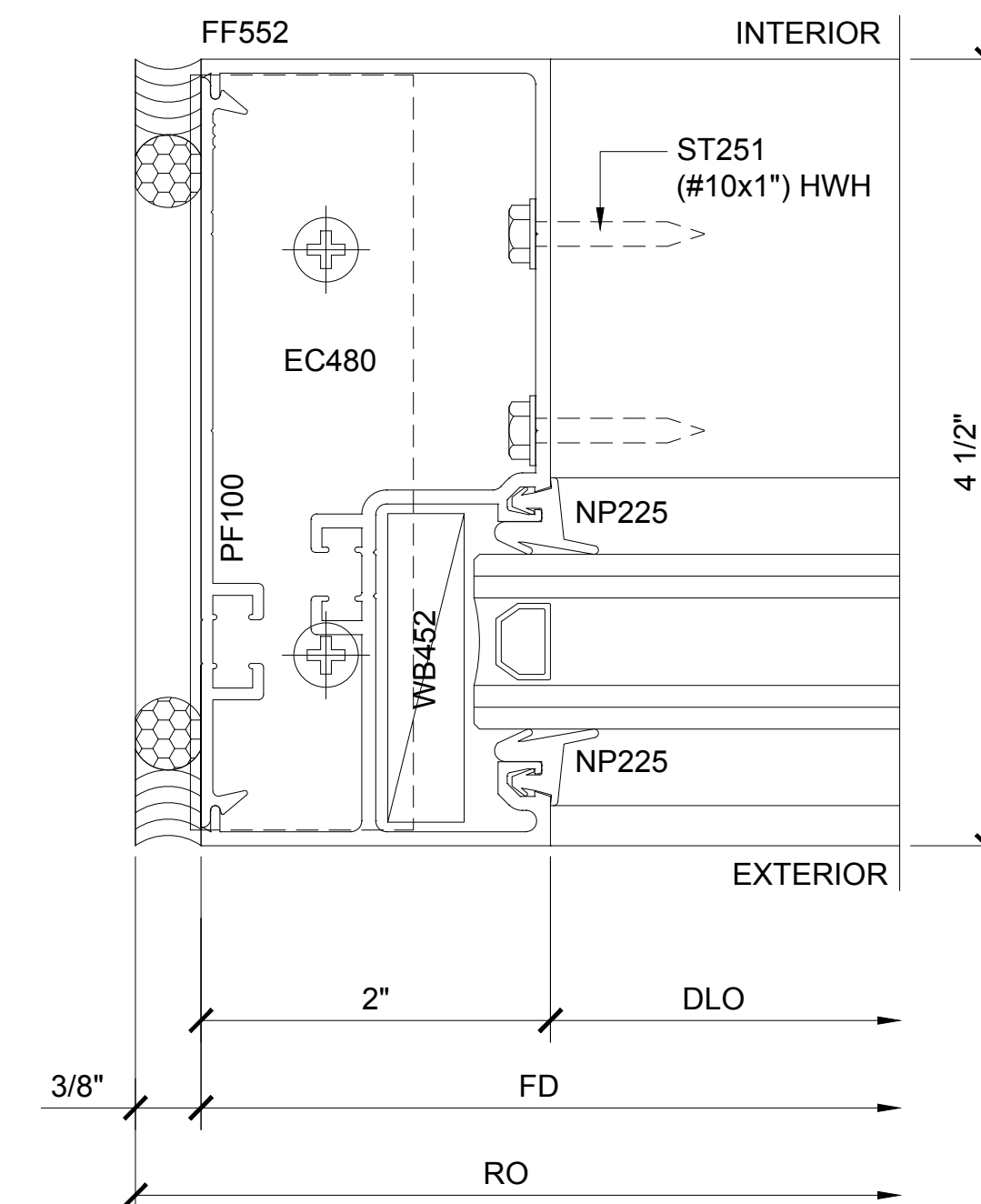
SECTION DETAIL AT JAMB
