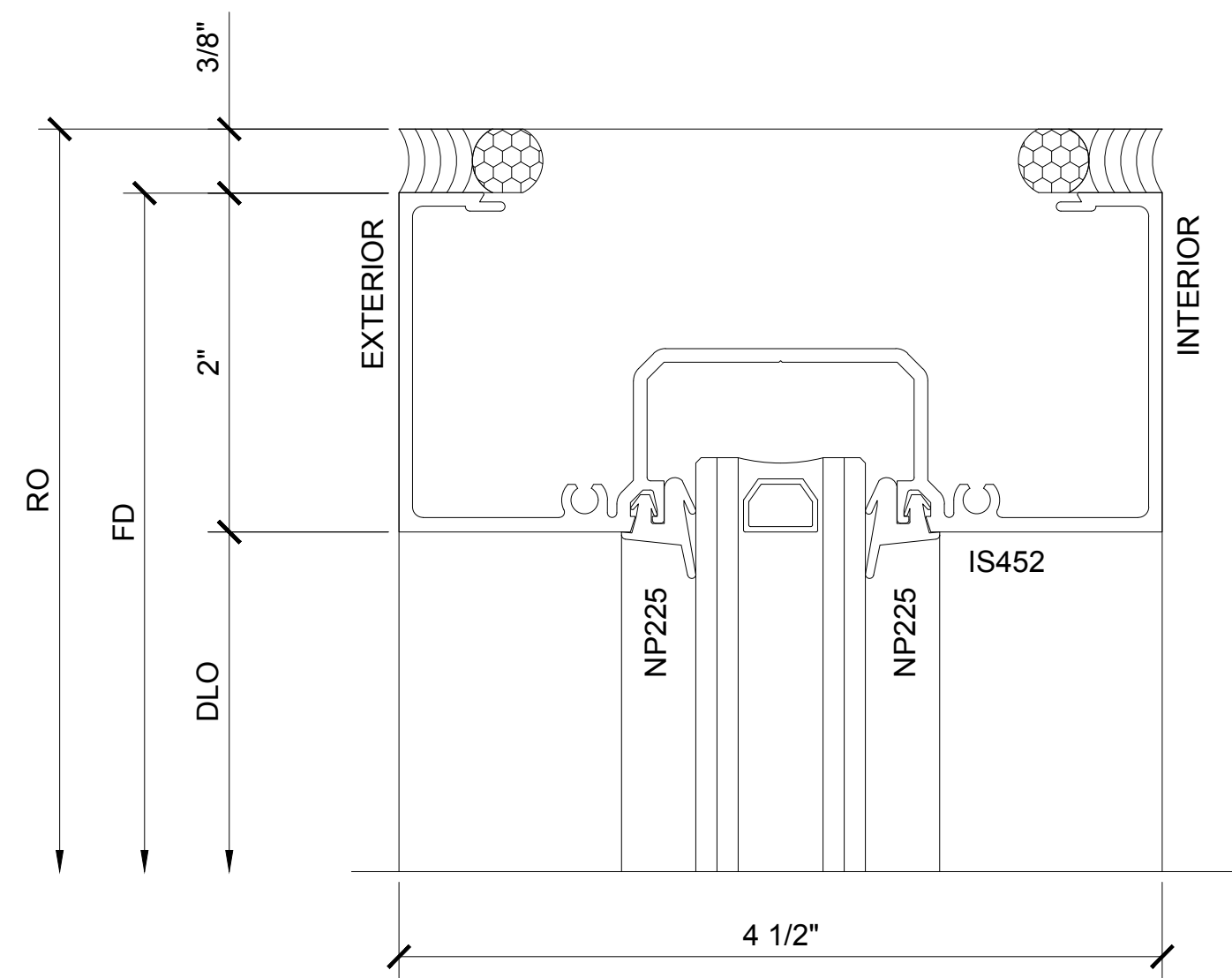
SECTION DETAIL AT HEAD
