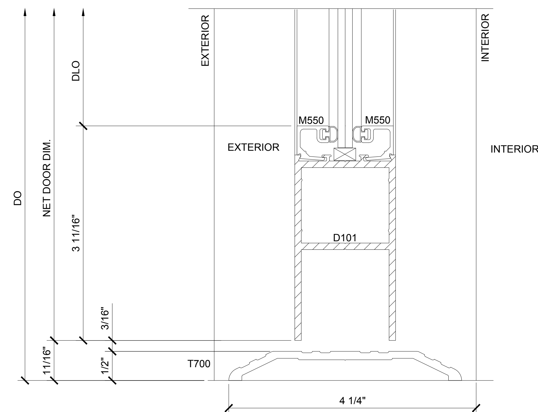
SECTION DETAIL AT BOTTOM RAIL
