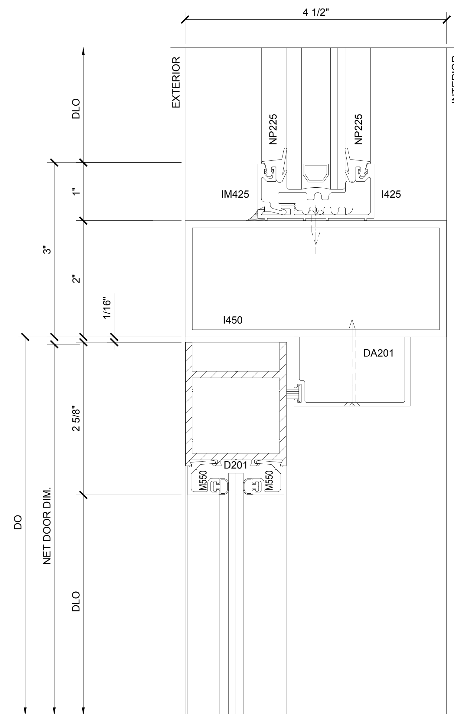
SECTION DETAIL AT DOOR HEAD
