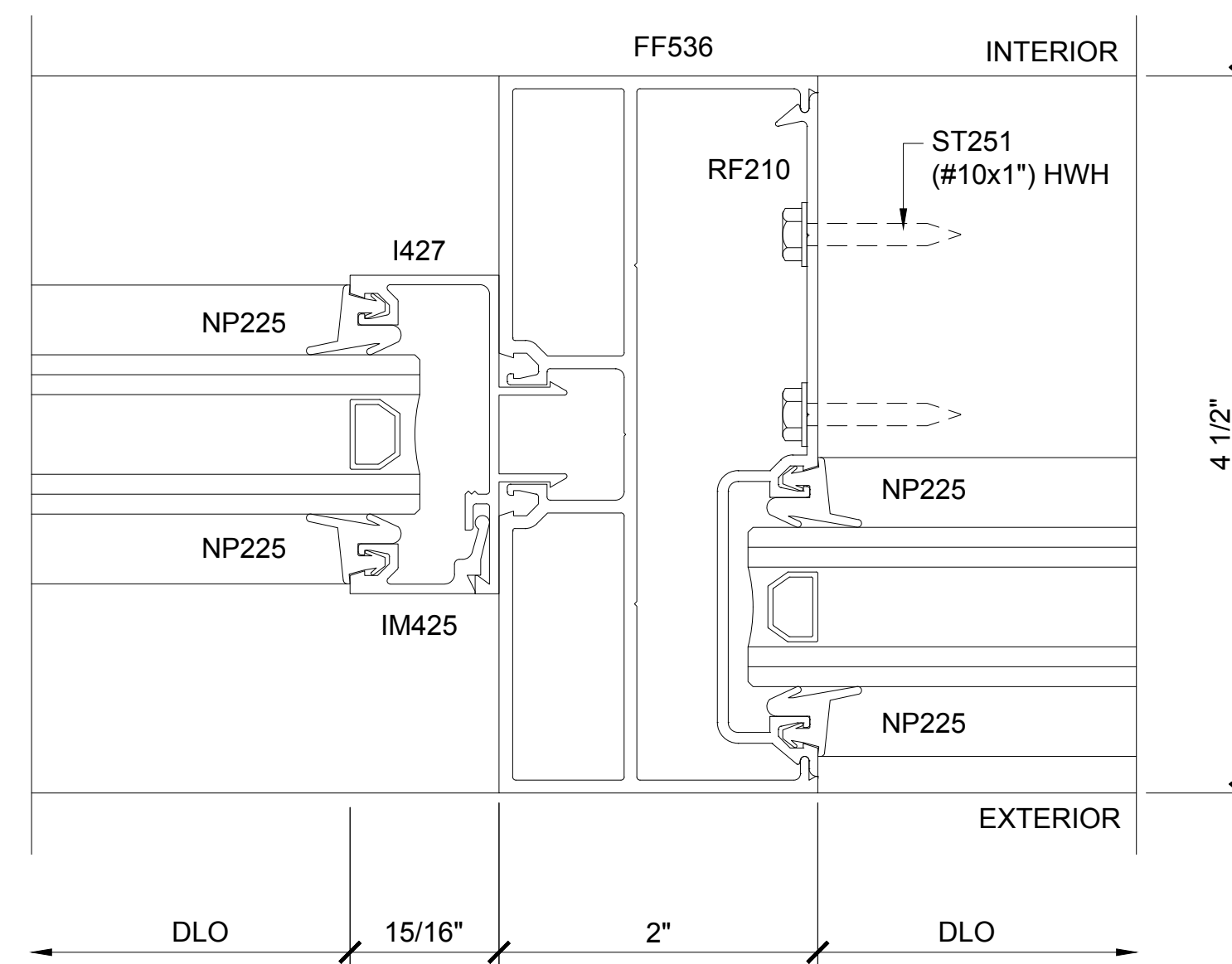
SECTION DETAIL AT INTERMEDIATE VERTICAL
