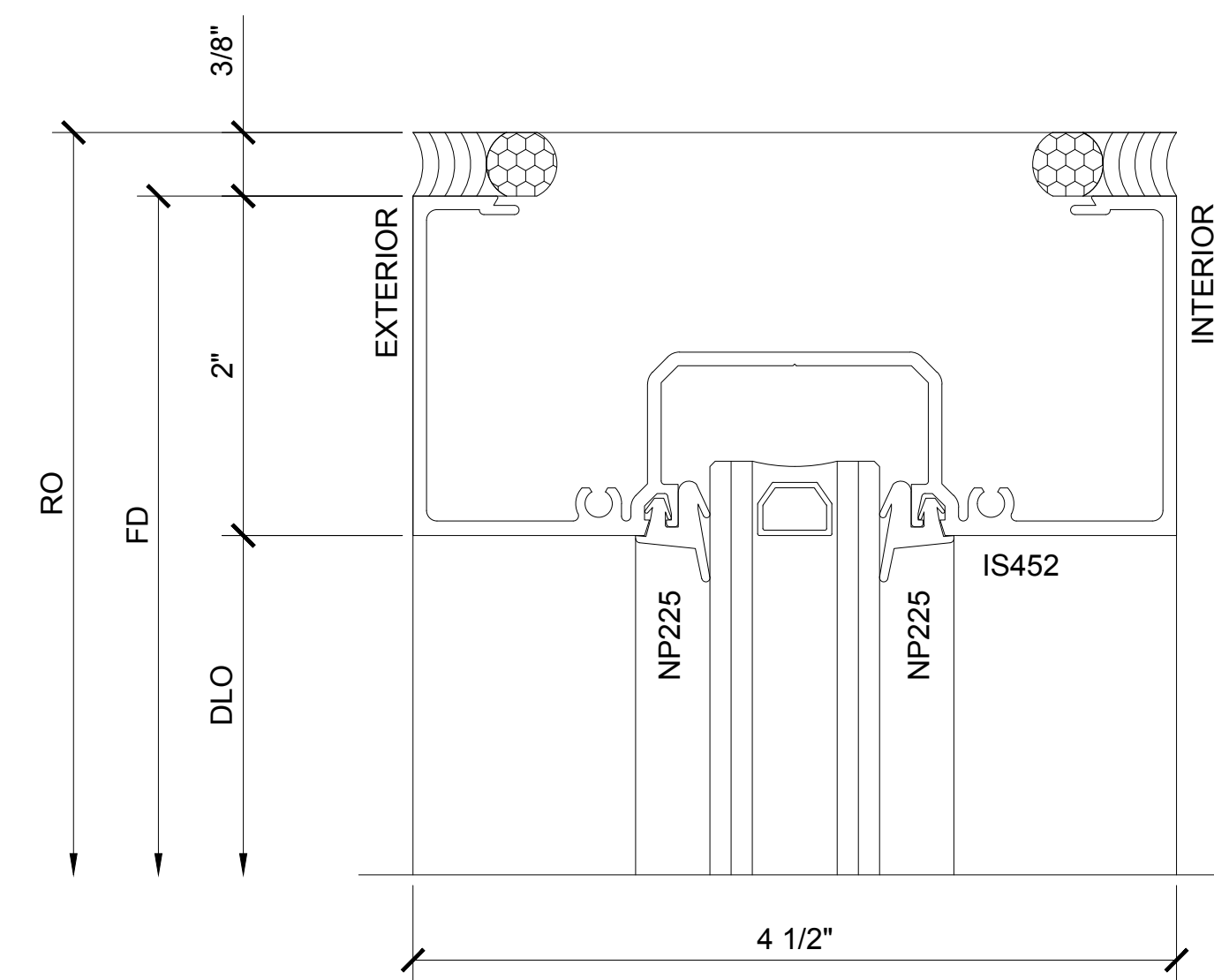
SECTION DETAIL AT HEAD
