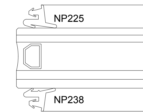
SECTION DETAIL AT FF451 - 1-5/16" GLASS (10)
