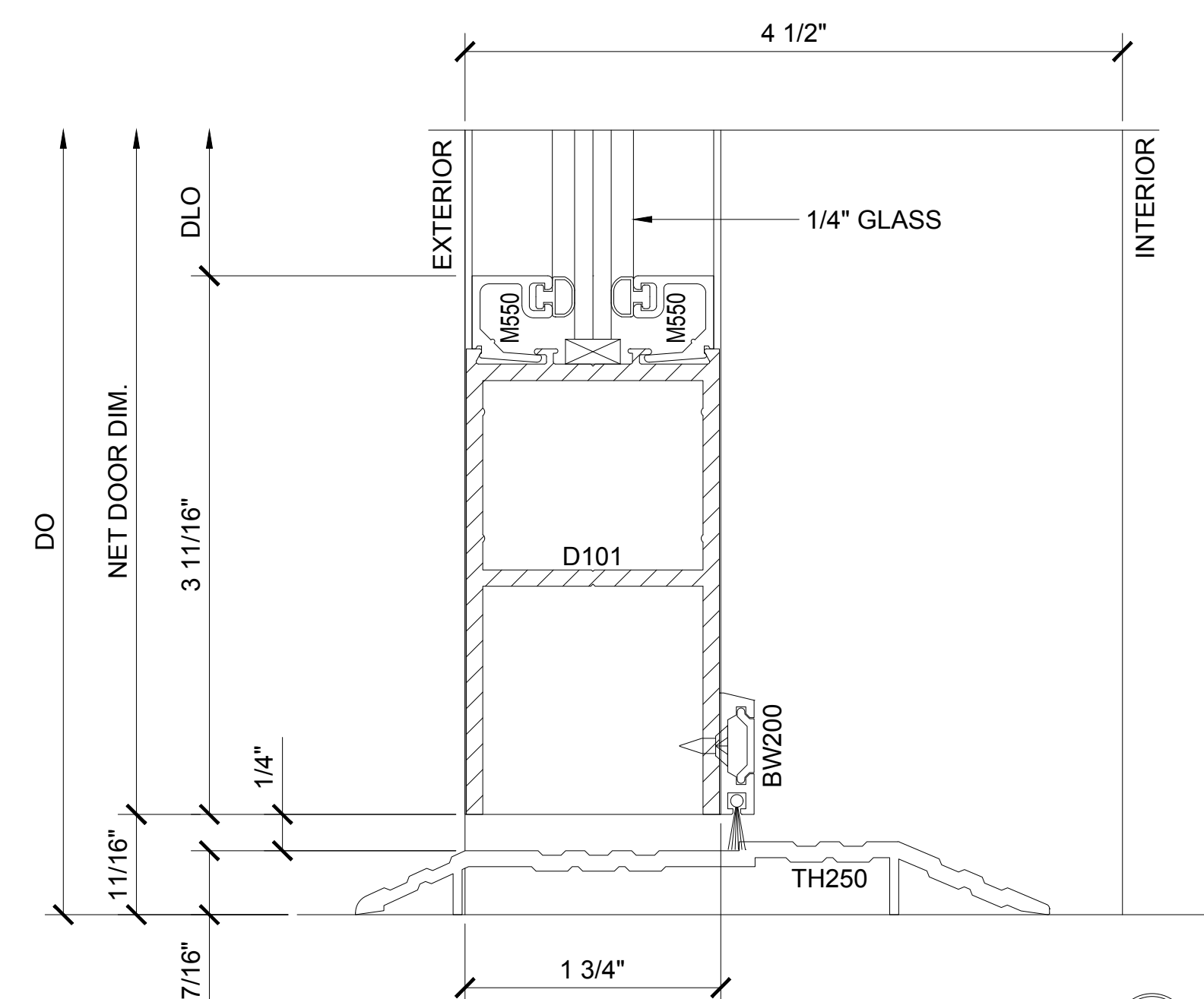
SECTION DETAIL AT BOTTOM RAIL
