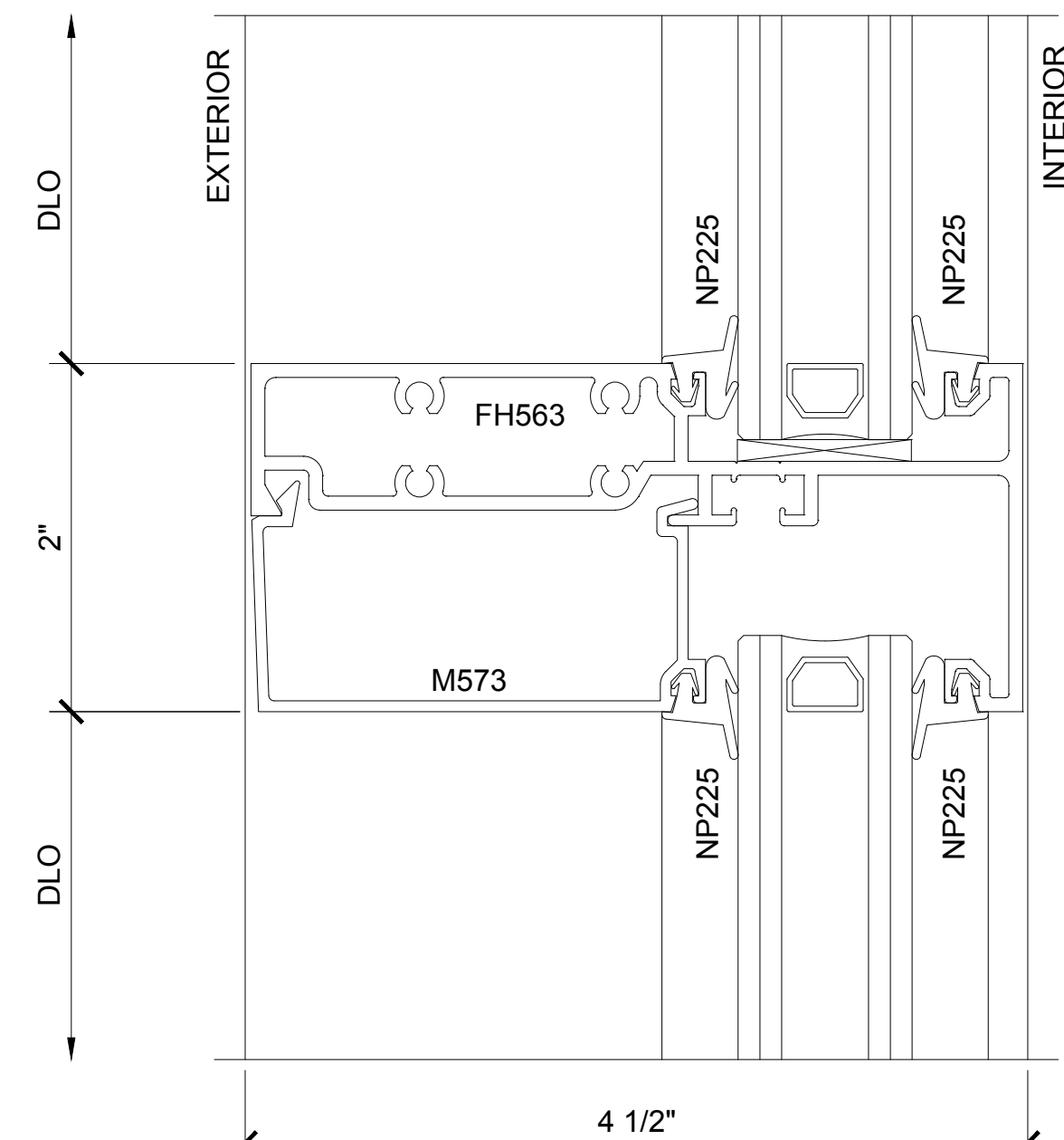
SECTION DETAIL AT INTERMEDIATE HORIZONTAL
