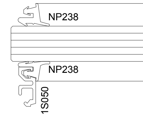
SECTION DETAIL AT FF451 - 5/8" GLASS 6
