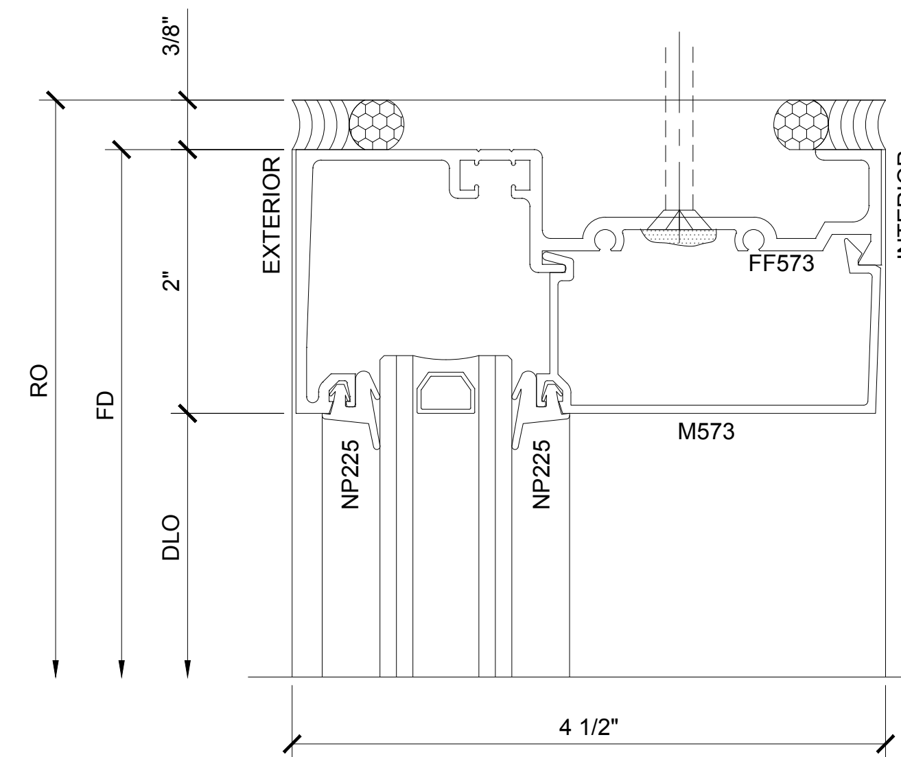
SECTION DETAIL AT HEAD W/ HEAD ANCHOR
