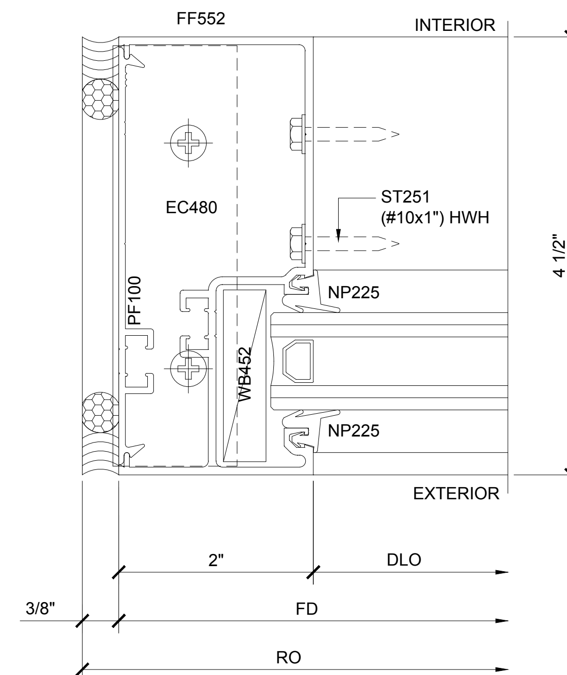
SECTION DETAIL AT JAMB
