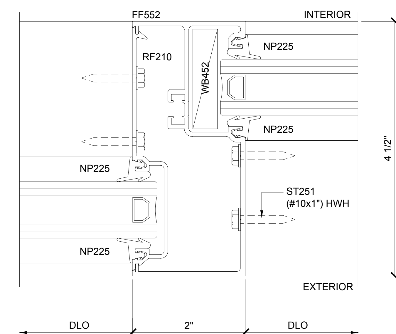
SECTION DETAIL AT HOLLOW INTERMEDIATE VERTICAL
