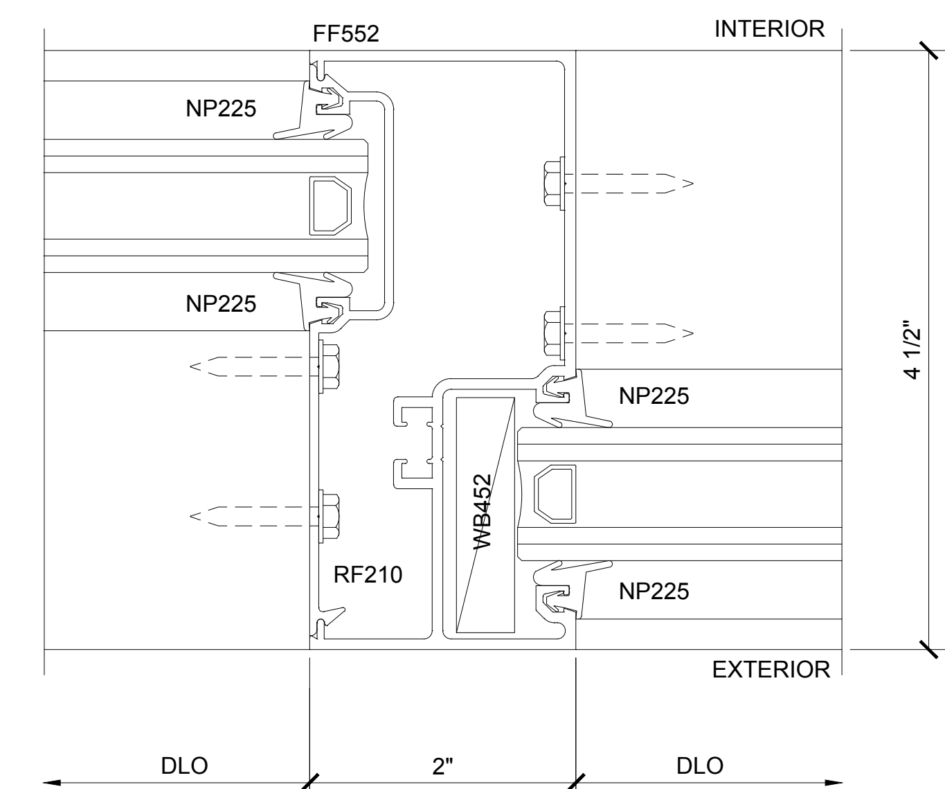
SECTION DETAIL AT HOLLOW INTERMEDIATE VERTICAL
