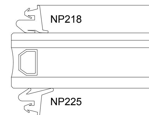
SECTION DETAIL AT FF451 - 15/16" GLASS
