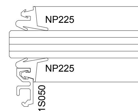
SECTION DETAIL AT FF451 - 1/2" GLASS 4
