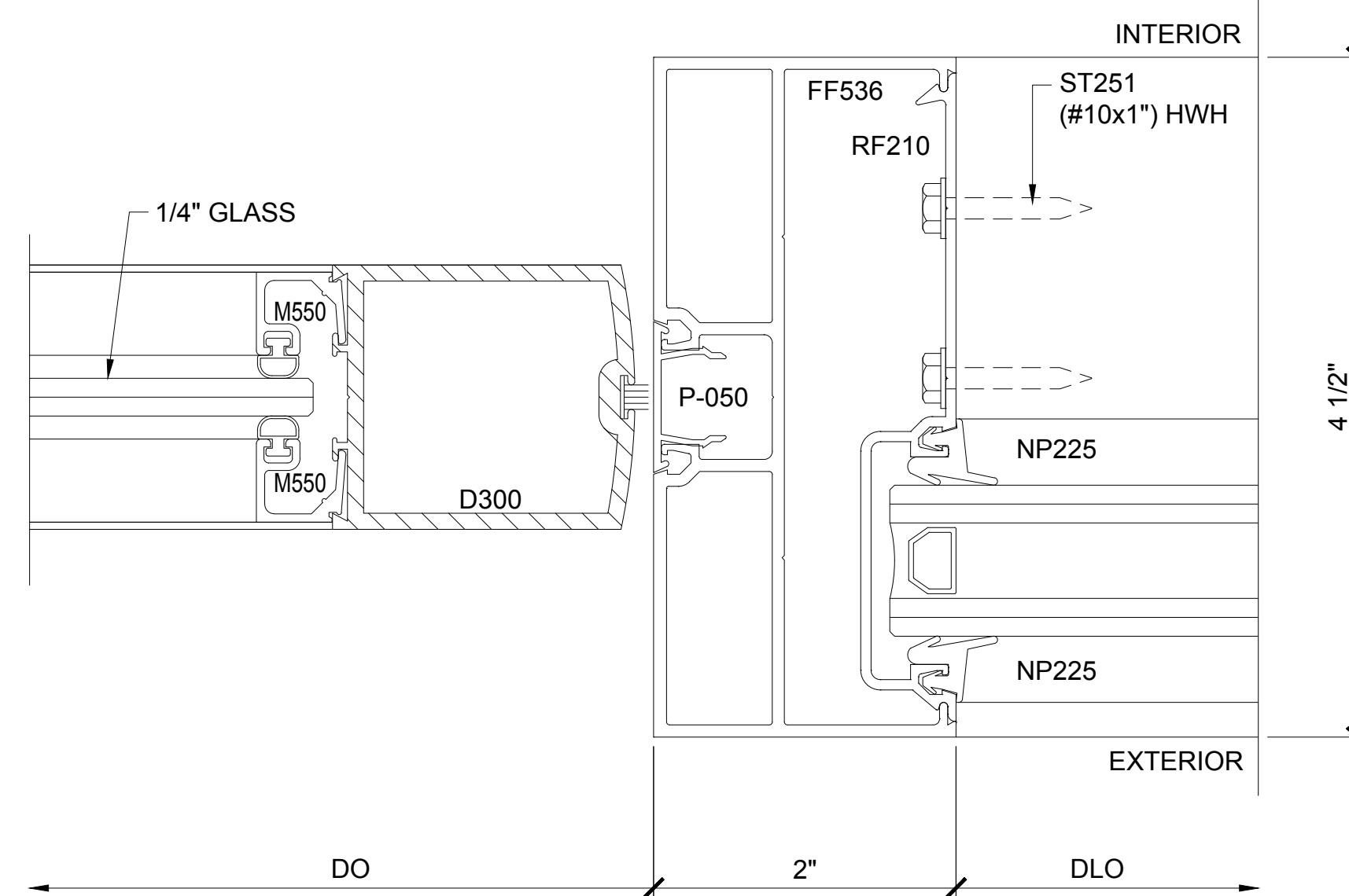
SECTION DETAIL AT INTERMEDIATE VERTICAL
