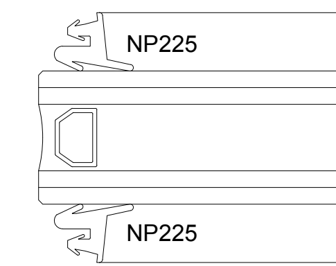
SECTION DETAIL AT FF451 - 1" GLASS 9
