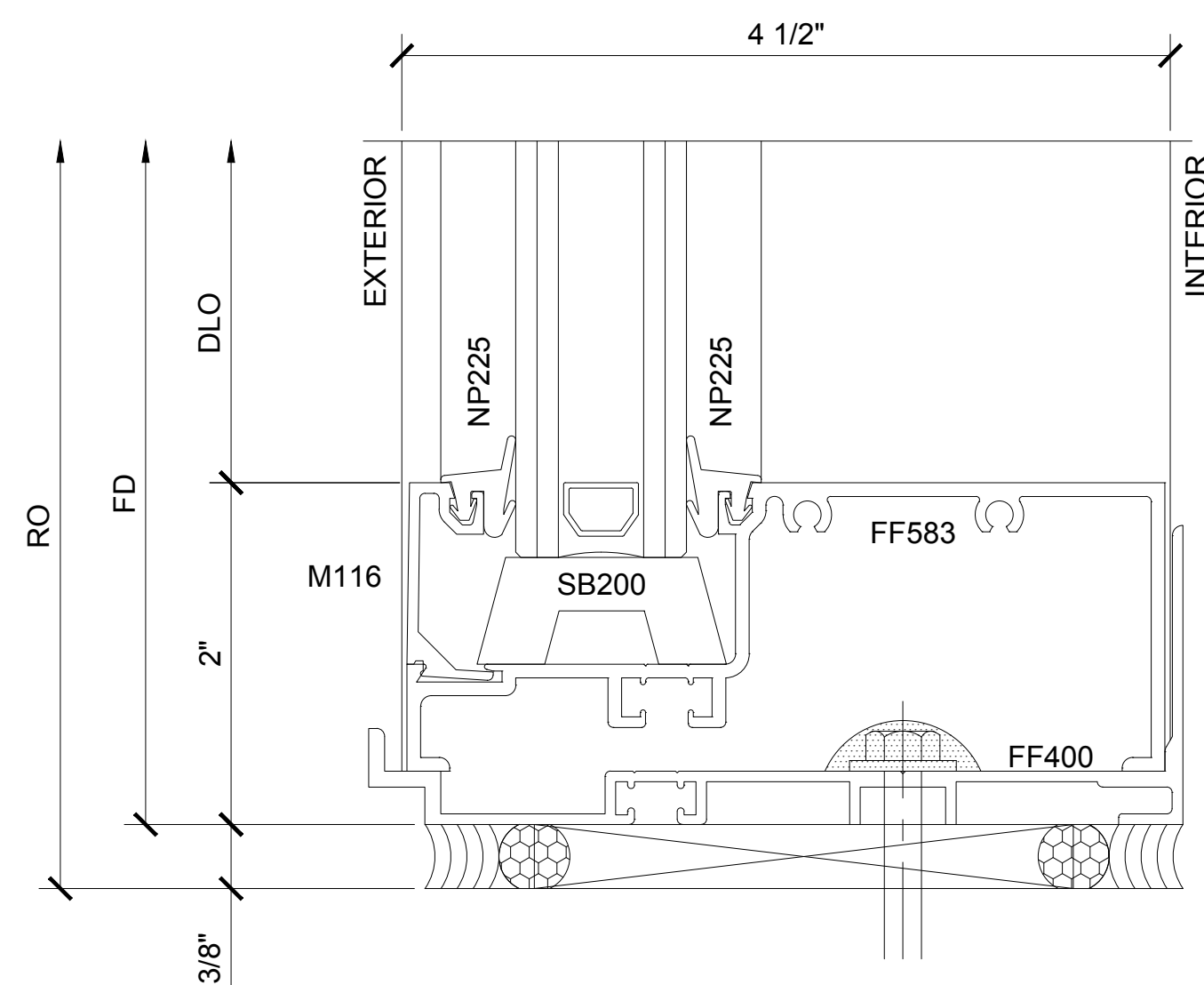
SECTION DETAIL AT SILL
