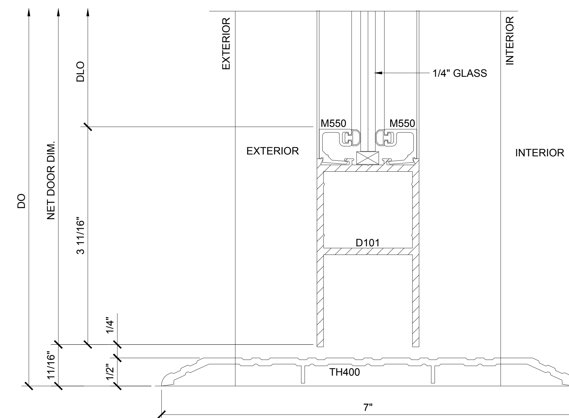
SECTION DETAIL AT BOTTOM RAIL
