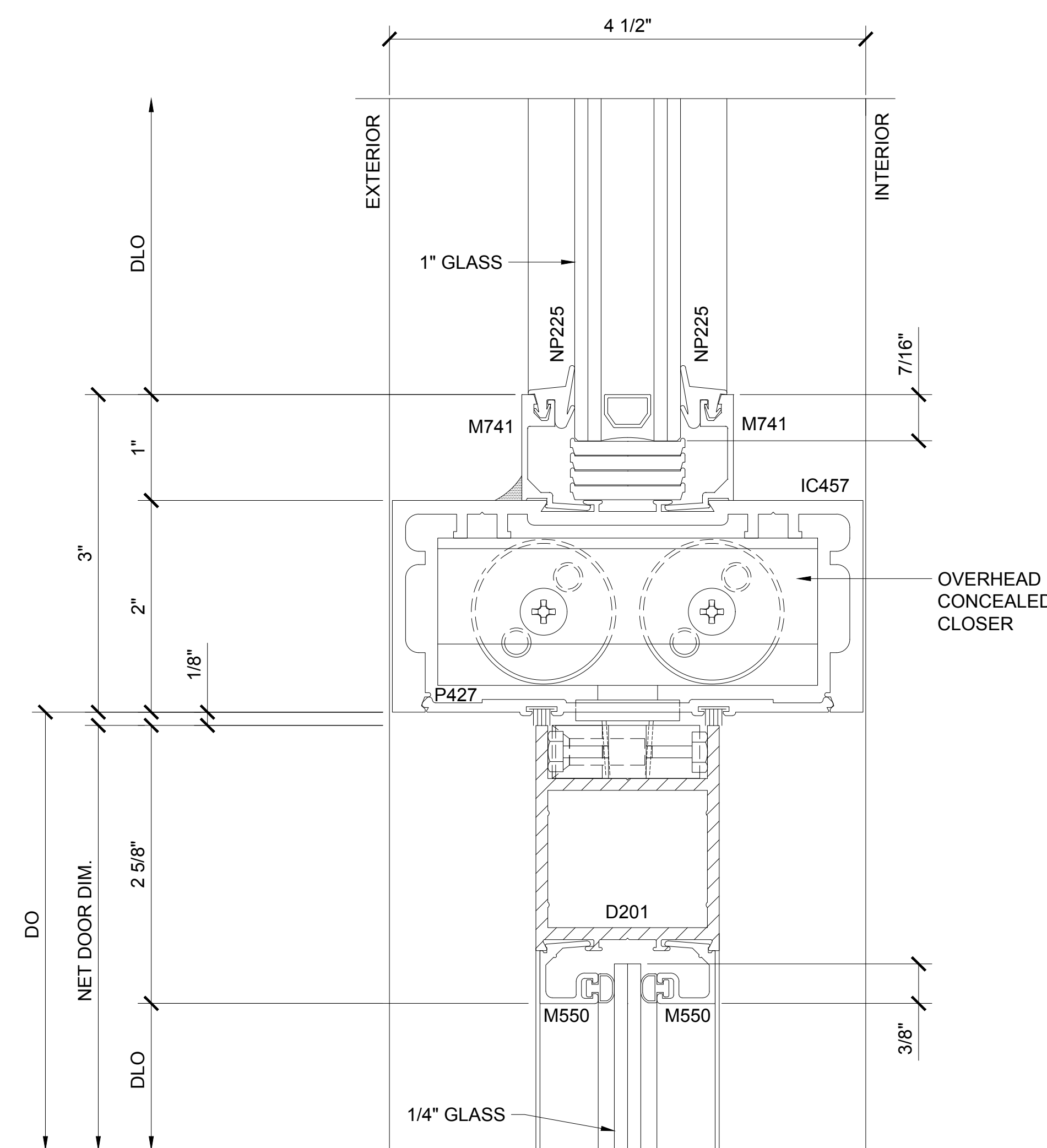
SECTION DETAIL AT DOOR HEAD WITH OHCC
