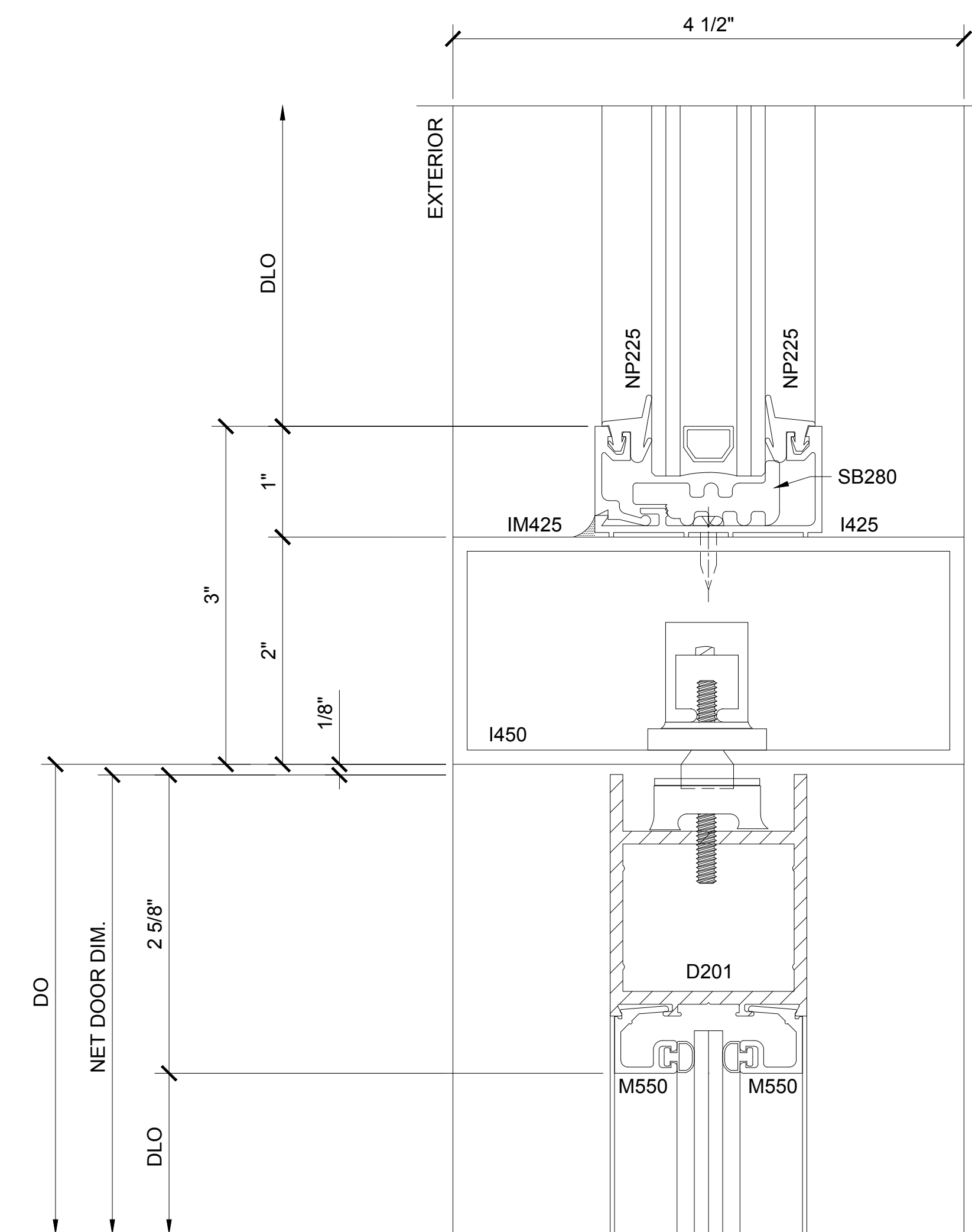
SECTION DETAIL AT DOOR HEAD WITH PIVOT
