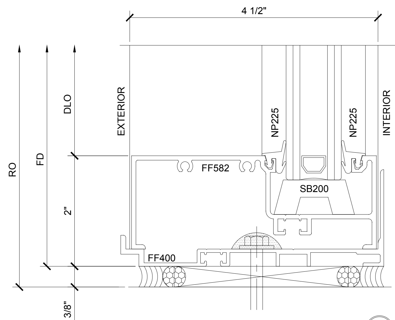
SECTION DETAIL AT SILL 3
