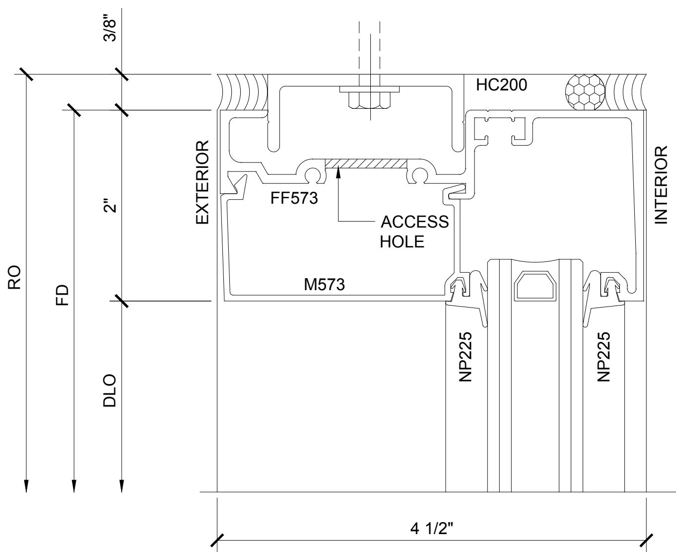
SECTION DETAIL AT HEAD W/ HEAD ANCHOR 4
