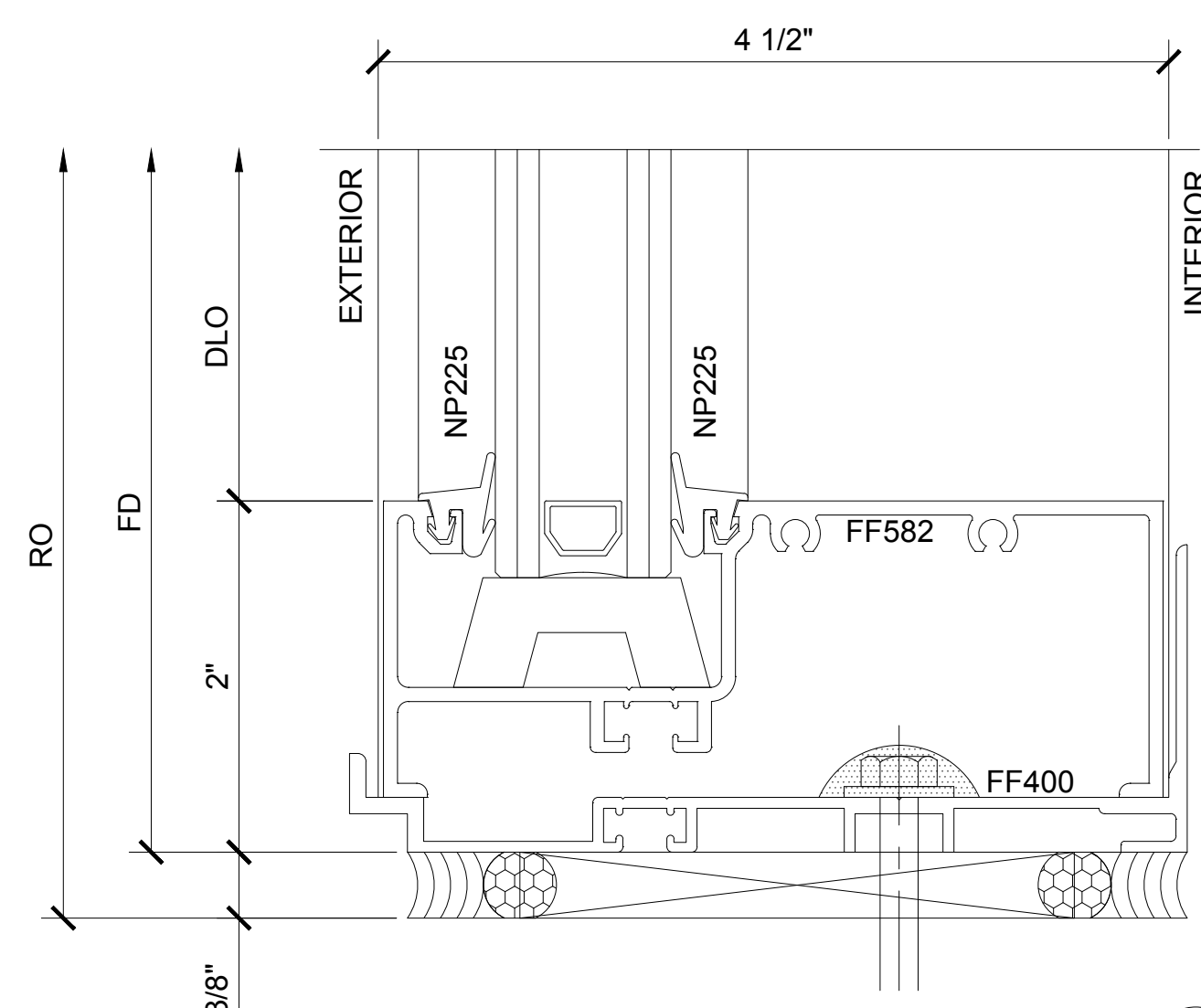
SECTION DETAIL AT SILL
