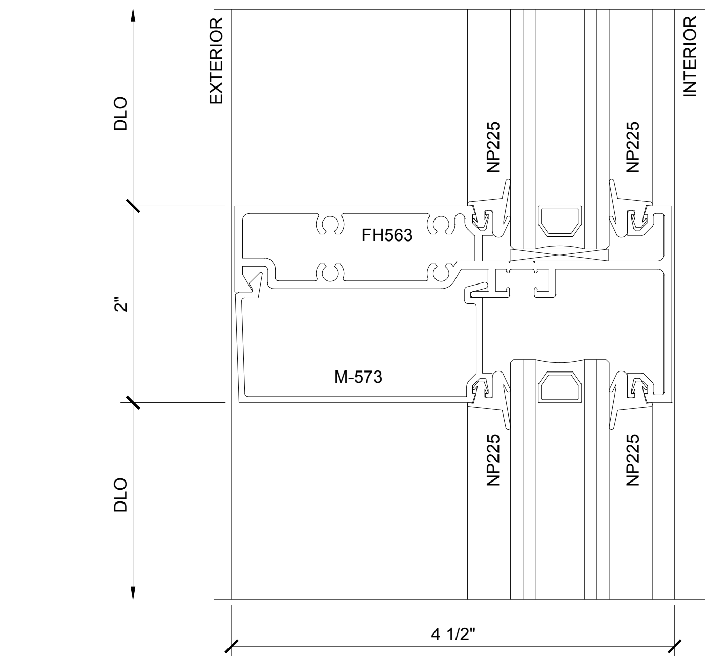
SECTION DETAIL AT INTERMEDIATE HORIZONTAL 2
