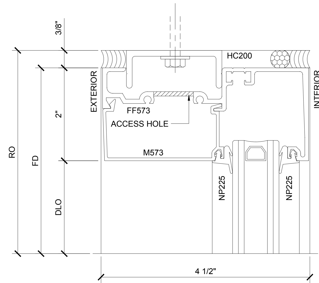
SECTION DETAIL AT HEAD W/ HEAD ANCHOR
