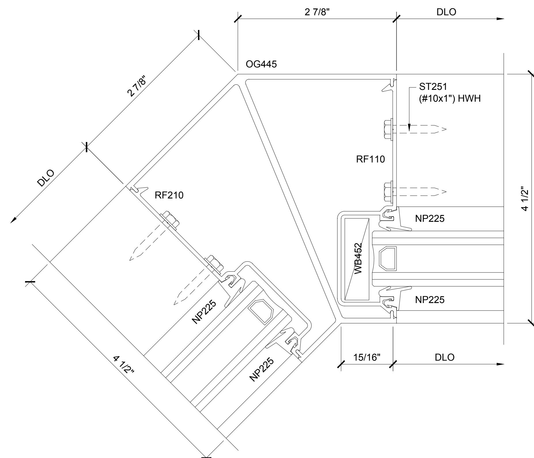
SECTION DETAIL @ JAMB - 135° ①
