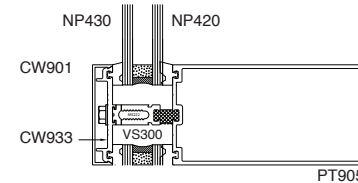
② SILL
