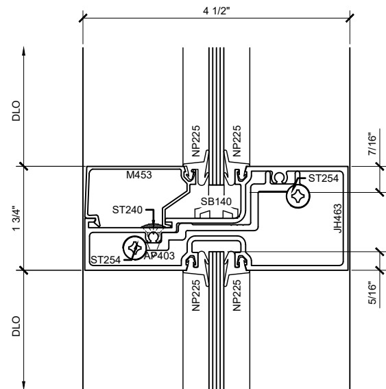
SECTION DETAIL AT INTERMEDIATE HORIZONTAL ③ TYPICAL FOR SCREW RACE ASSEMBLY - (SHEAR BLOCK FOR LOAD DISTRIBUTION)
