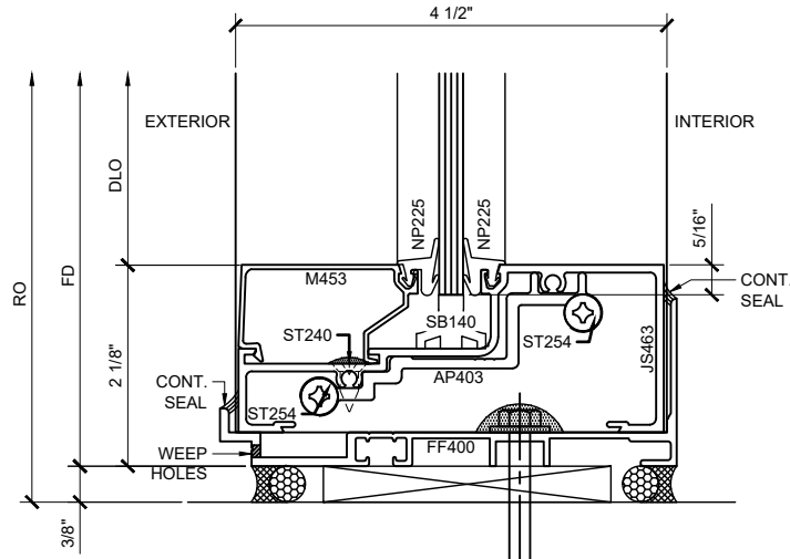
SECTION DETAIL AT INTERMEDIATE HORIZONTAL ② TYPICAL FOR SHEAR LUG ASSEMBLY
