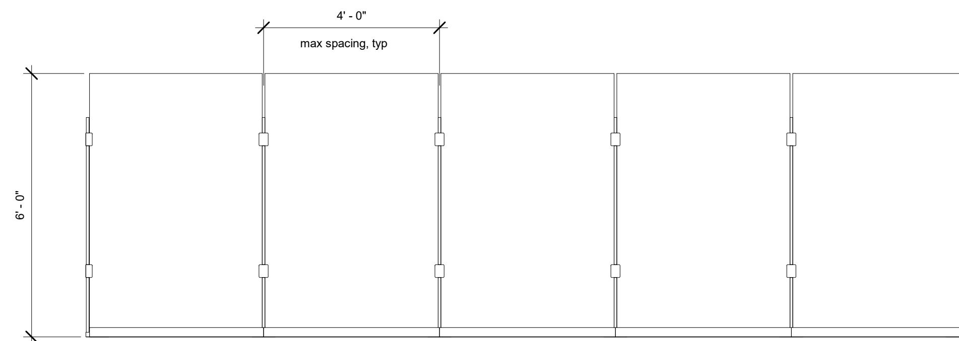
③ KPOSTBS (60" Tall) 1/2" = 1'-0"
