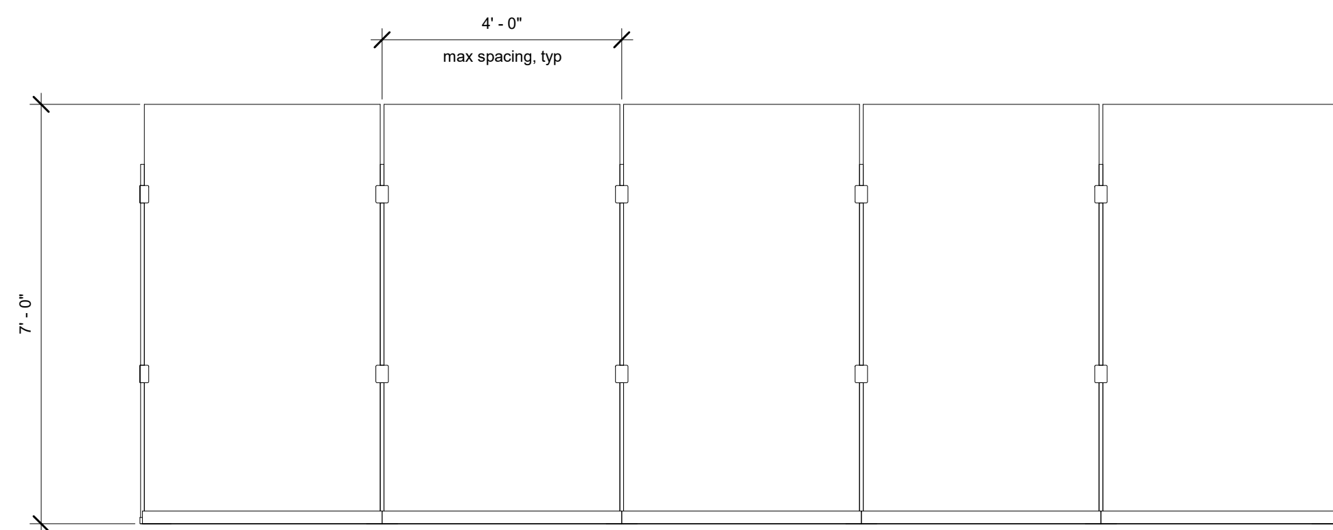
② KPOSTBS (72" Tall) 1/2" = 1'-0"
