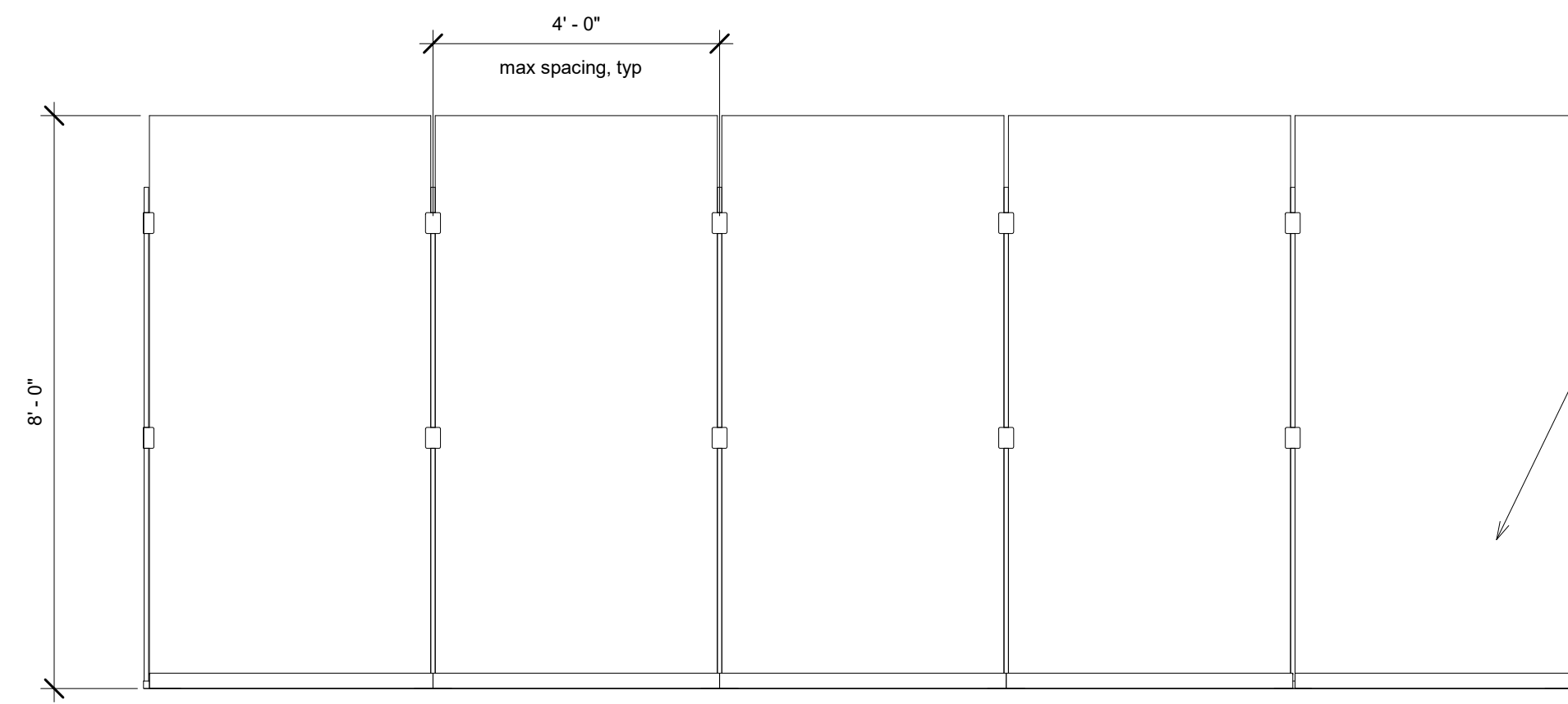
① KPOSTBS (84" Tall) 1/2" = 1'-0"
