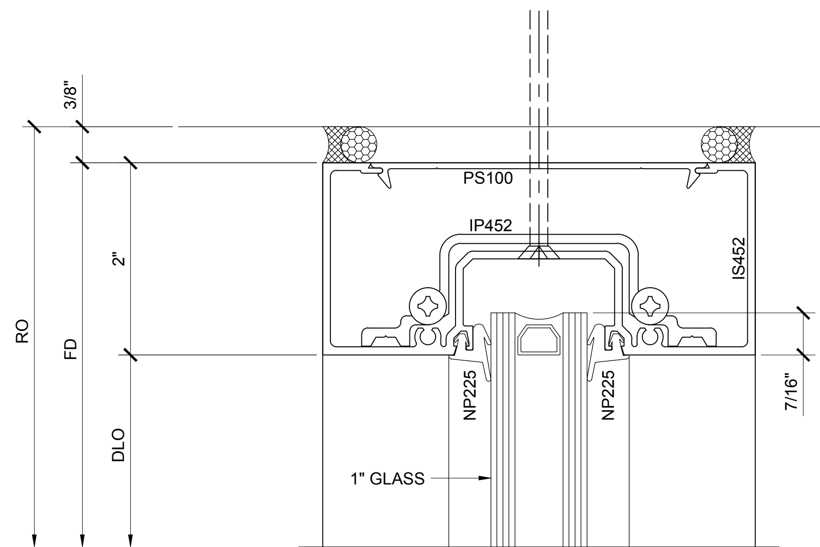
SECTION DETAIL @ STOREFRONT HEAD
