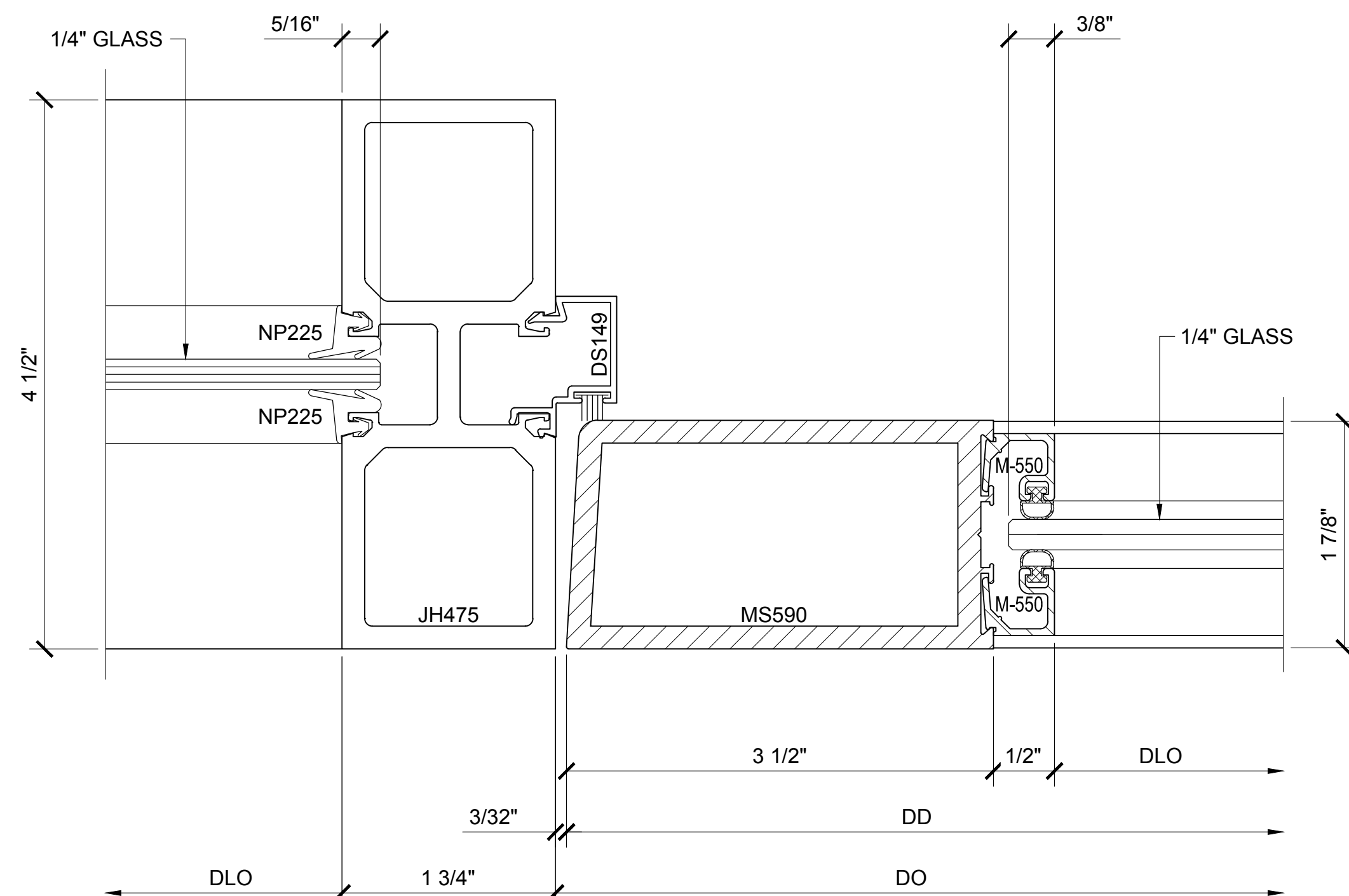
SECTION DETAIL @ DOOR JAMB
