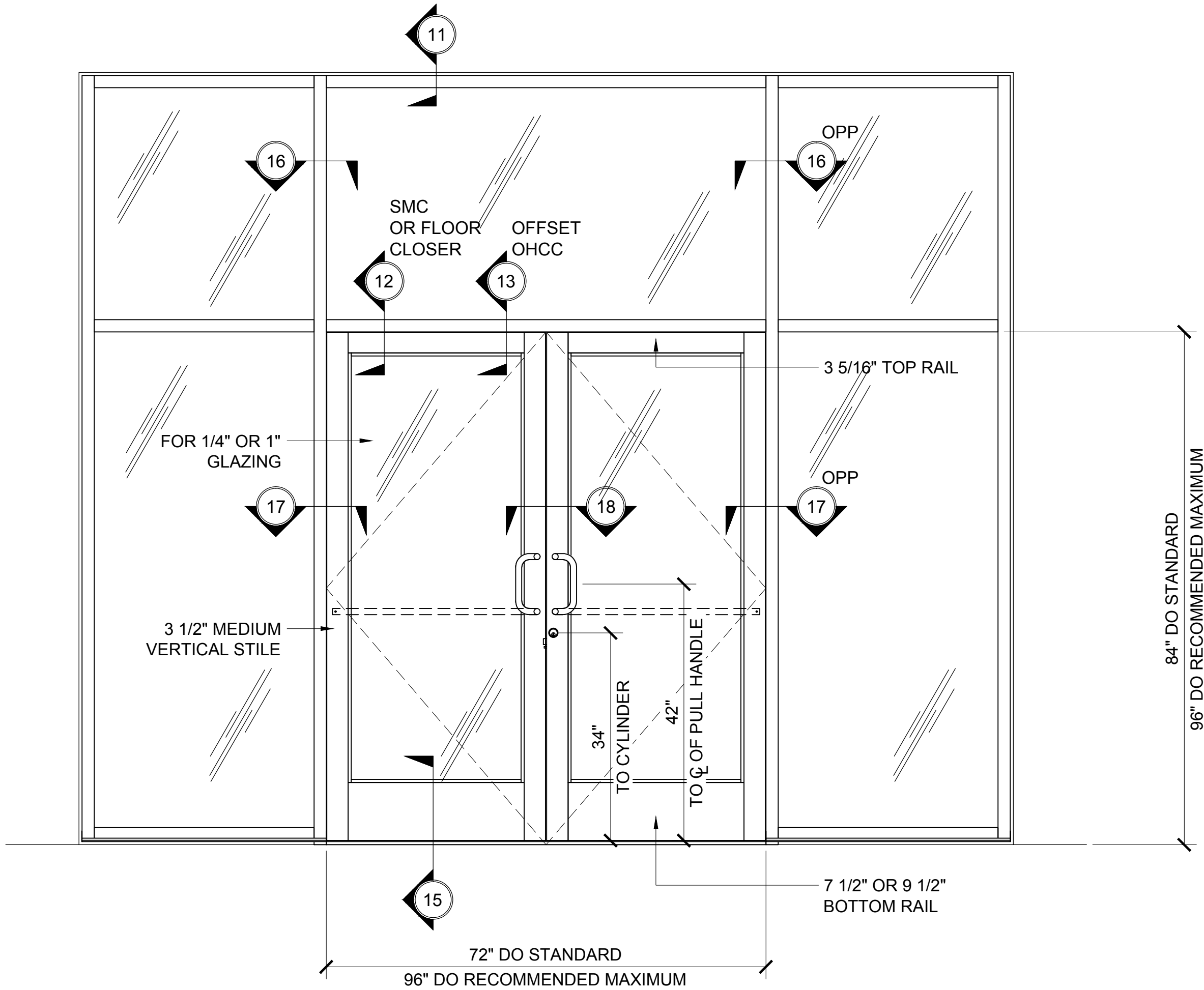
OFFSET-HUNG MEDIUM STILE SERIES 800 DOOR ADA COMPLIANT ELEVATION
