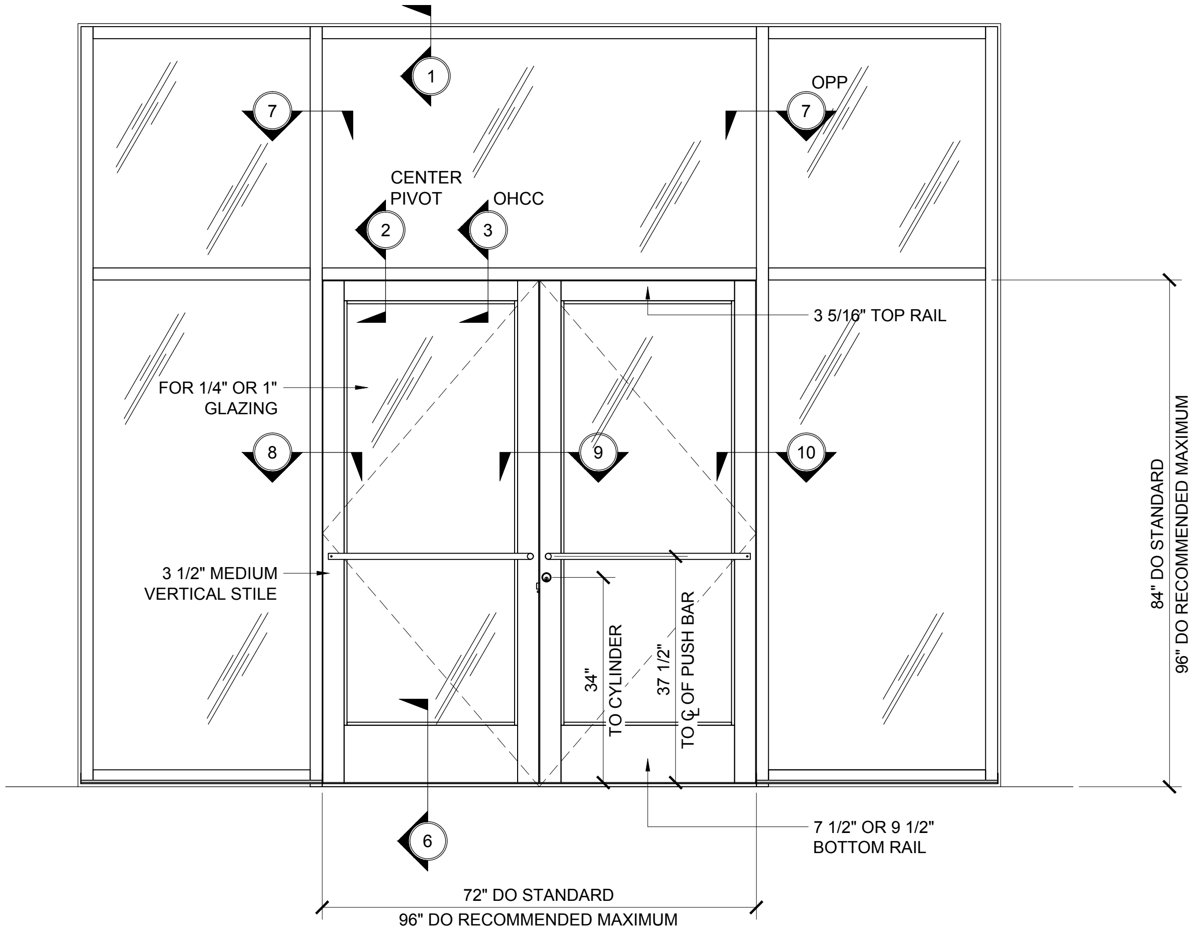
CENTER-HUNG MEDIUM STILE SERIES 800 DOOR ADA COMPLIANT ELEVATION
