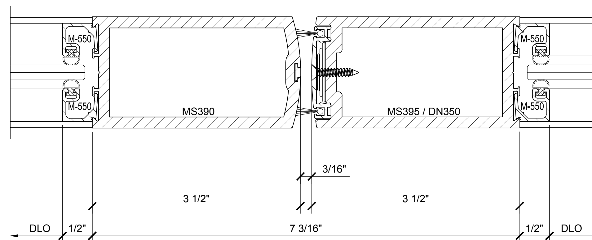
SECTION DETAIL @ MEETING STILES
