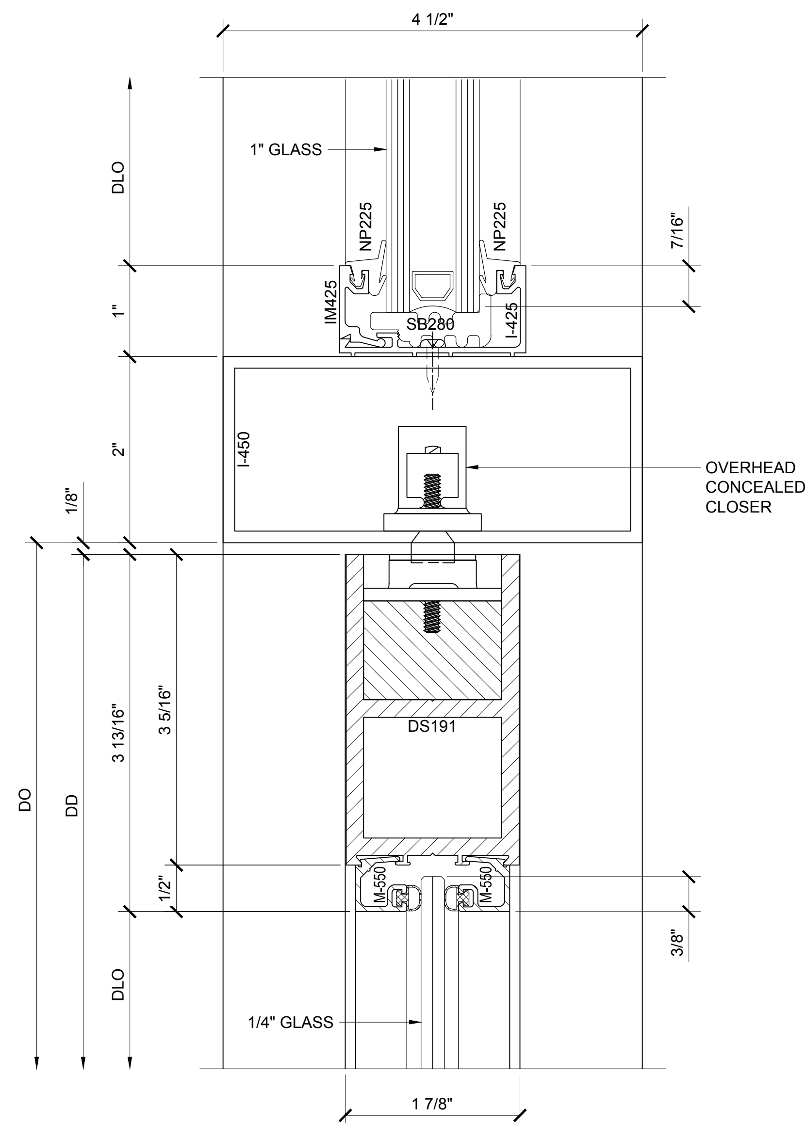
SECTION DETAIL @ DOOR HEAD WITH PIVOT
