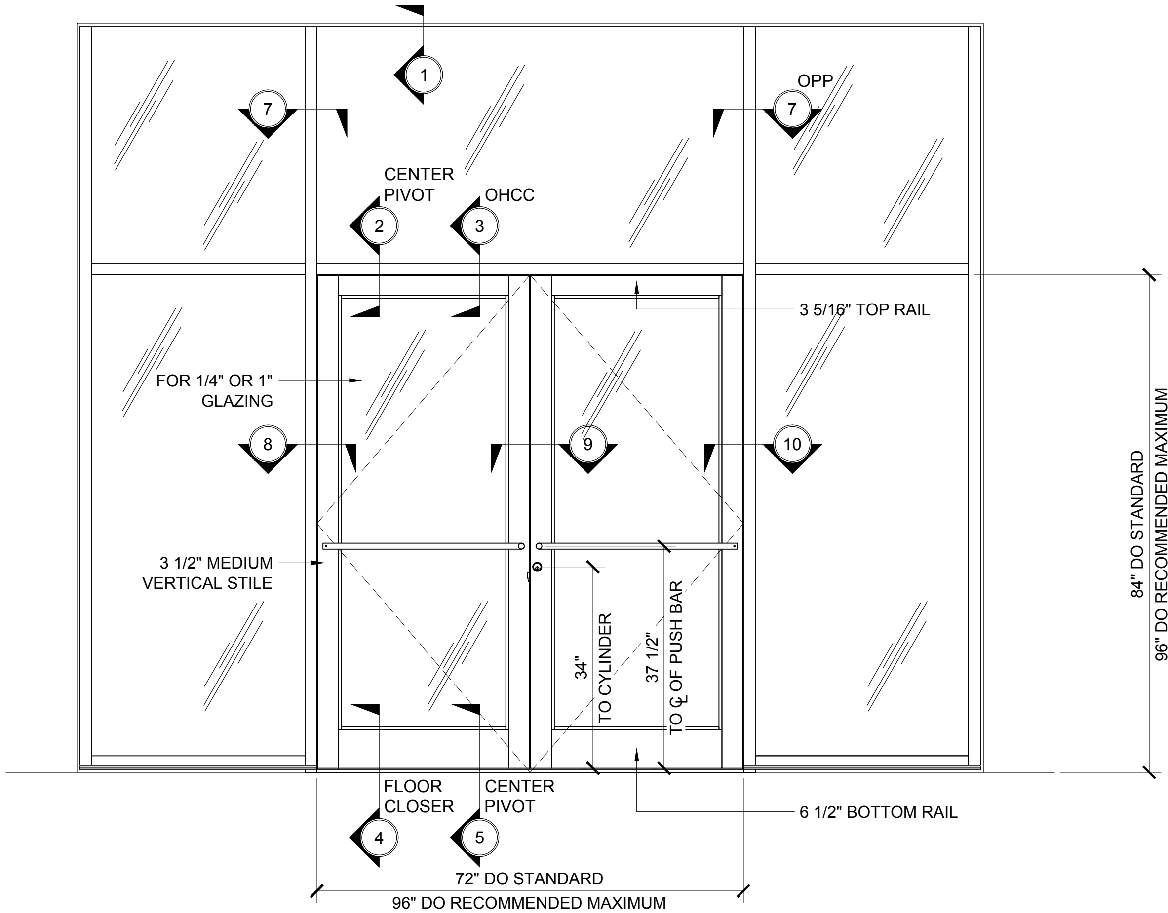
CENTER-HUNG MEDIUM STILE SERIES 800 DOOR TYPICAL ELEVATION
