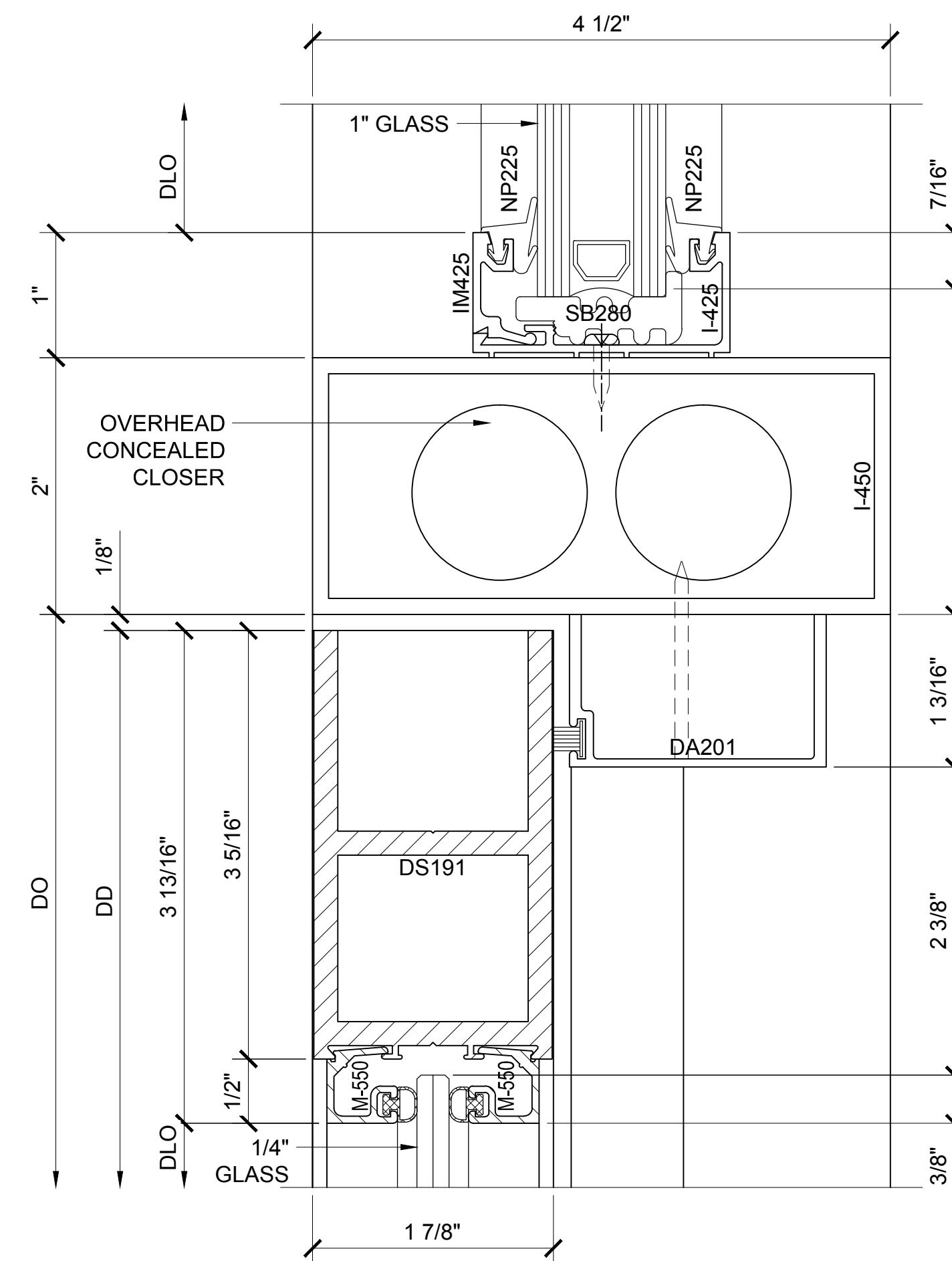
SECTION DETAIL @ DOOR HEAD WITH OHCC (13)
