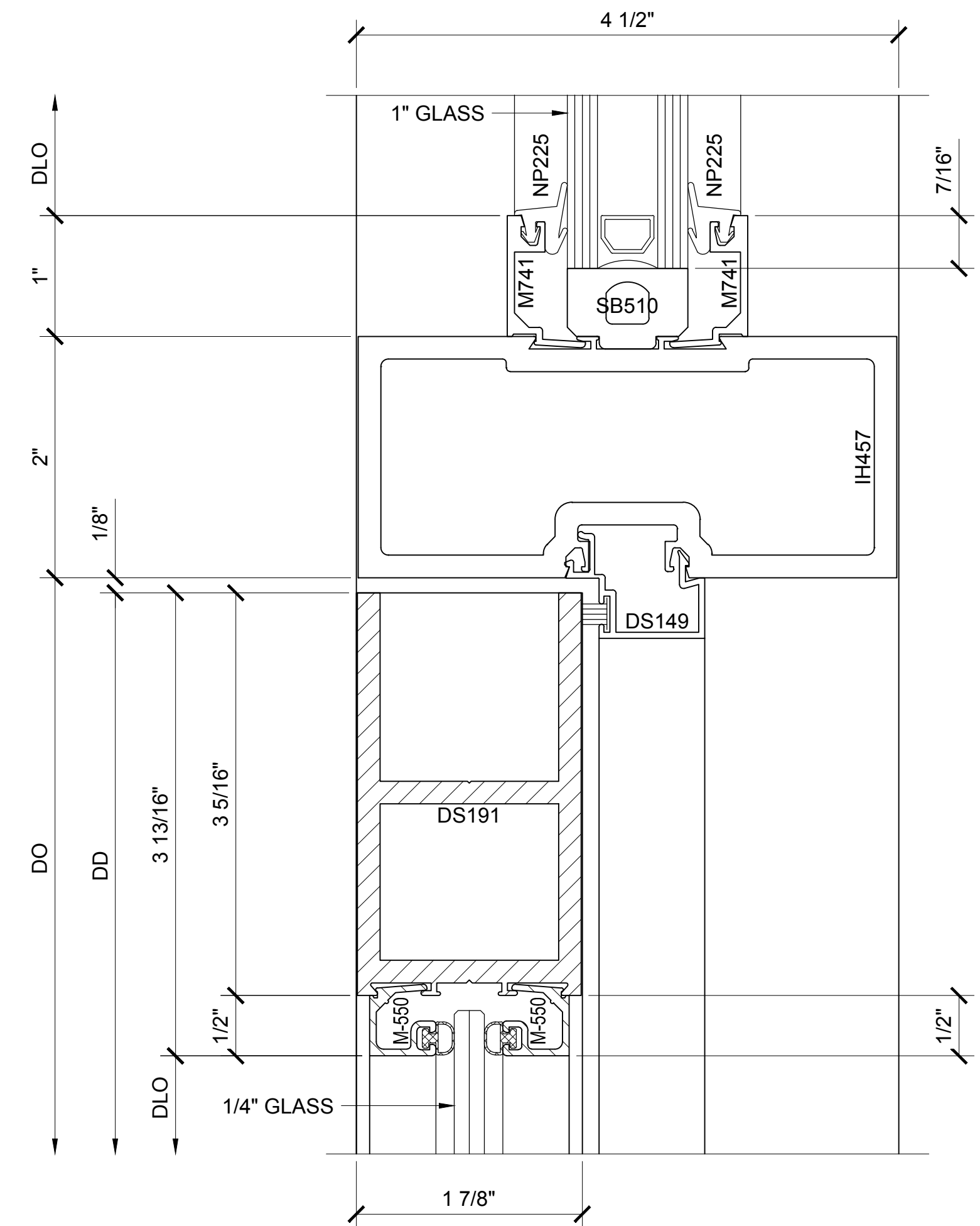
SECTION DETAIL @ DOOR HEAD WITH PIVOT (12)
