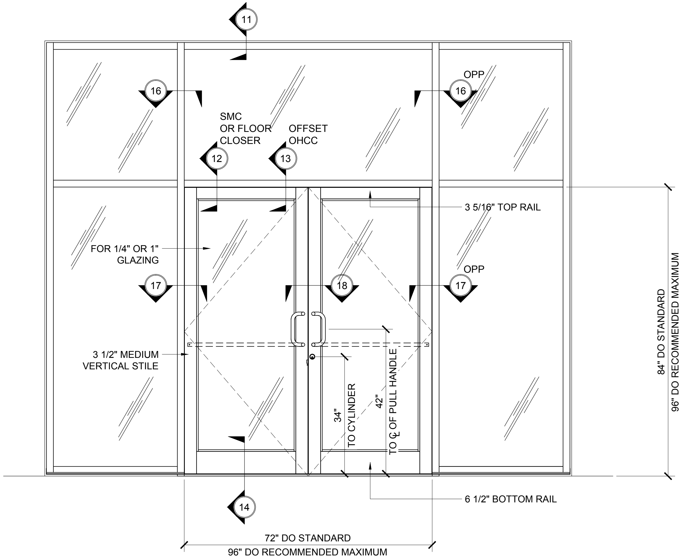
OFFSET-HUNG MEDIUM STILE SERIES 800 DOOR TYPICAL ELEVATION
