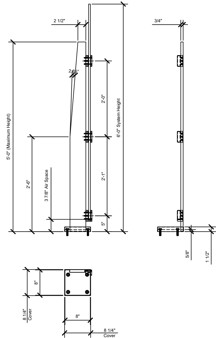
3 MET60REBS - 3/4" TH. BRUSHED SS CENTER POST (60" TALL)
