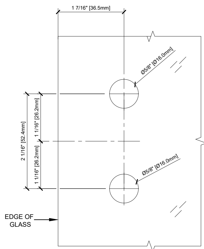
FIXED PANEL TEMPLATE
