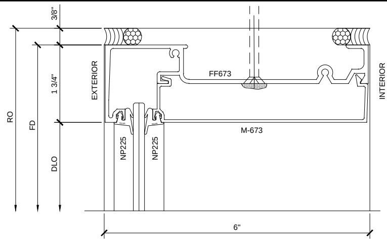
SECTION DETAIL AT HEAD 8
