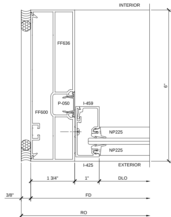
SECTION DETAIL AT JAMB ①
