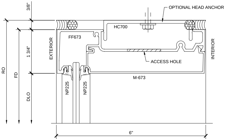
SECTION DETAIL AT HEAD W/ ANCHOR ①
