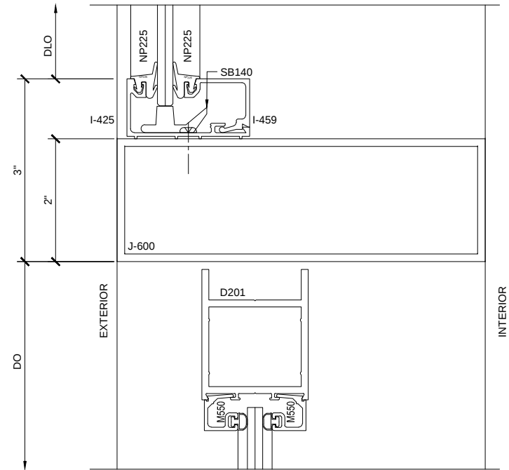
SECTION DETAIL AT DOOR HEADER 9
