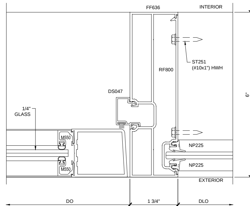
SECTION DETAIL AT INTERMEDIATE VERTICAL
