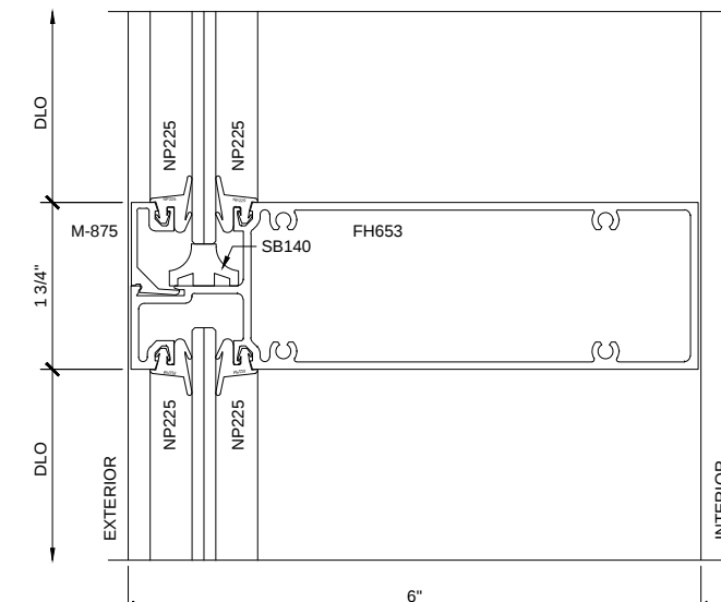
SECTION DETAIL AT INTERMEDIATE HORIZONTAL EXTERIOR GLAZING
