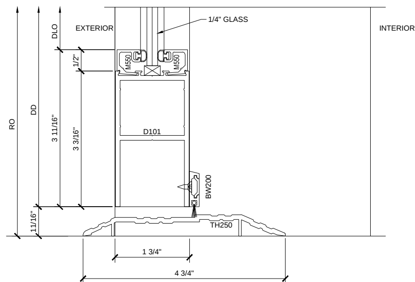
SECTION DETAIL @ BOTTOM RAIL 11
