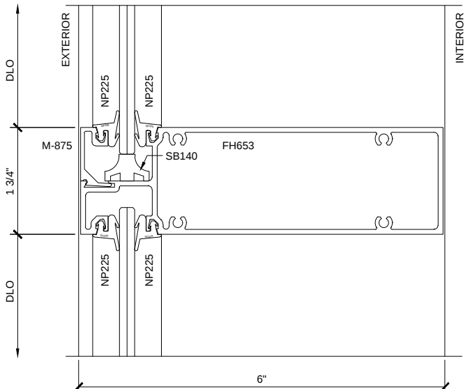
SECTION DETAIL AT INTERMEDIATE HORIZONTAL ⑥
