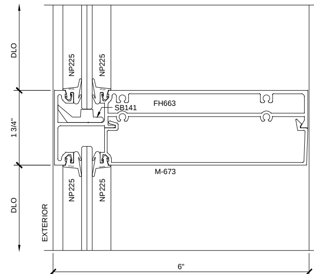
SECTION DETAIL AT INTERMEDIATE HORIZONTAL INTERIOR GLAZING
