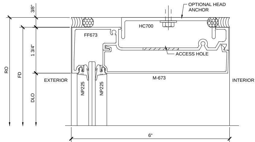
SECTION DETAIL AT HEAD 7
