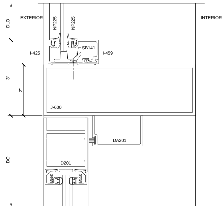
SECTION DETAIL @ DOOR HEADER 10
