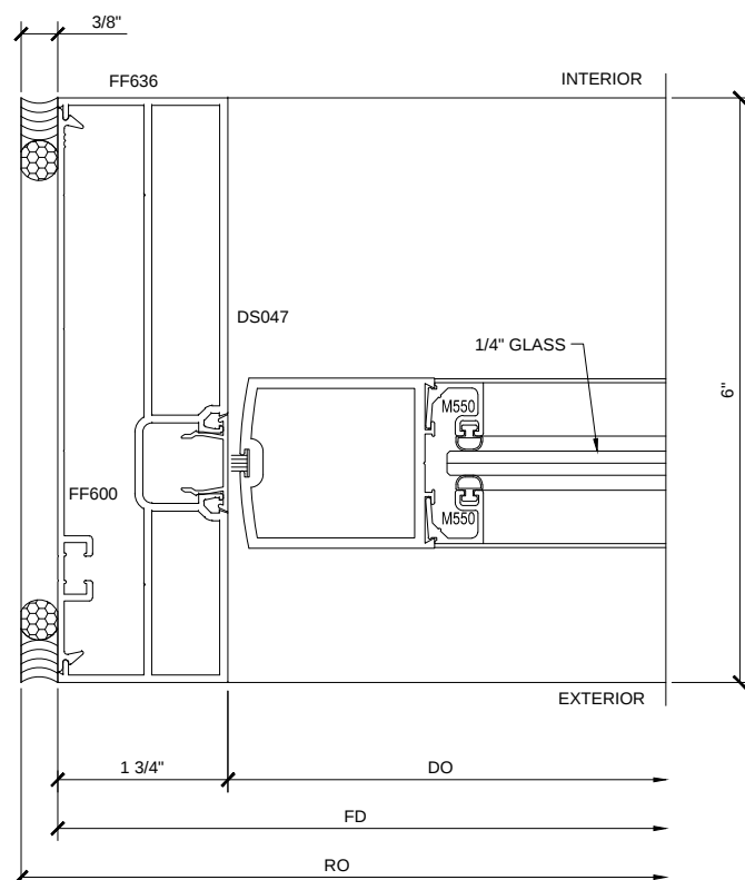
SECTION DETAIL AT DOOR JAMB ②
