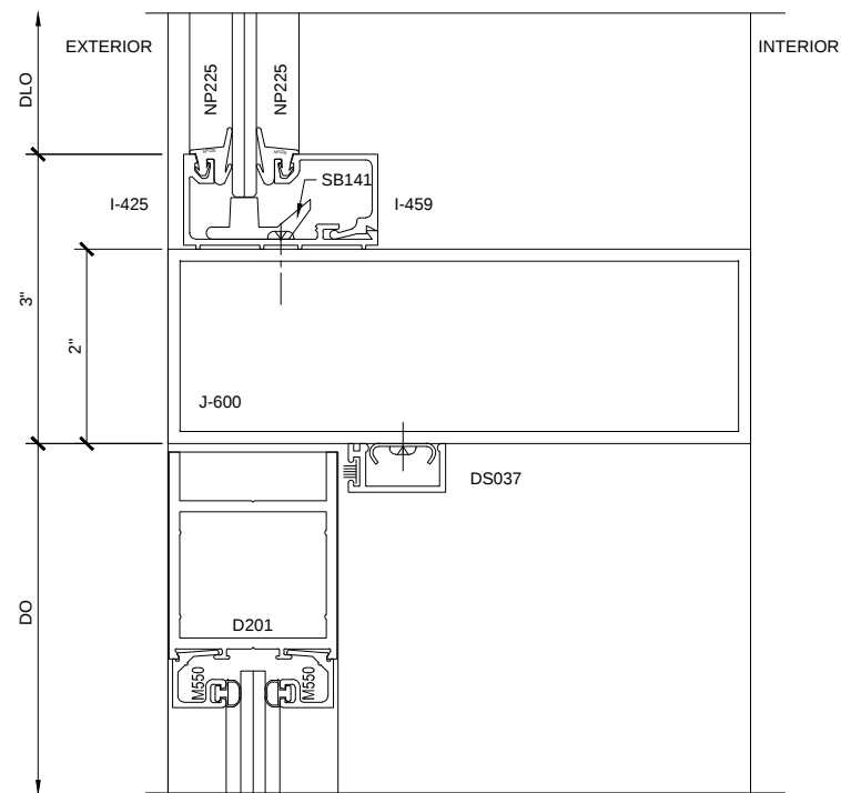
SECTION DETAIL @ DOOR HEADER 8
