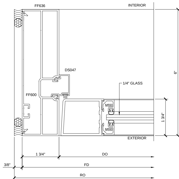
SECTION DETAIL AT DOOR JAMB
