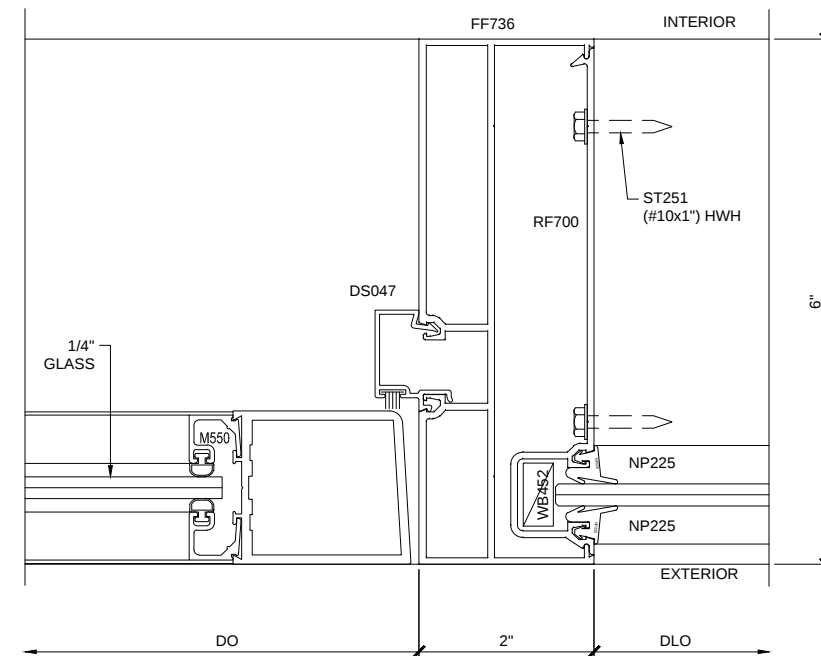
SECTION DETAIL AT INTERMEDIATE VERTICAL (2")
