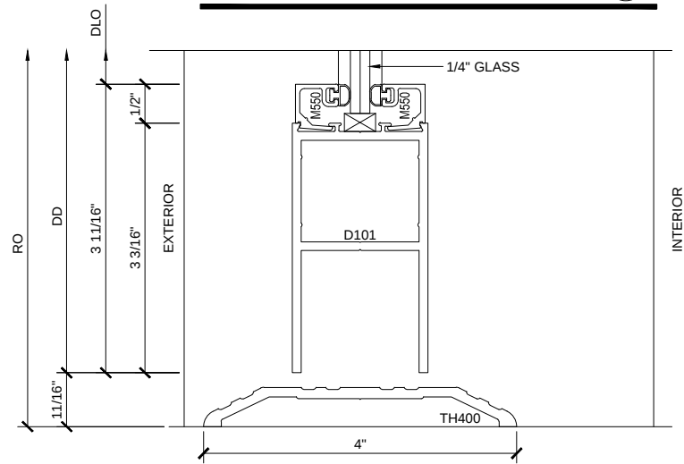
SECTION DETAIL AT BOTTOM RAIL 10
