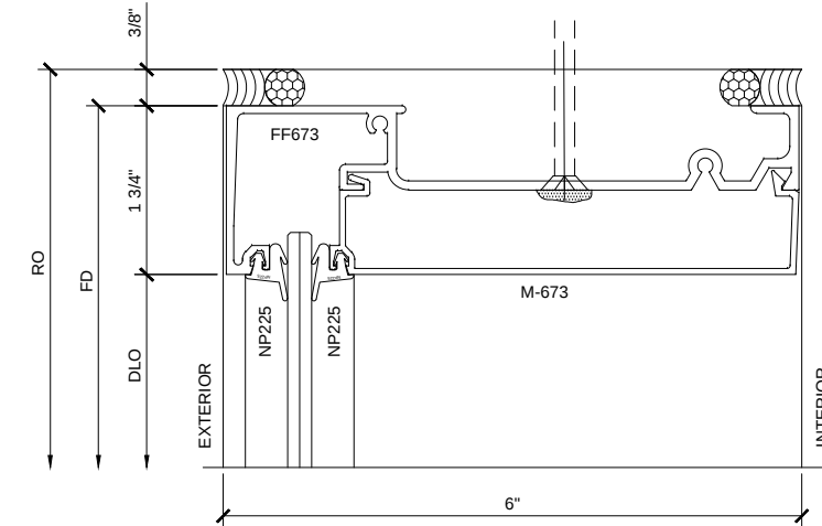
SECTION DETAIL AT HEAD EXTERIOR GLAZING
