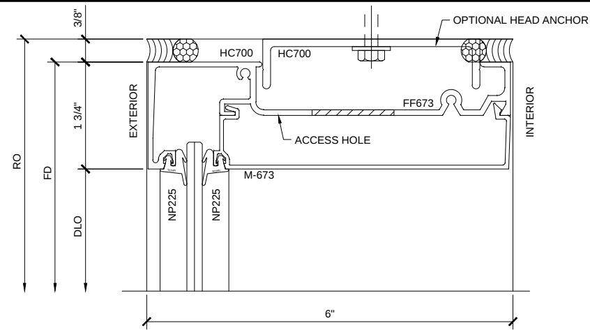
SECTION DETAIL AT HEAD INTERIOR GLAZING 7
