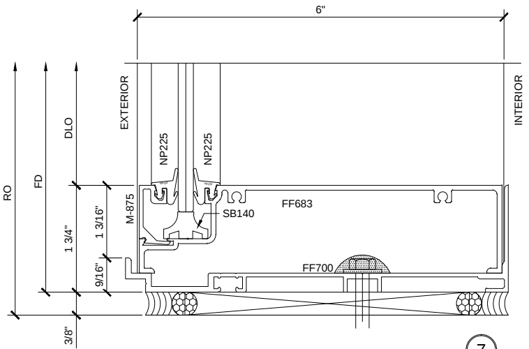
SECTION DETAIL AT SILL ⑦
