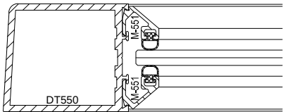
1/4" GLASS - TAPERED
