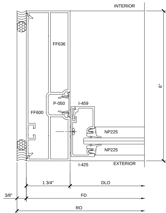
SECTION DETAIL @ JAMB
