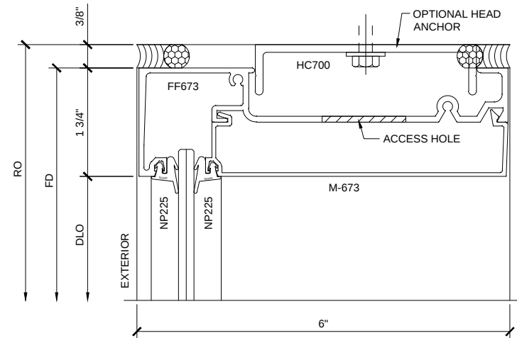
SECTION DETAIL AT HEAD INTERIOR GLAZING
