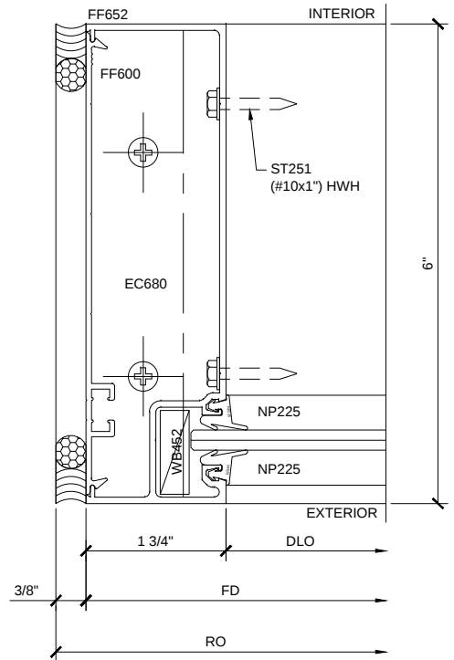
SECTION DETAIL AT JAMB
