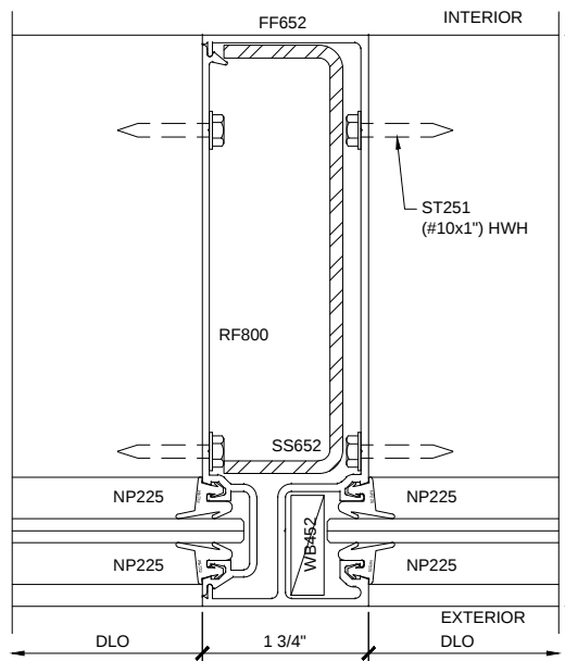
SECTION DETAIL AT INTERMEDIATE VERTICAL
