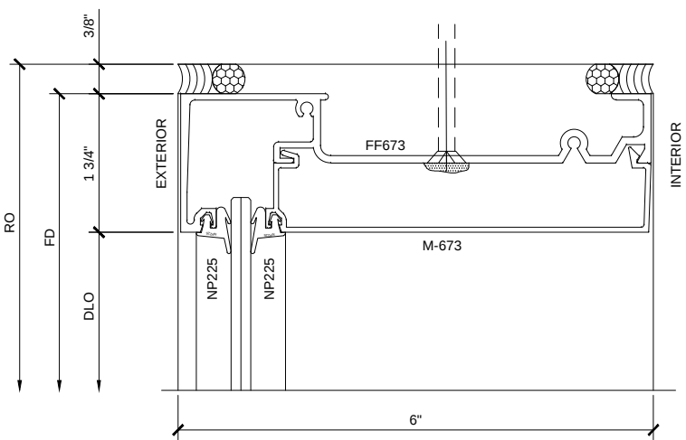
SECTION DETAIL AT HEAD ⑤
