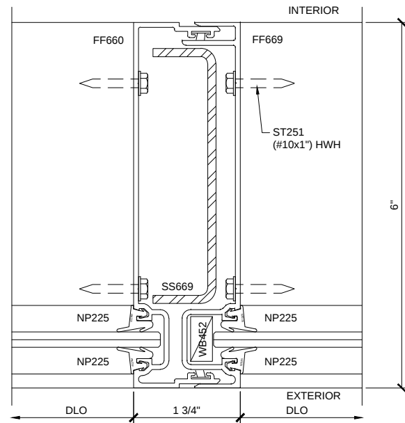
SECTION DETAIL EXPANSION INTERMEDIATE VERTICAL
