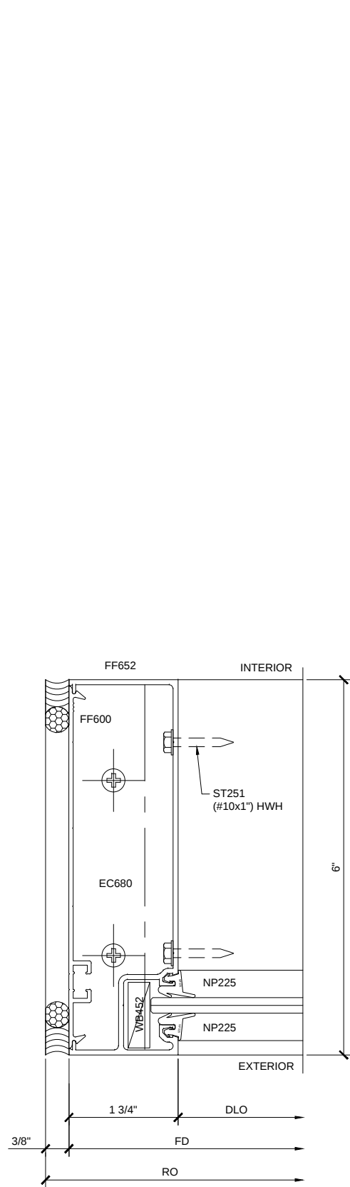
SECTION DETAIL AT JAMB ②
