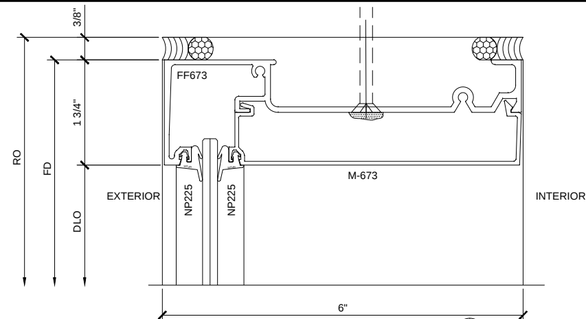
SECTION DETAIL AT HEAD 9
