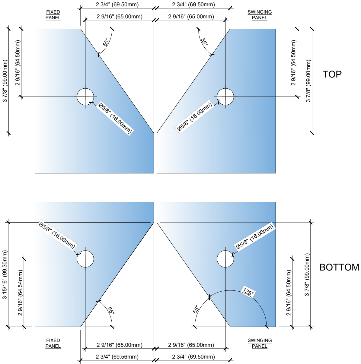
3B GLASS CUT OUT DETAIL - 4MM FIXED PANEL GAP ARCH REF: SCALE: 1'-0"=1'-0"
