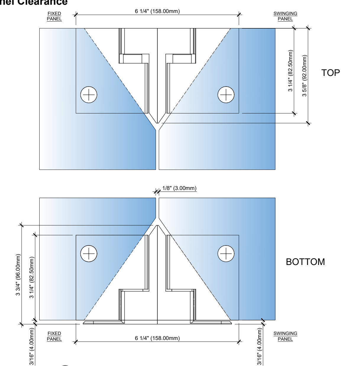
2B FRONT VIEW DETAIL - 4MM FIXED PANEL GAP ARCH REF: SCALE: 1'-0"=1'-0"
