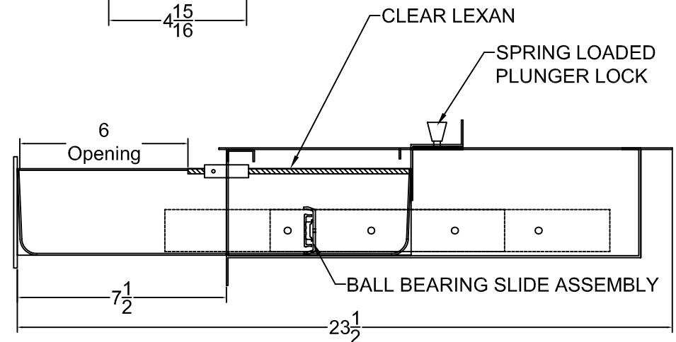
Fully Opened Position
