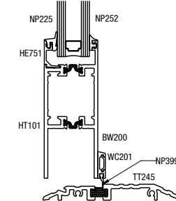
2 BOTTOM RAIL
