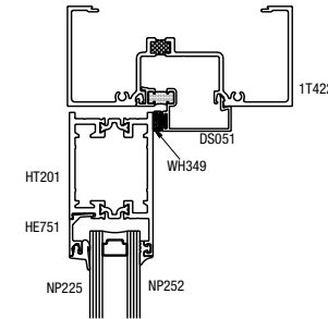
1 TOP RAIL
