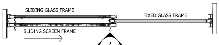
1 PLAN VIEW REF: Scale: NTS.
