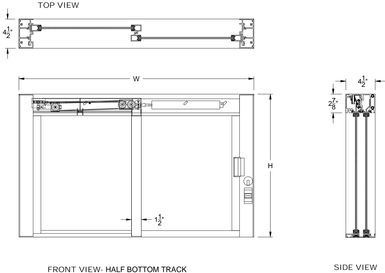
FRONT VIEW- HALF BOTTOM TRACK
