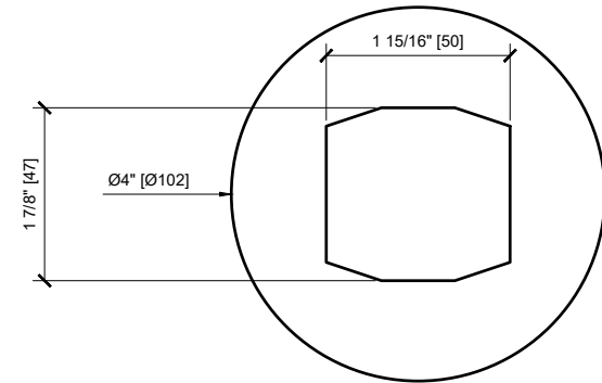
⑤ AFWC1G / AFWC6G (OPTIONAL GARNISH RING) 1'-0"=1'-0"
