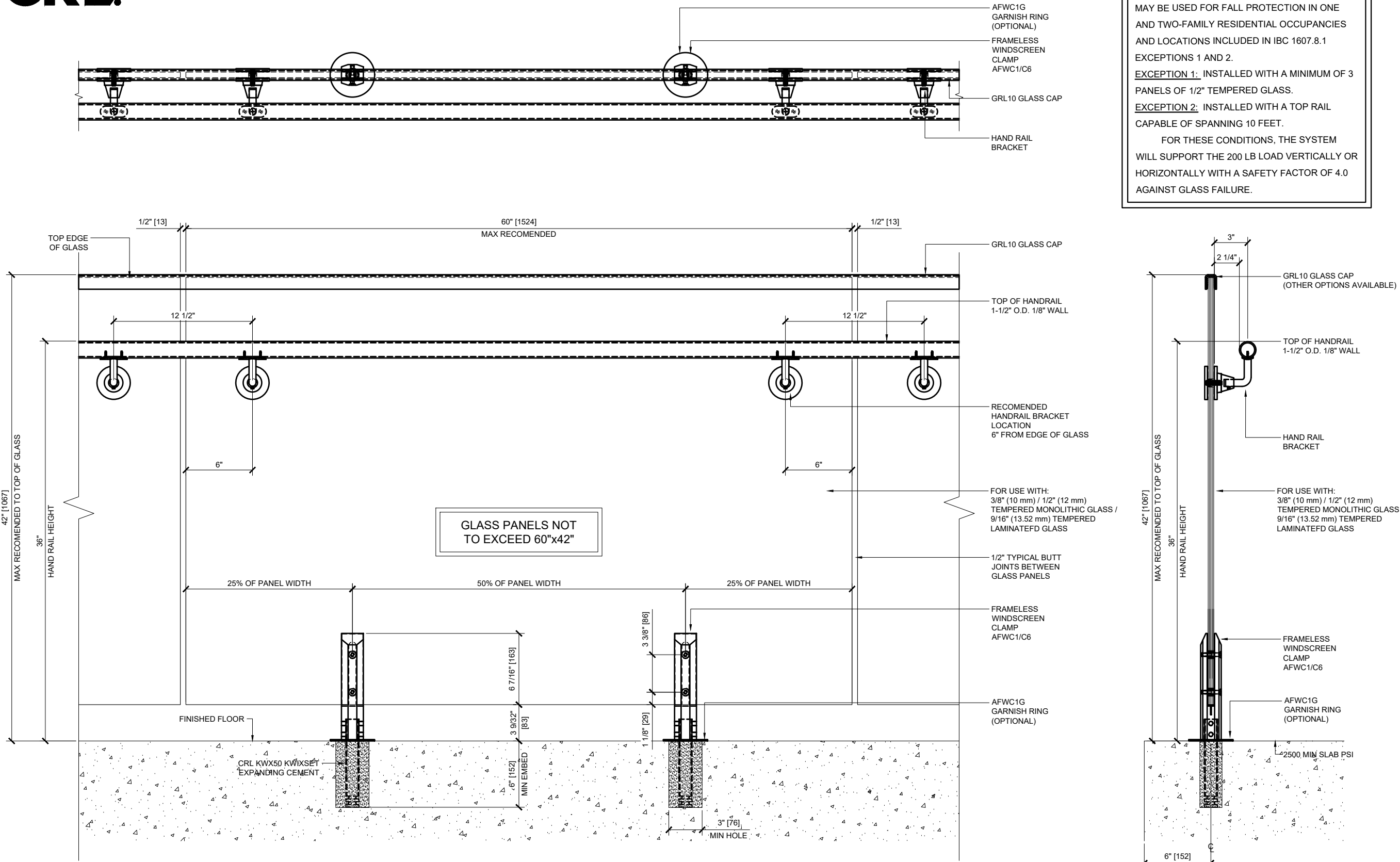
① GUARDRAIL INTERIOR ELEVATION
