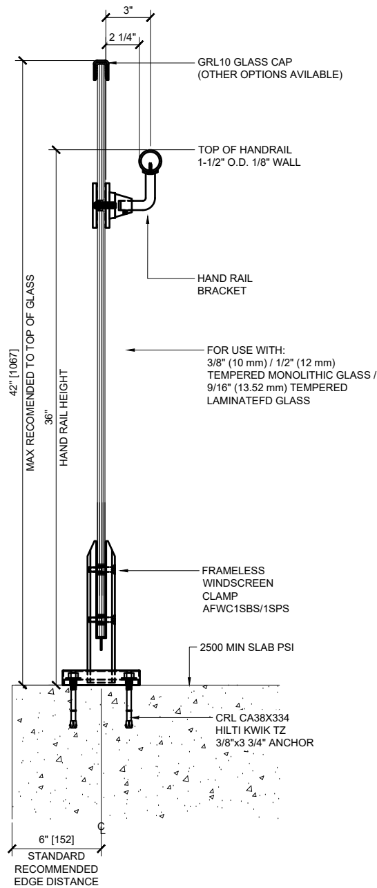
② GUARD RAIL SECTION
