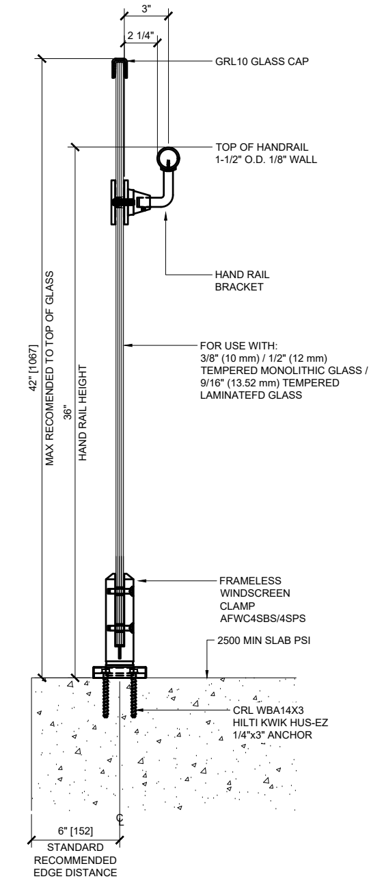
② GUARD RAIL SECTION
