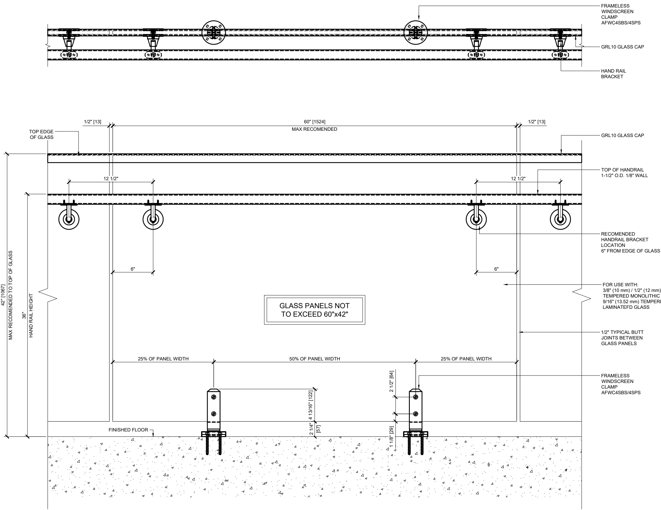
① GUARDRAIL INTERIOR ELEVATION
