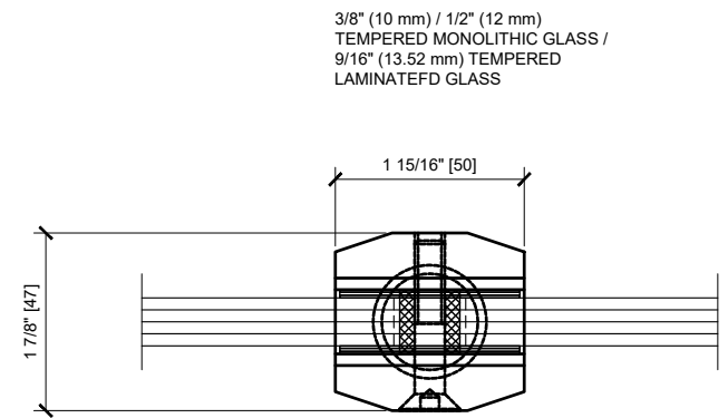
⑤ GLASS FABRICATION REQUIREMENTS 1'-0"=1'-0"
