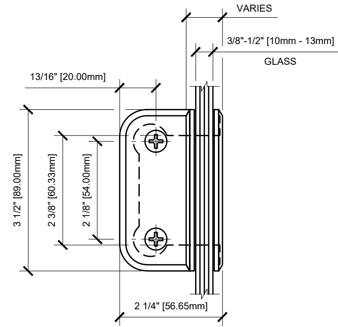
ESTA090XX - CRL ESTATE 090 SERIES 90 DEGREE GLASS TO GLASS HINGE
