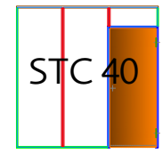
SETUP B - STC 40 Wooden sound-proof door incl. drop-down seal with glass side panels and transom
