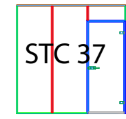
SETUP A - STC 37 Glass door incl. drop-down seal with glass side panels and transom
