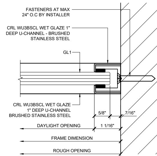
④ WALL JAMB DETAIL ARCH REF: 1'-0"=1'-0"
