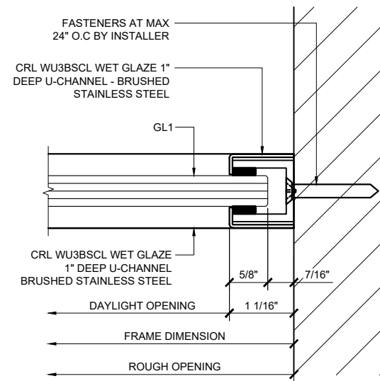
③ WALL JAMB DETAIL ARCH REF: 1'-0"=1'-0"
