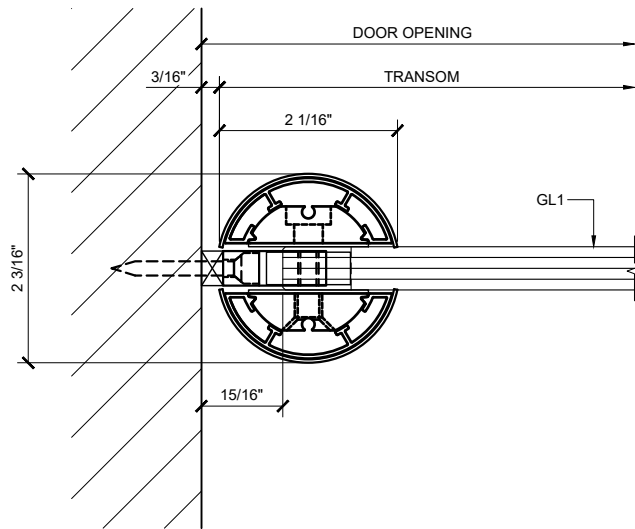
⑤ TRANSOM POST SECTION AT WALL DETAIL ARCH REF: 1'-0"=1'-0"
