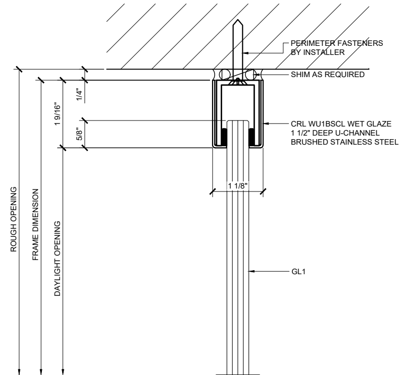
④ SIDELITE HEAD DETAIL
