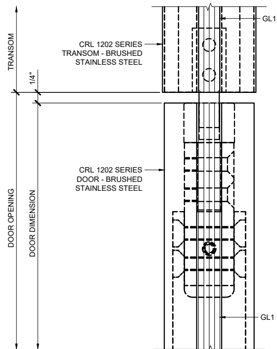
② DOOR HEAD AT TRANSOM DETAIL
