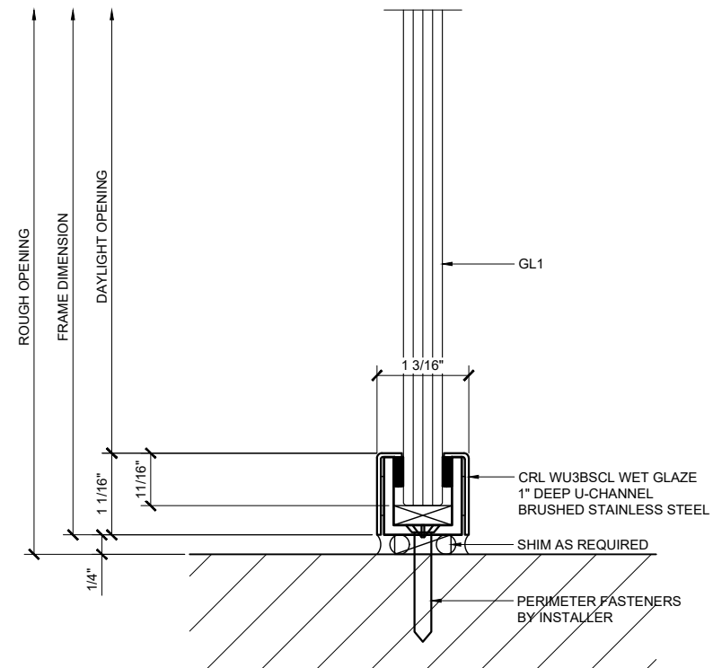
⑤ SIDELITE SILL DETAIL
