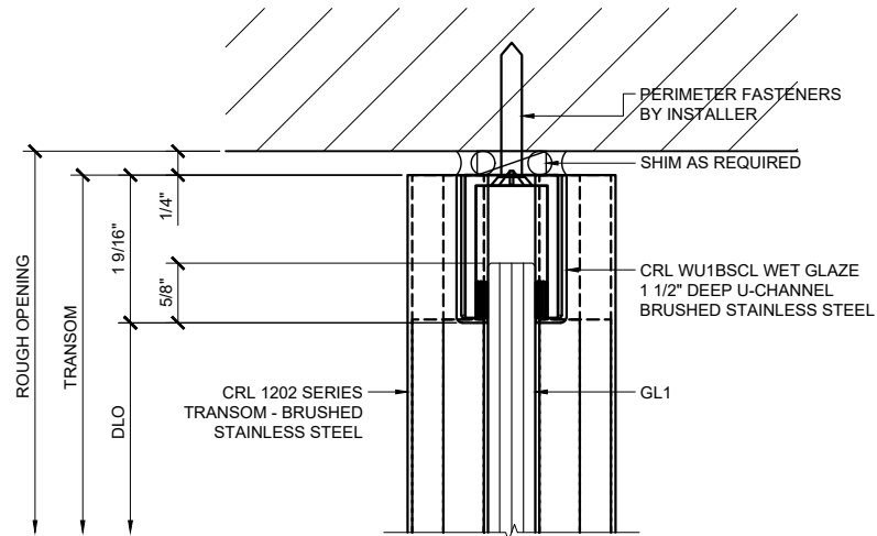
① TRANSOM HEAD DETAIL
