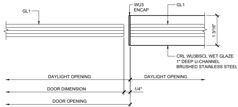
② DOOR JAMB AT SIDELITE ARCH REF: 1'-0"=1'-0"
