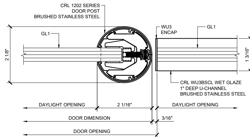
③ DOOR PIVOT POST SECTION DETAIL ARCH REF: 1'-0"=1'-0"
