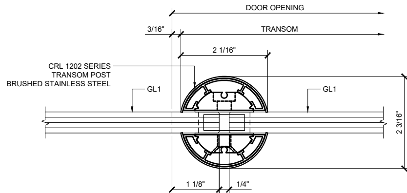
⑤ TRANSOM POST SECTION DETAIL
