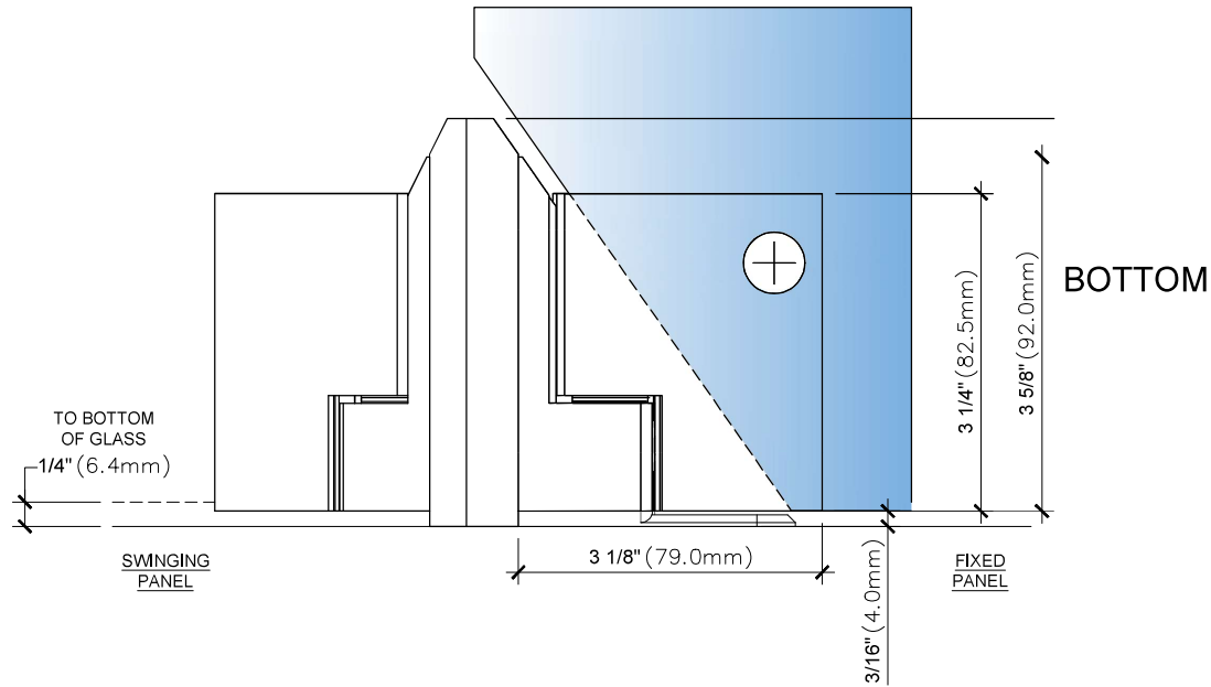
2B FRONT VIEW DETAIL @4MM FIXED PANEL GAP ARCH REF: (SWINGING PANEL GLASS NOT SHOWN) SCALE: 1'-0"=1'-0"
