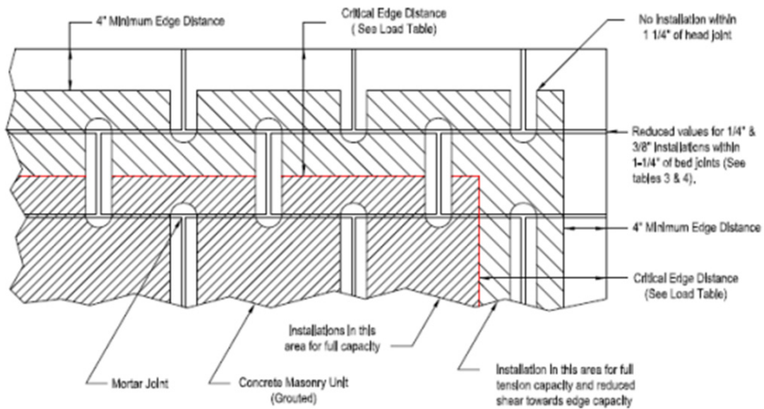
FIGURE 2—ACCEPTABLE LOCATIONS (SHADED AREAS) FOR HILTI KWIK HUS-EZ ANCHORS IN GROUT-FILLED CONCRETE MASONRY
