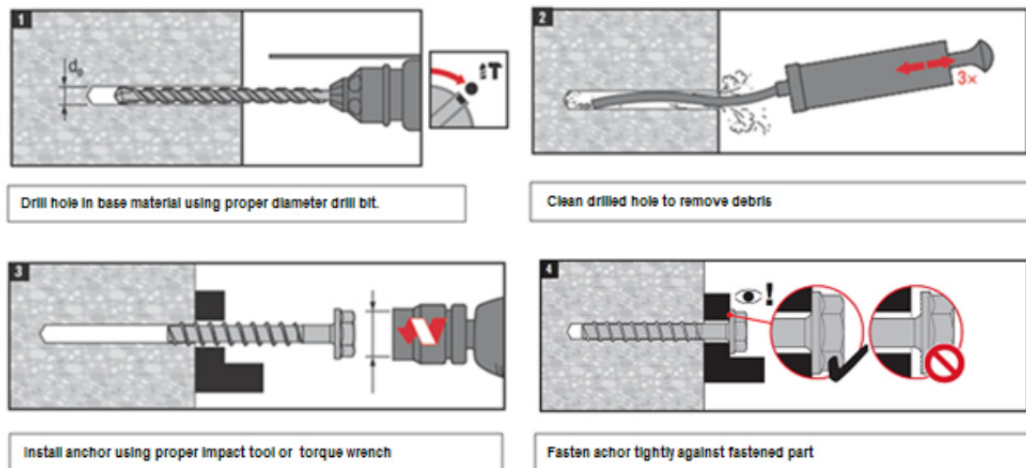
FIGURE 4—INSTALLATION INSTRUCTIONS – HILTI KWIK HUS-EZ (KH-EZ)
