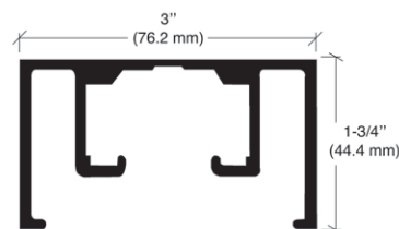
D1670 OVERHEAD TRACK When Matching a Store Front Extrusion, D1670 Upper Track may be used. Specify D1019 Assembly
