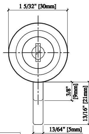
PLUNGER LOCK FOR 3/8" (9.5mm) GLASS DOOR
