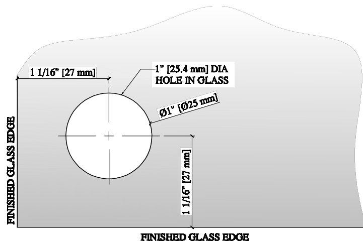
GLASS FABRICATION
