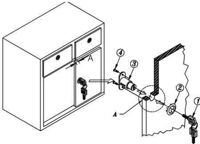
① Keys ② Rosette ③ Cylinder ④ Screws
