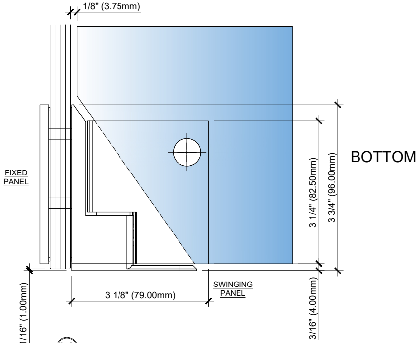
2A FRONT VIEW DETAIL - 1MM FIXED PANEL GAP ARCH REF: SCALE: 1'-0"=1'-0"
