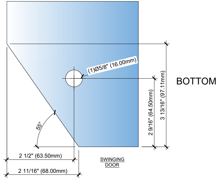
3A GLASS CUT OUT DETAIL - 1MM FIXED PANEL GAP ARCH REF: SCALE: 1'-0"=1'-0"
