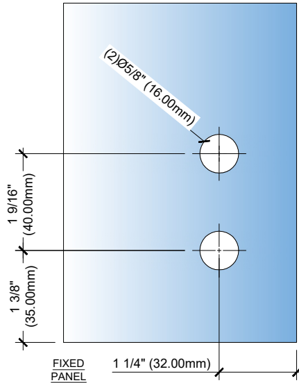
3A GLASS CUT OUT DETAIL - 1MM FIXED PANEL GAP ARCH REF: SCALE: 1'-0"=1'-0"
