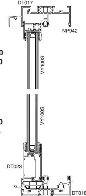
4 FIXED SILL
