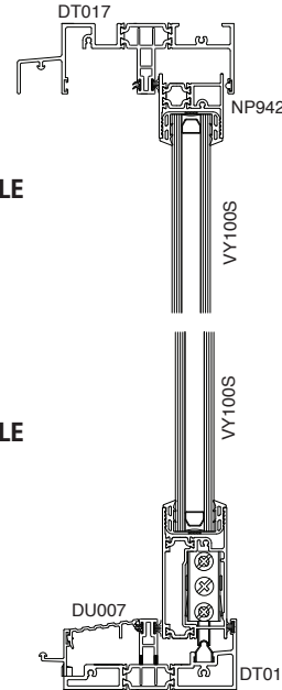
3 FIXED HEAD
