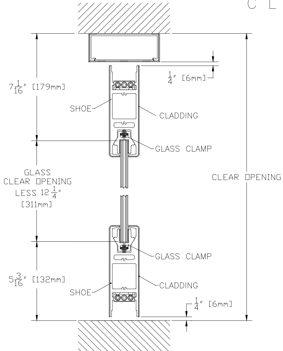
6" SQUARE DOOR RAIL TOP AND BOTTOM CLAD WITH CLAD HEADER
