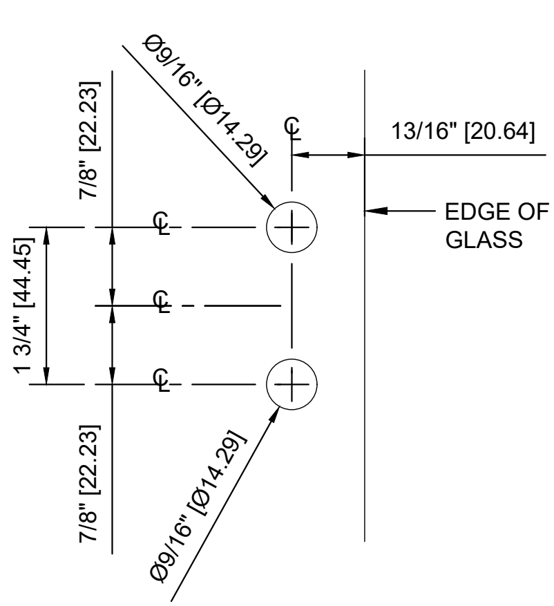
DOOR PANEL "A" GLASS FABRICATION TEMPLATE
