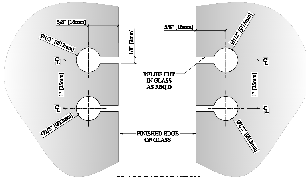
GLASS FABRICATION
