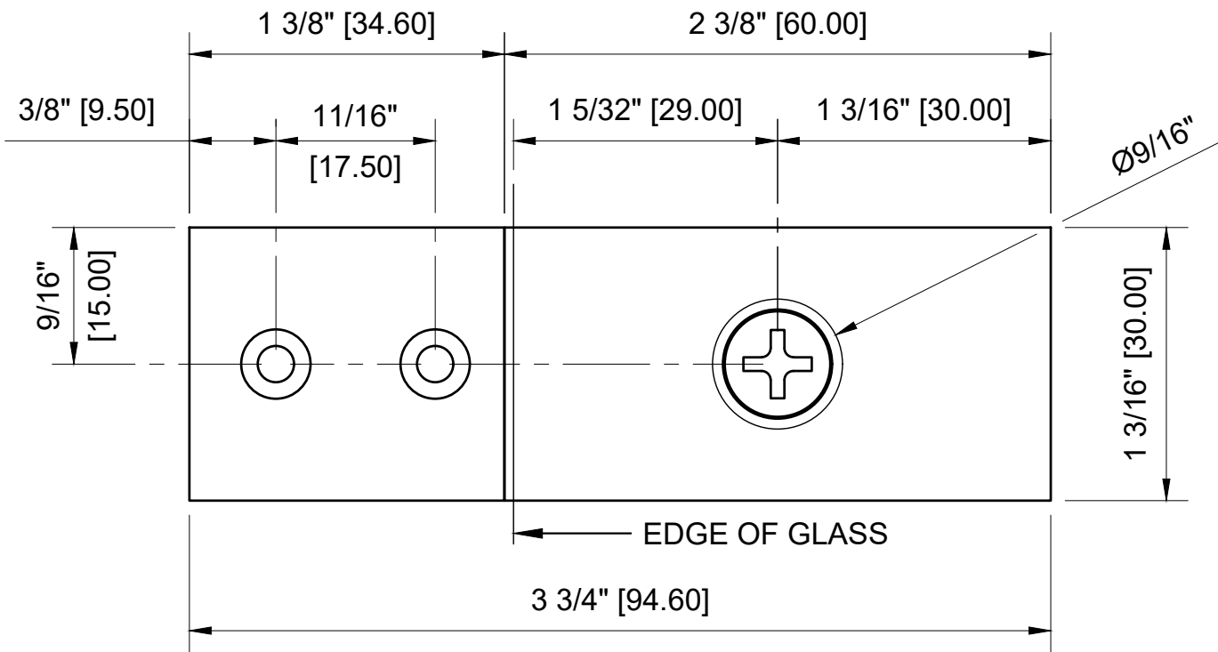
CRL - EH85 BRUSHED NICKEL LIGHT DUTY SQUARE CORNER STYLE HINGE FOR 1/4" - 5/16" GLASS
