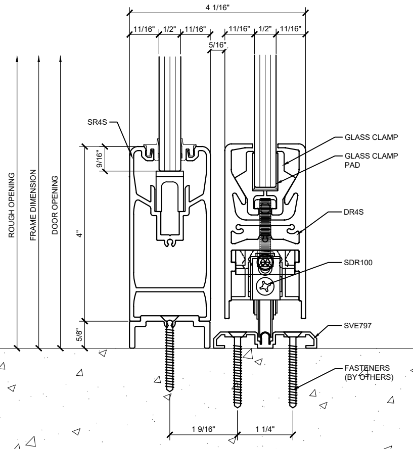
② SECTION DETAIL @ BOTTOM RAIL
