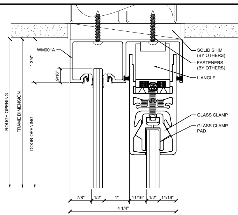
① SECTION DETAIL @ HEAD
