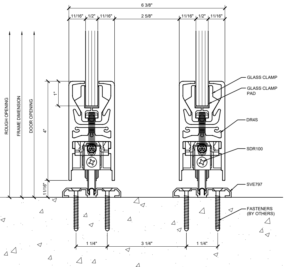
② SECTION DETAIL @ BOTTOM RAIL
