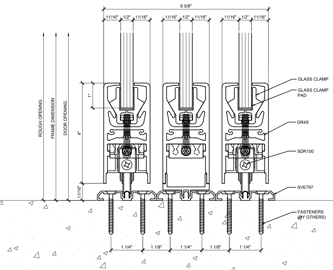
② SECTION DETAIL @ BOTTOM RAIL
