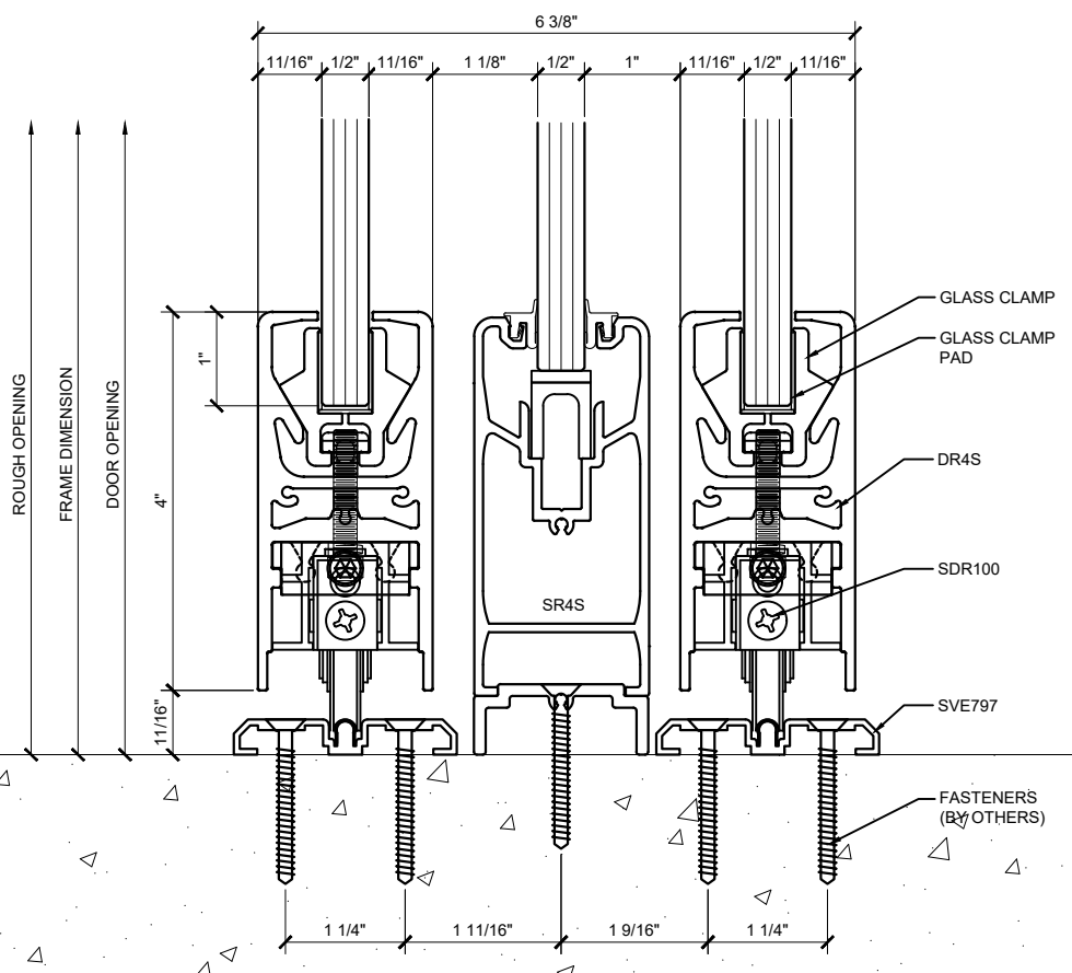
⑥ SECTION DETAIL @ BOTTOM RAIL
