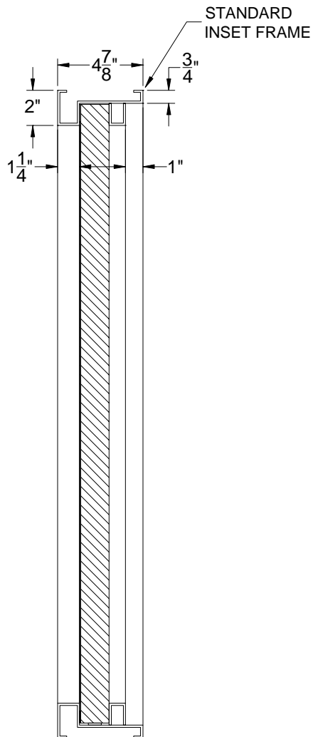
VERTICAL SECTION
