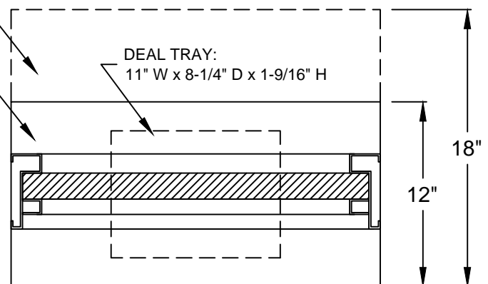
HORIZONTAL SECTION
