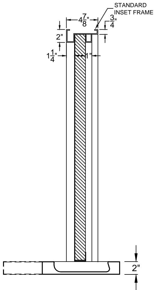
VERTICAL SECTION
