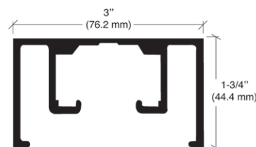
D1670 OVERHEAD TRACK When Matching a Store Front Extrusion, D1670 Upper Track may be used. Specify D1026 Assembly
