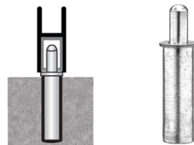
SPRING-LOADED D35 GUIDE
