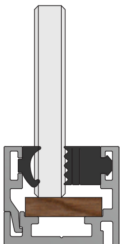
5/16" glass
