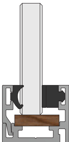
3/8" glass
