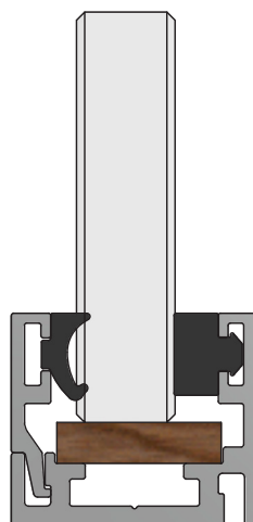
1/2" glass
