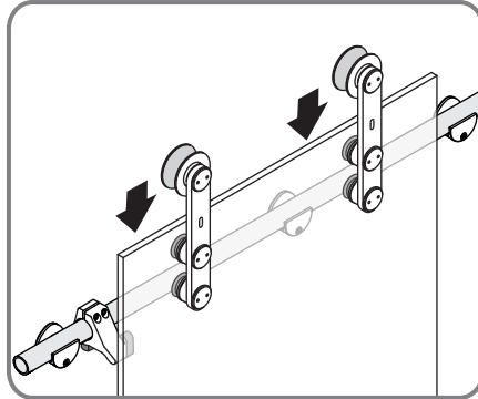
Place Top Rollers onto Tube.
