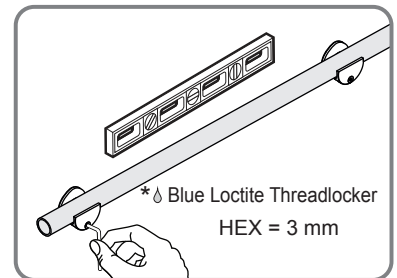
Level Tube and tighten Glass Clamps.
