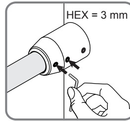
Ensure Sliding Tube is level. Tighten Set Screws in Wall Mount and Glass Clamps.
