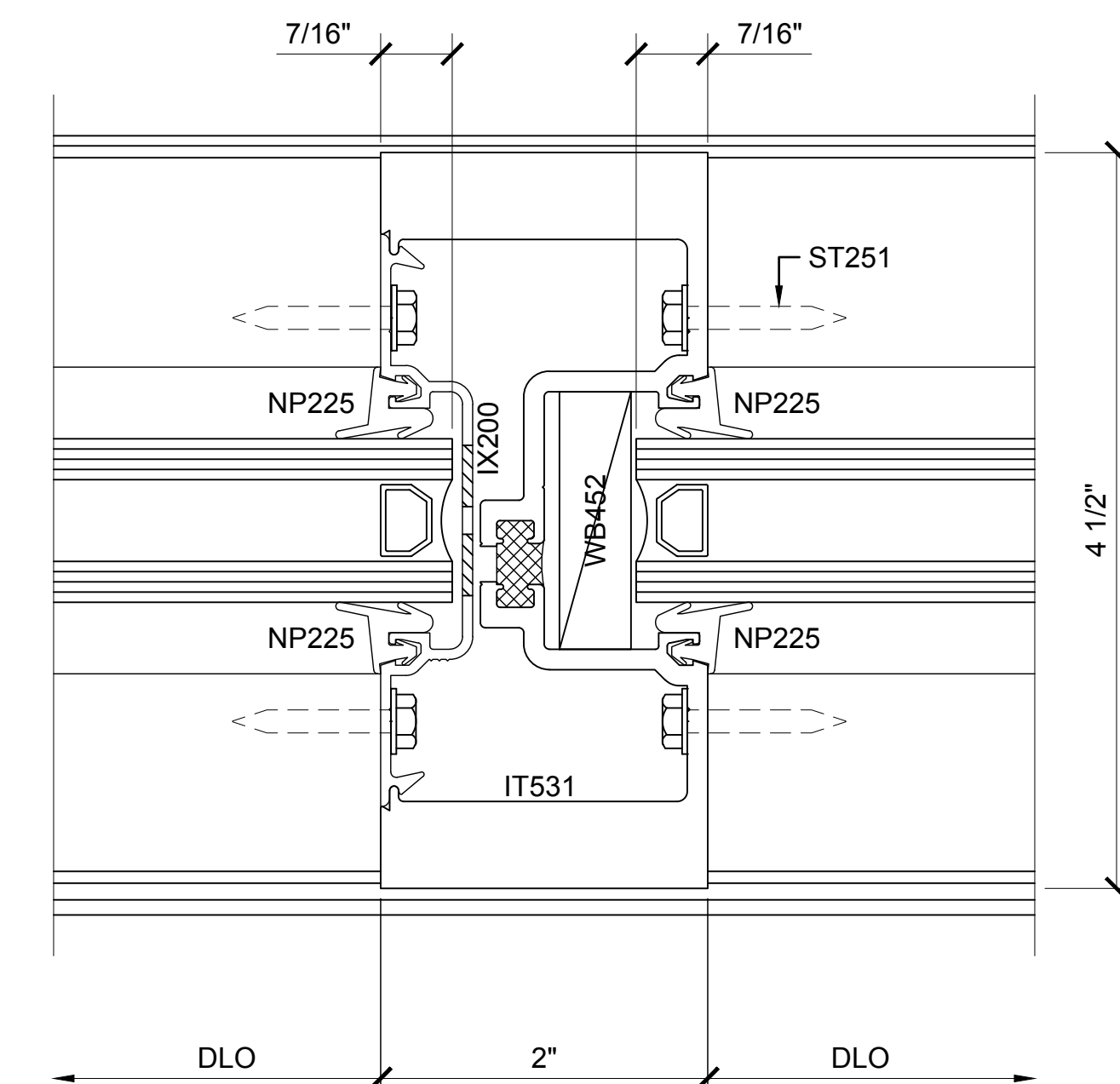
SECTION DETAIL AT INTERMEDIATE VERTICAL ⑧
