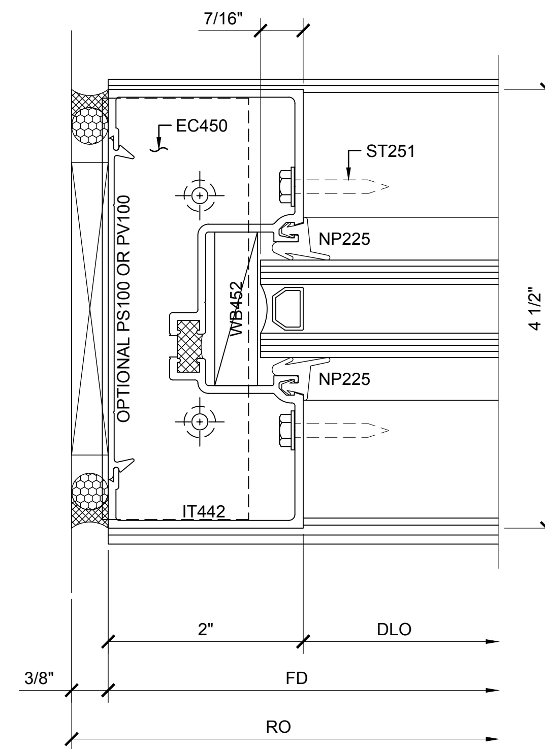
SECTION DETAIL AT JAMB
