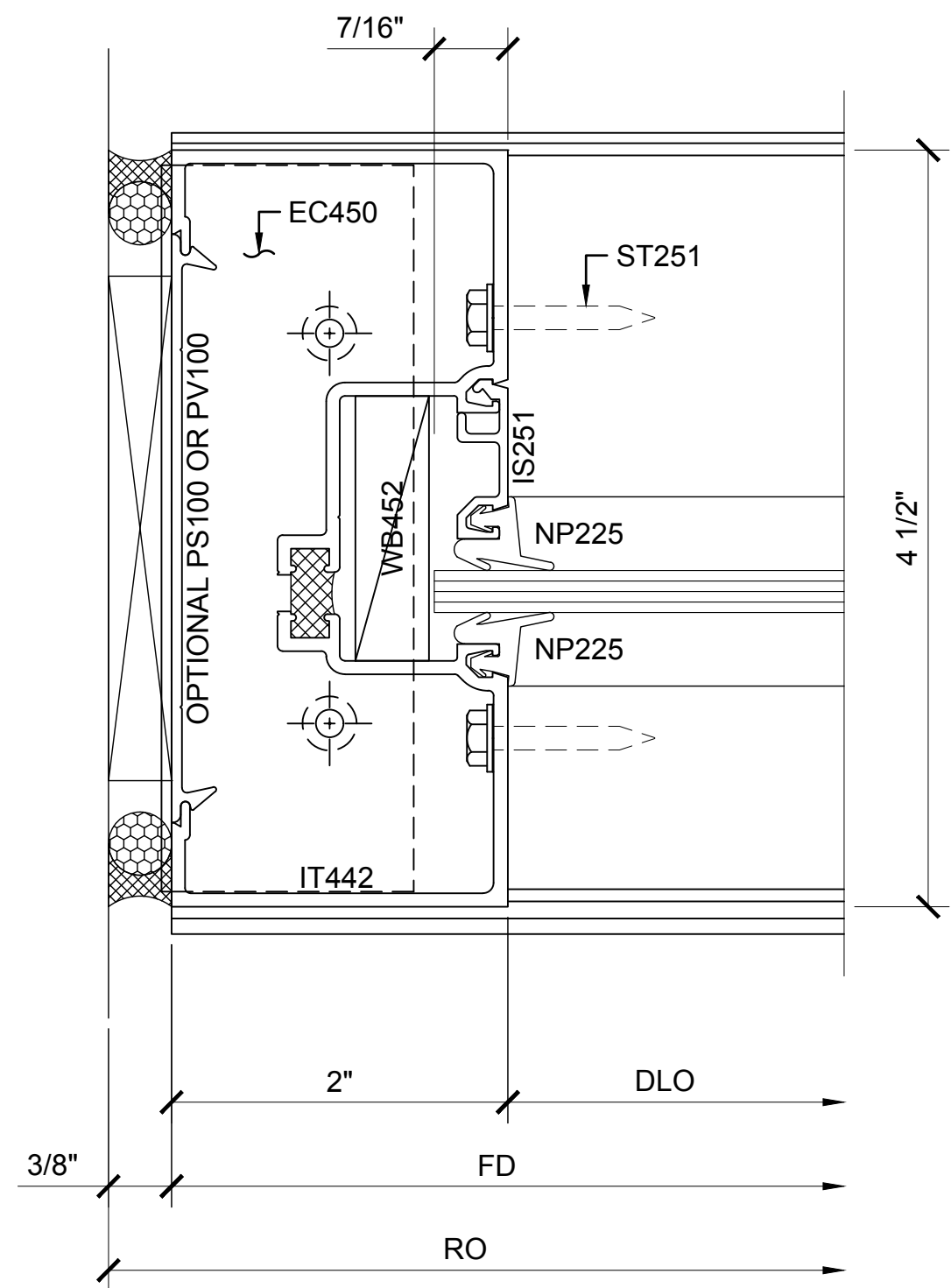
SECTION DETAIL AT JAMB 1 1/4" GLASS - OFFSET EXTERIOR
