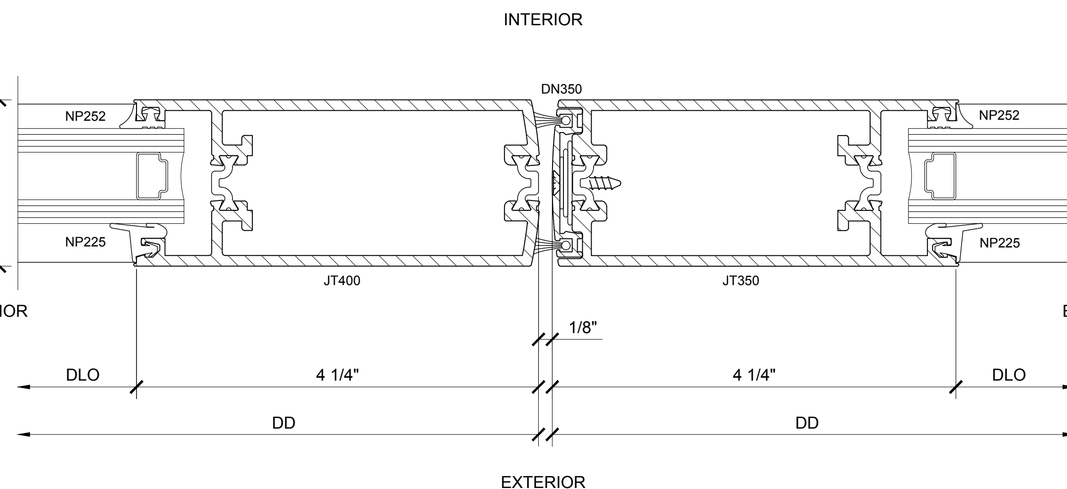
SECTION DETAIL @ MEETING STILES
