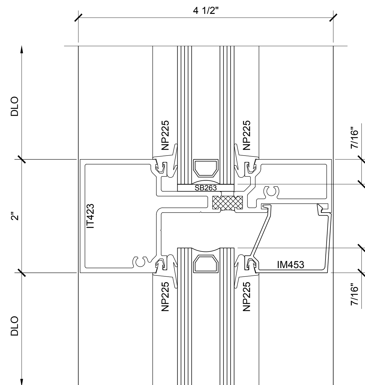
SECTION DETAIL AT INTERMEDIATE HORIZONTAL
