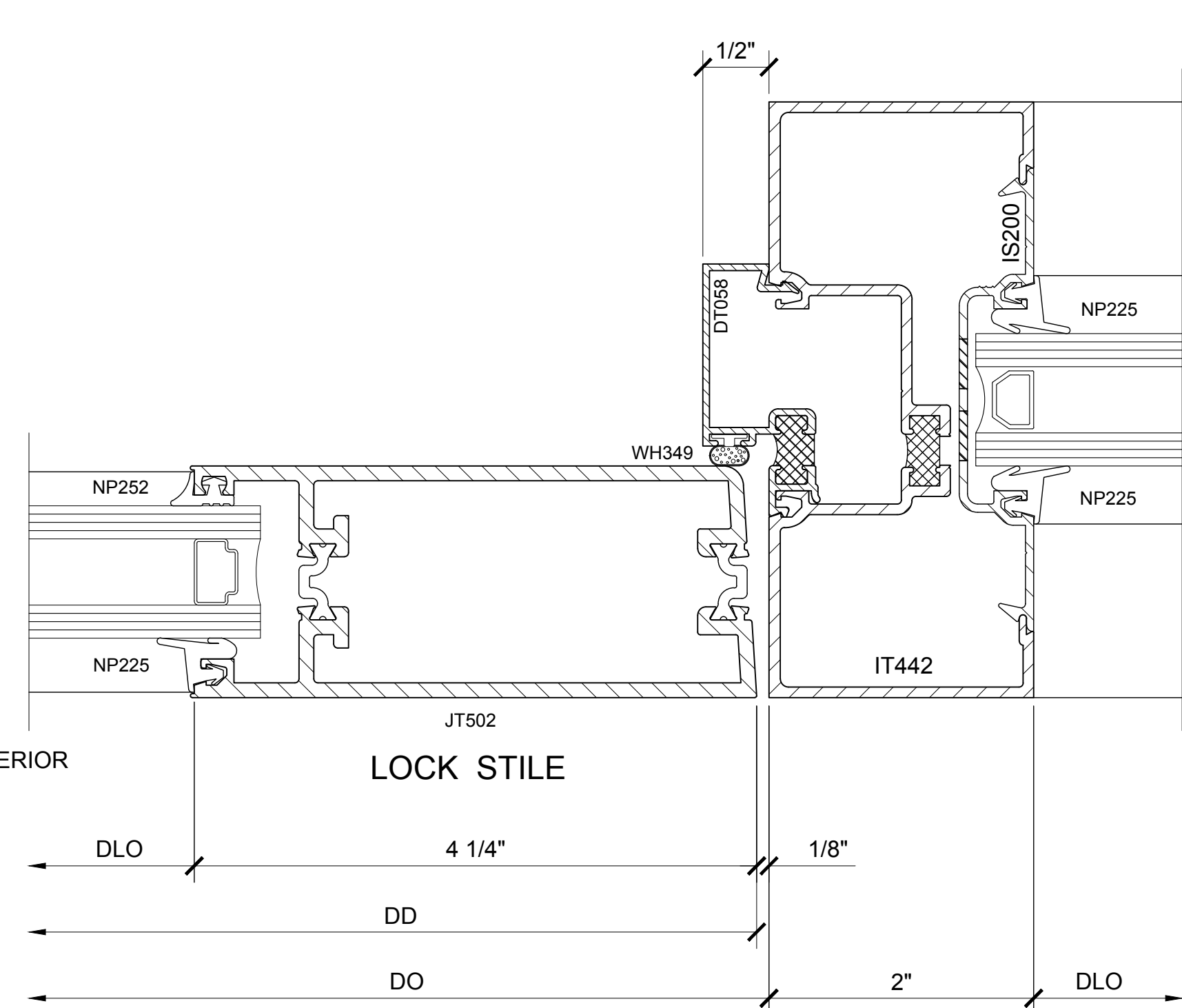
SECTION DETAIL @ DOOR JAMB (LOCK STILE FOR SINGLE DOOR)
