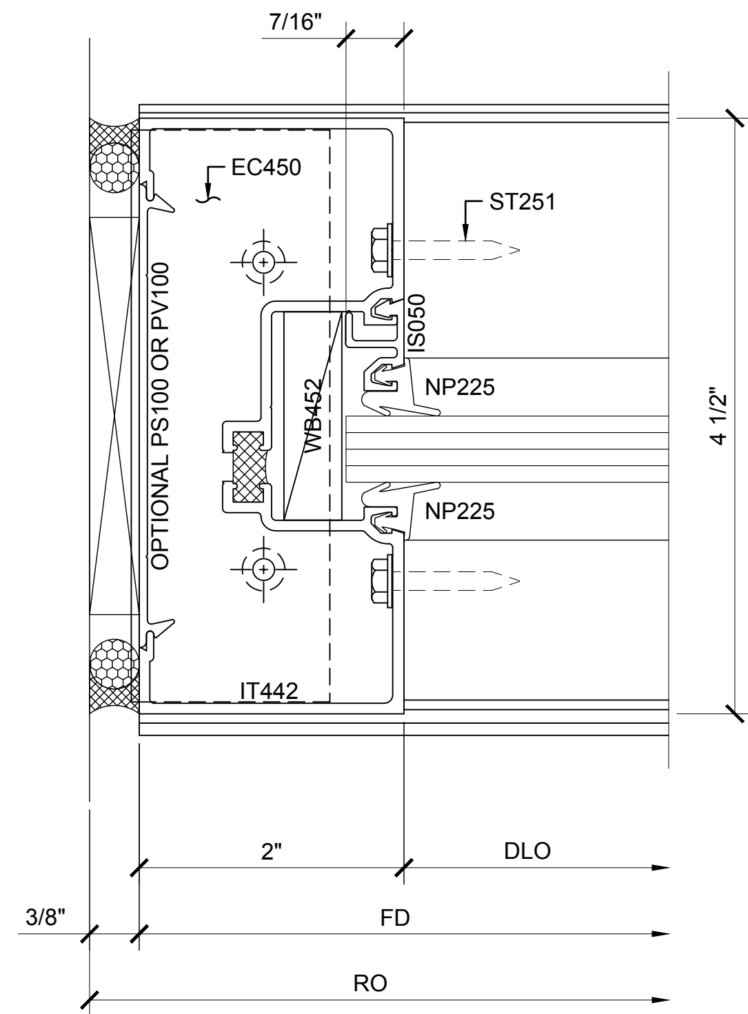
SECTION DETAIL AT JAMB ① 1/2" GLASS - OFFSET EXTERIOR
