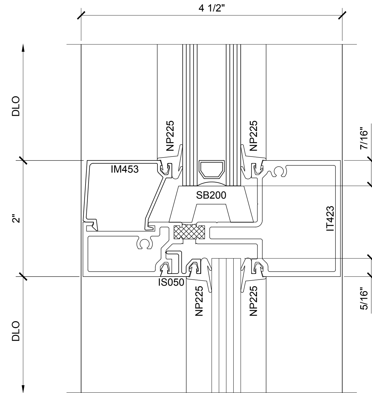
SECTION DETAIL AT INTERMEDIATE HORIZONTAL 6 1/2" GLASS - OFFSET INTERIOR
