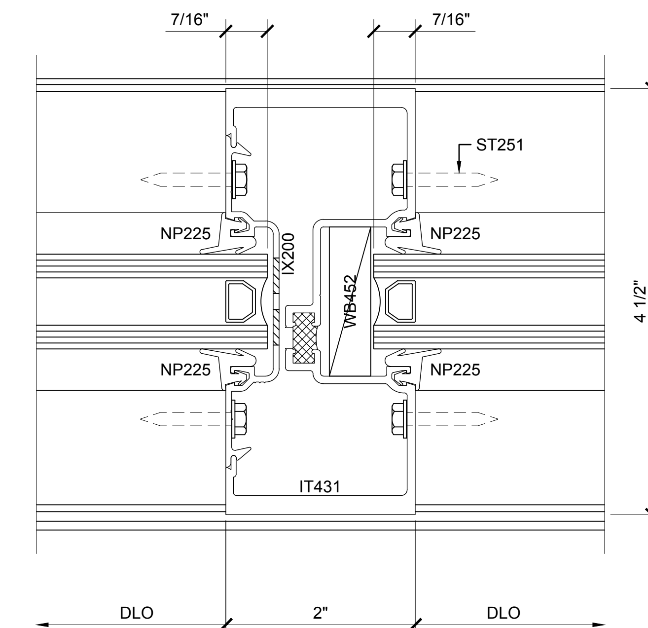
SECTION DETAIL AT INTERMEDIATE VERTICAL ⑦
