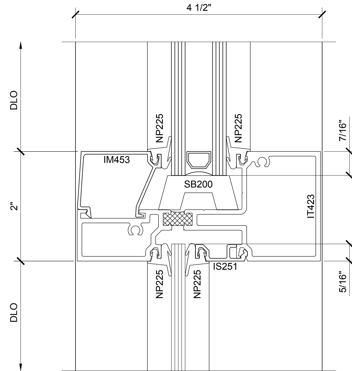
SECTION DETAIL AT INTERMEDIATE HORIZONTAL 5 1/4" GLASS - OFFSET EXTERIOR
