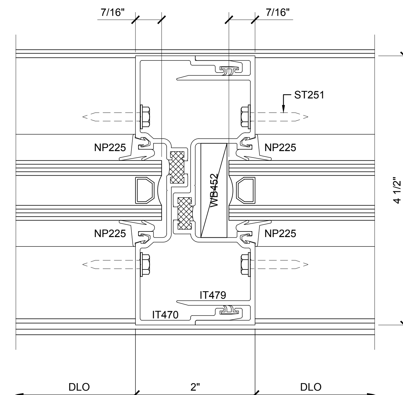
SECTION DETAIL AT EXPANSION MULLION
