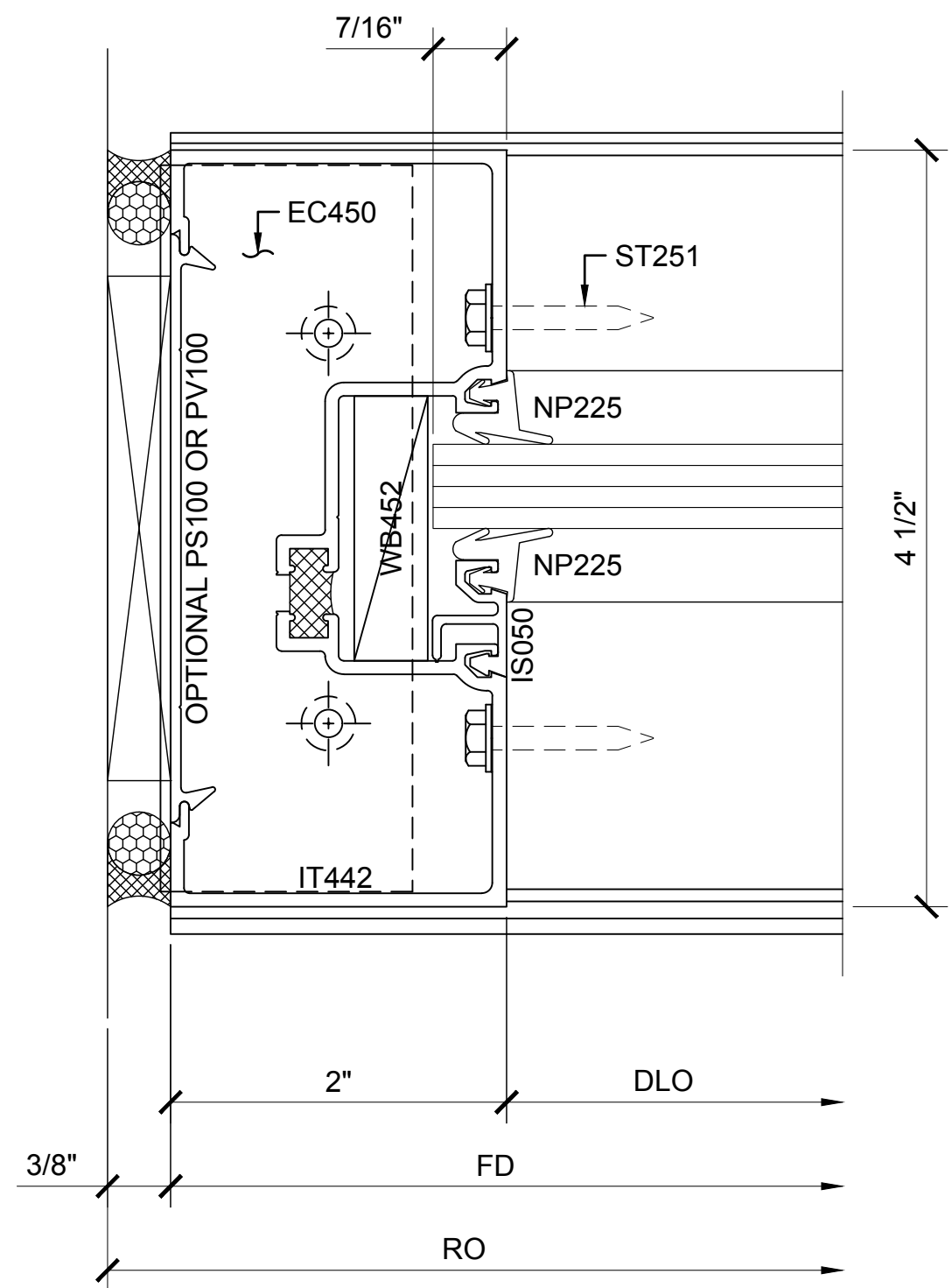
SECTION DETAIL AT JAMB ② 1/2" GLASS - OFFSET INTERIOR
