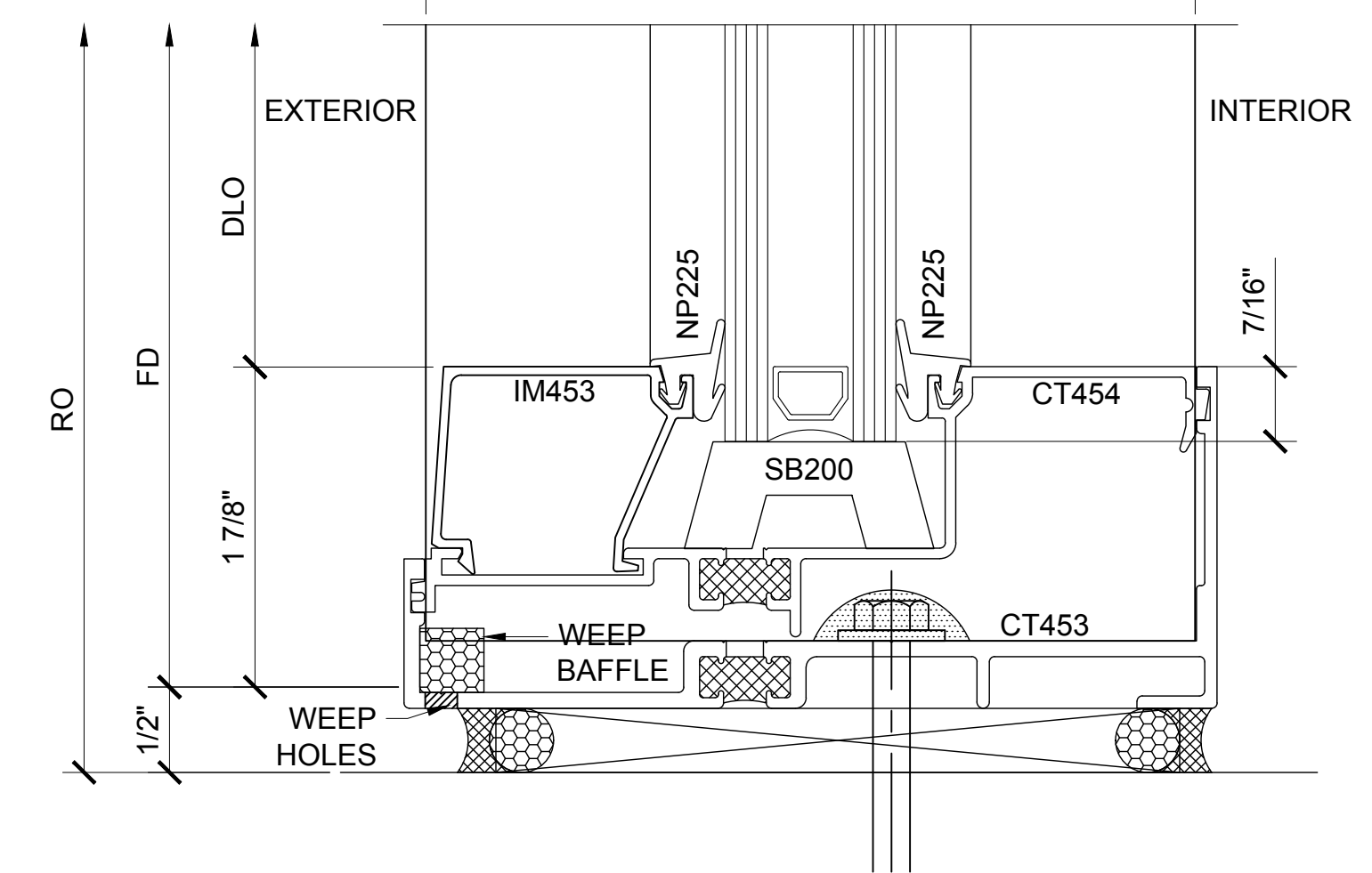
SECTION DETAIL AT SILL ④
