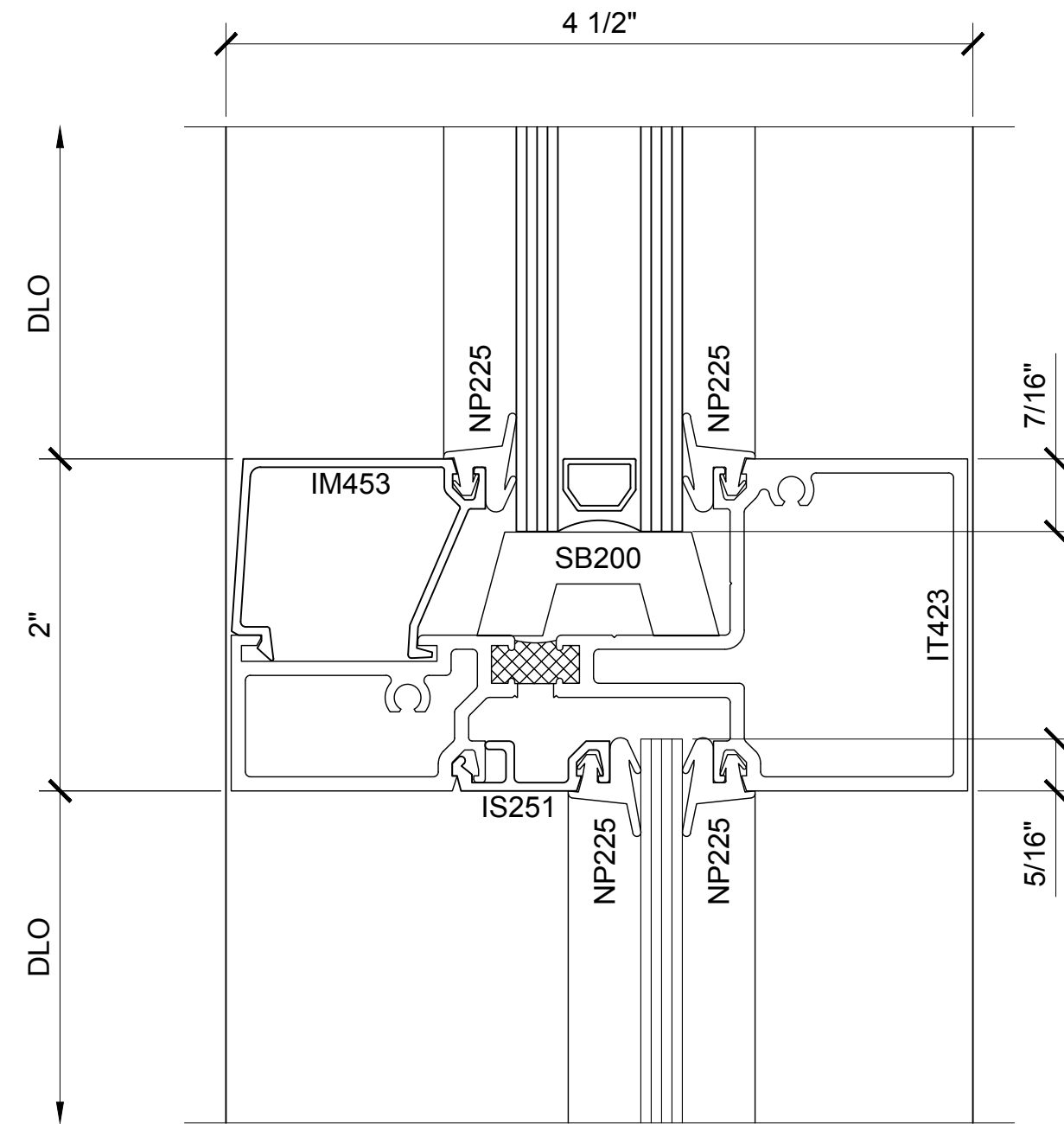
SECTION DETAIL AT INTERMEDIATE HORIZONTAL 6 1/4" GLASS - OFFSET INTERIOR
