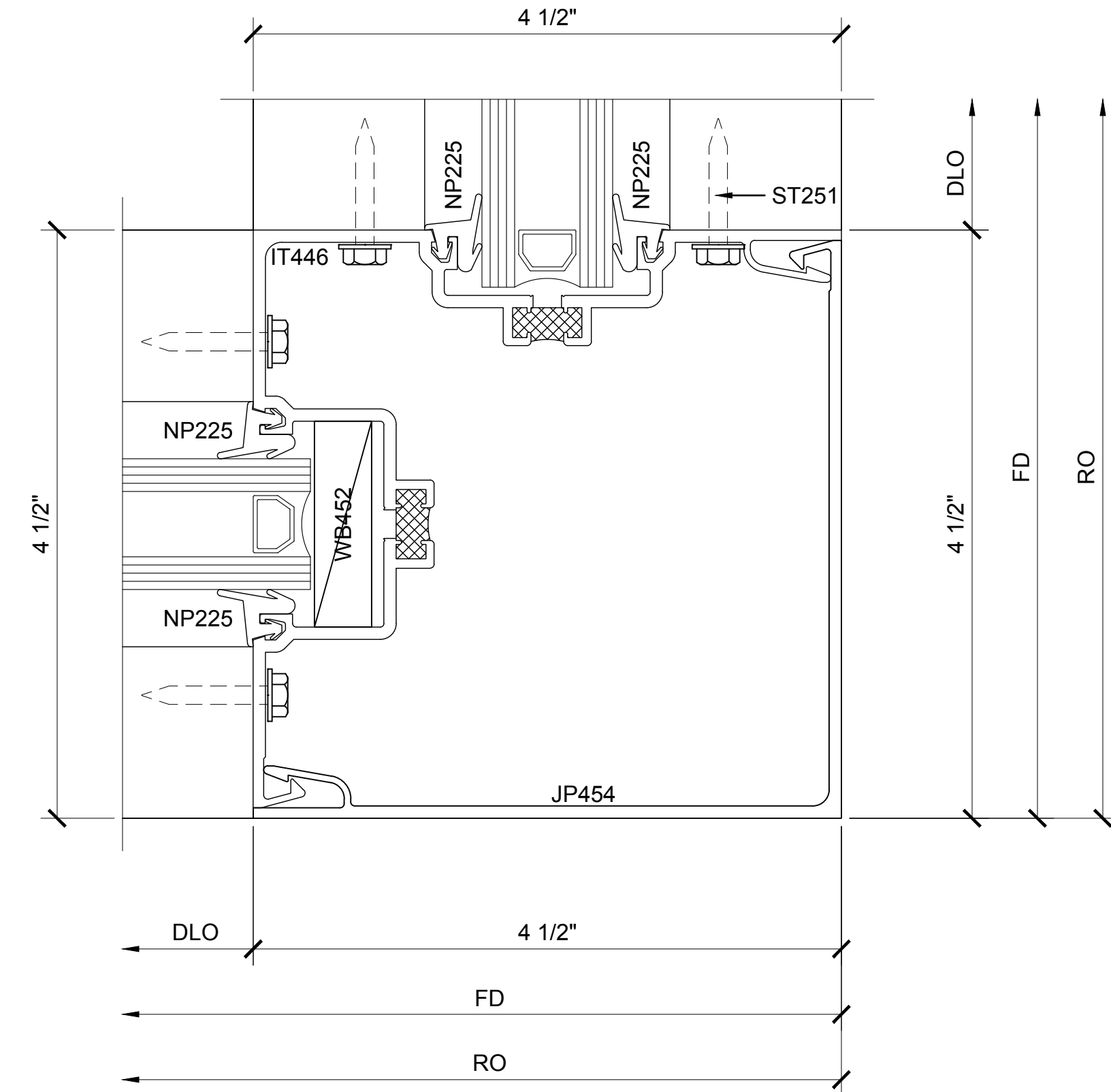
SECTION DETAIL AT WIDE STYLE CORNER VERTICAL ③
