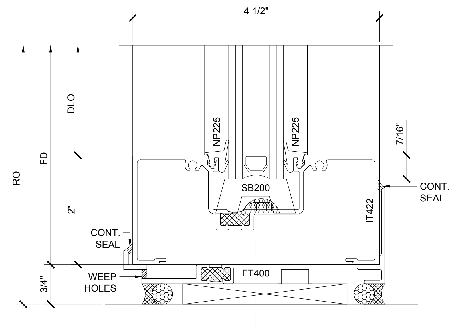
SECTION DETAIL AT SILL
