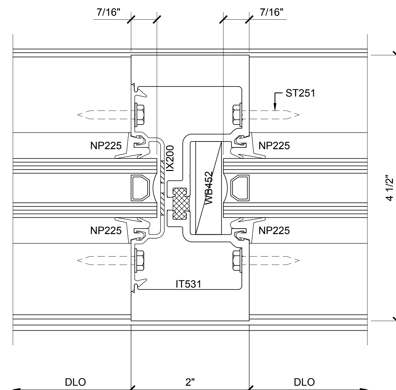
SECTION DETAIL AT INTERMEDIATE VERTICAL
