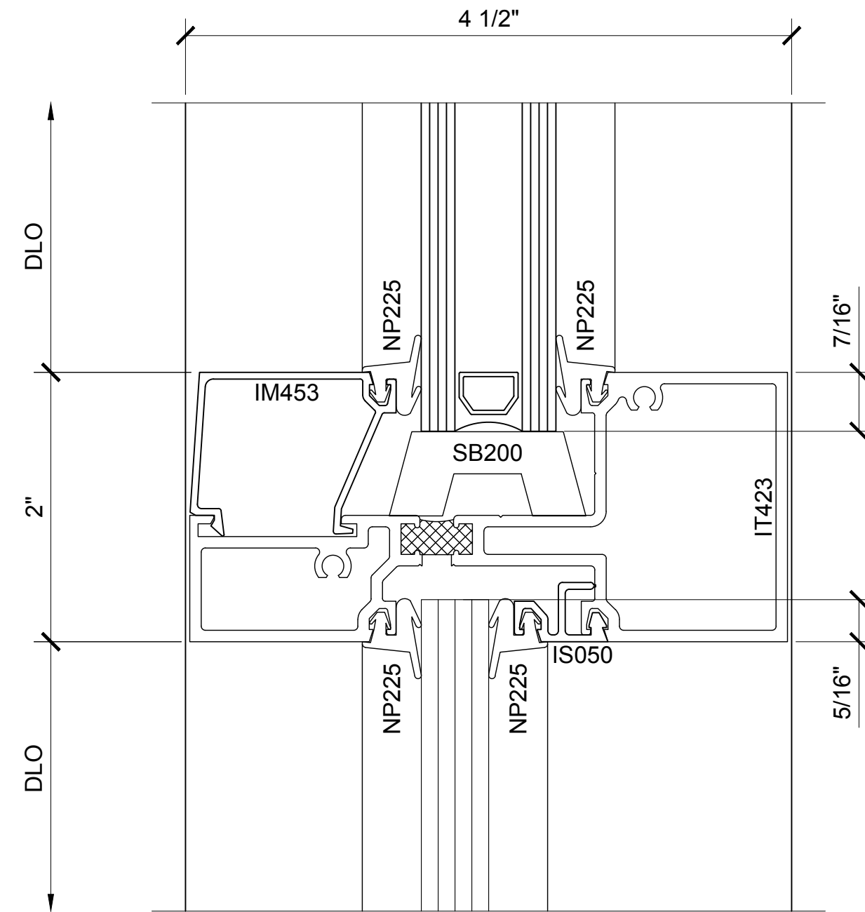
SECTION DETAIL AT INTERMEDIATE HORIZONTAL 5 1/2" GLASS - OFFSET EXTERIOR
