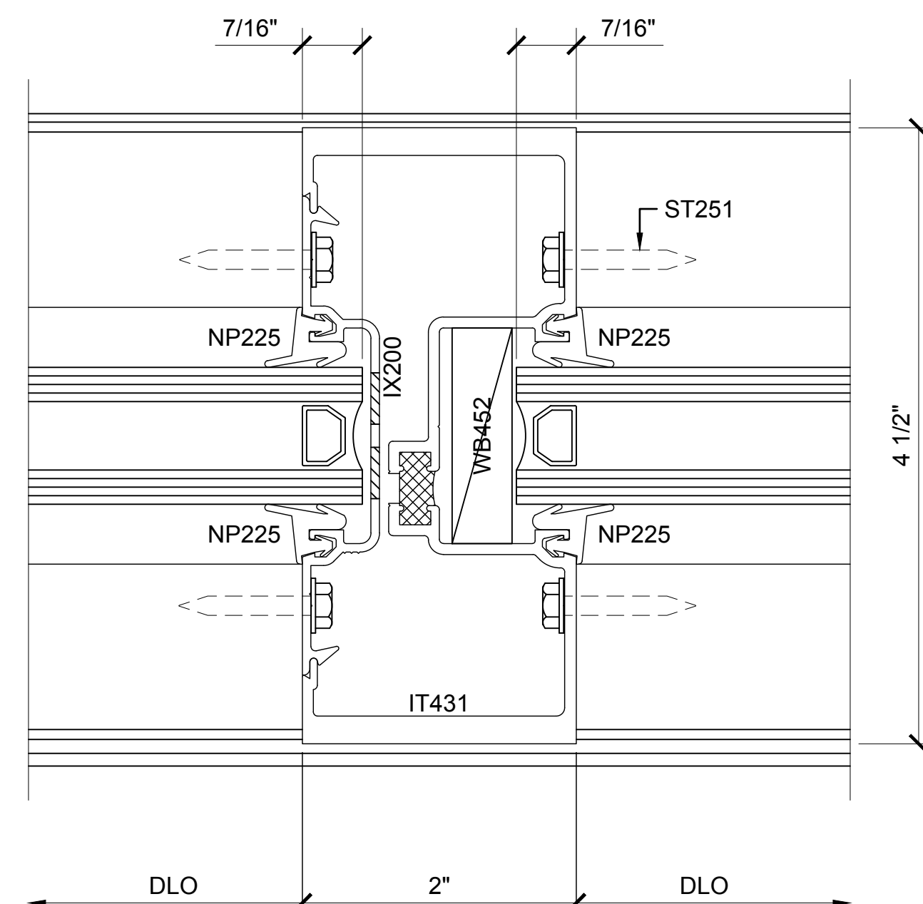
SECTION DETAIL AT INTERMEDIATE VERTICAL
