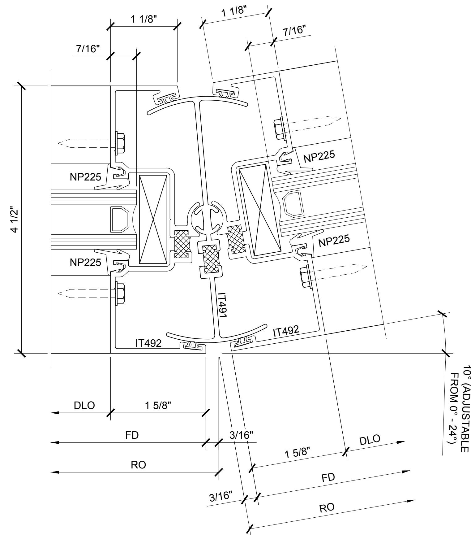
SECTION DETAIL AT ADJUSTABLE ANGLE POST COVER
