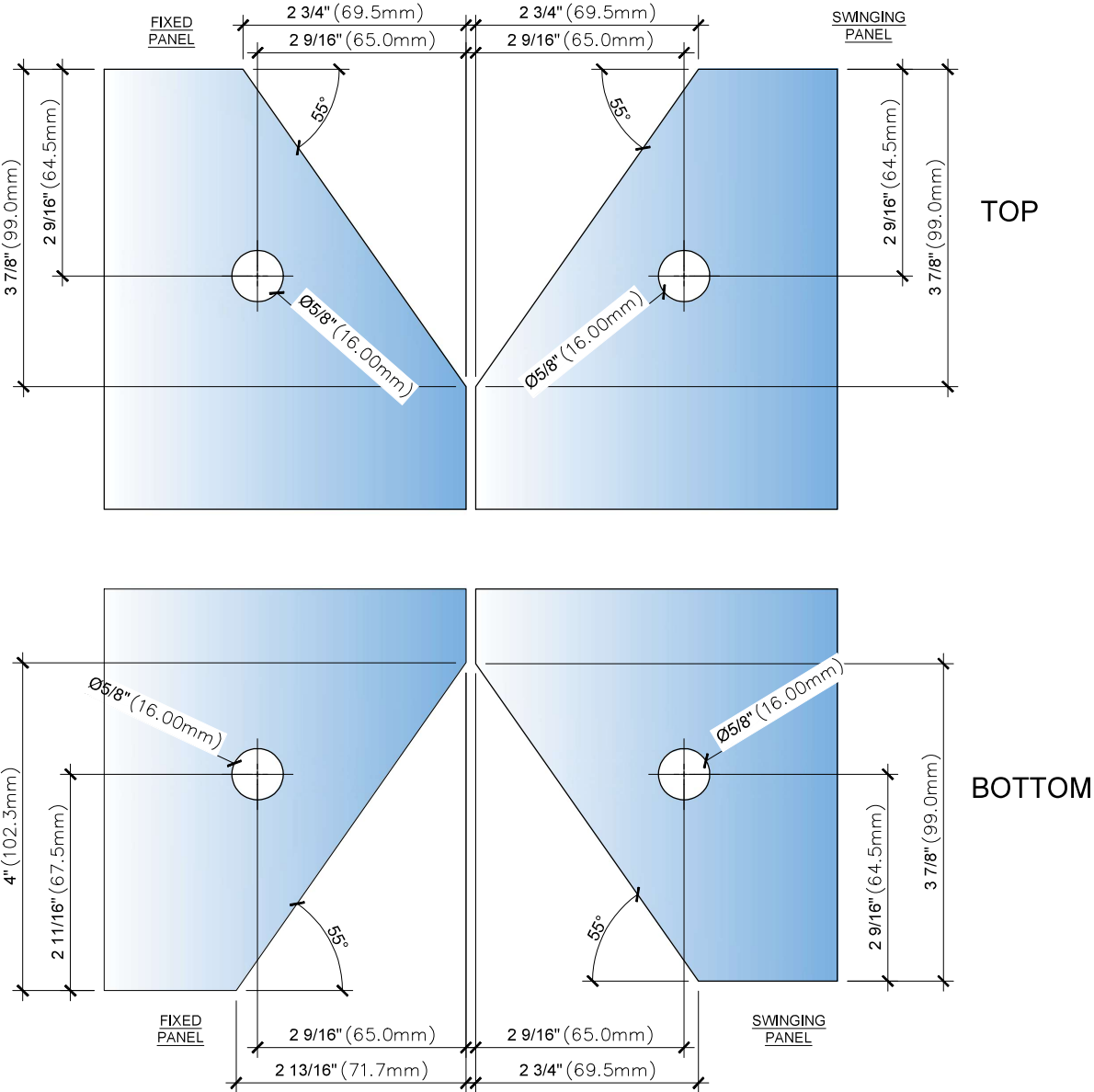
3A GLASS CUT OUT DETAIL - 1MM FIXED PANEL GAP
