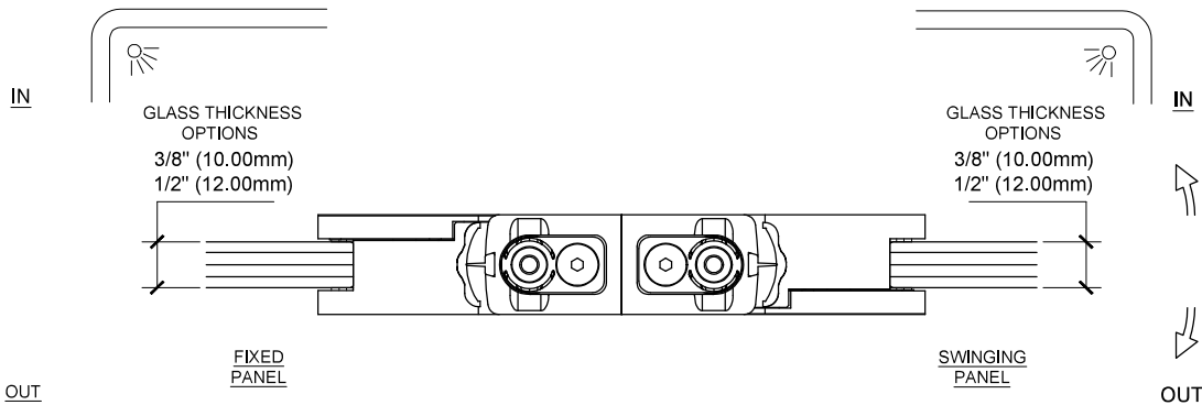
1 PLAN VIEW DETAIL
