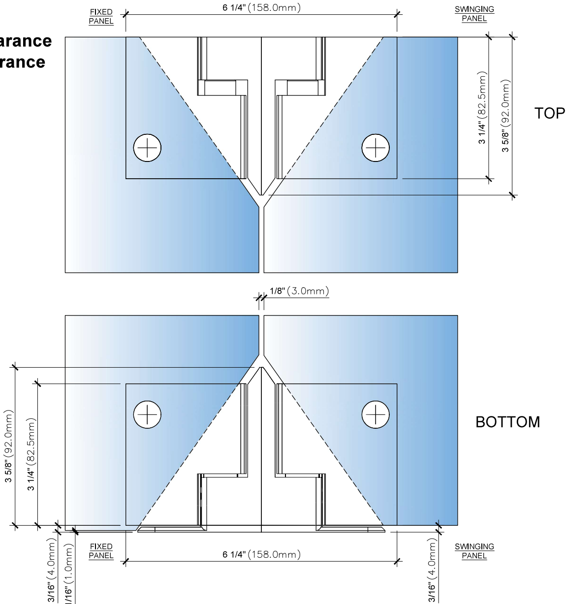
2A FRONT VIEW DETAIL -1MM FIXED PANEL GAP
