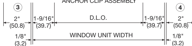
ANCHOR CLIP ASSEMBLY
