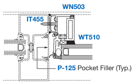
ANCHOR CLIP ASSEMBLY
