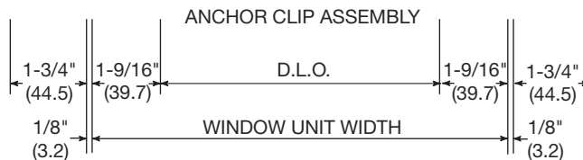
ANCHOR CLIP ASSEMBLY
