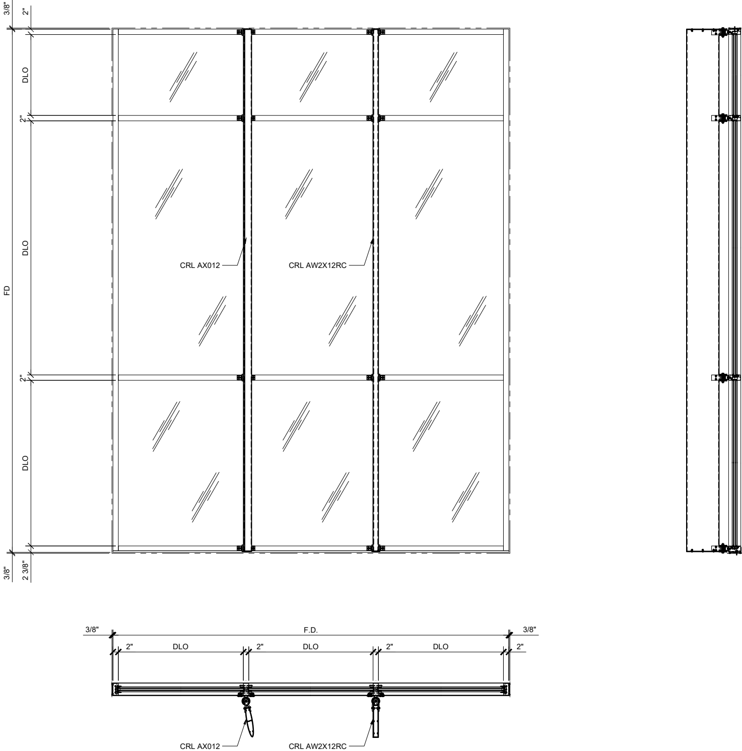
① 451 (INTERIOR GLAZING) STOREFRONT 8010 SERIES SUNSHADE 3/4"=1'-0"
