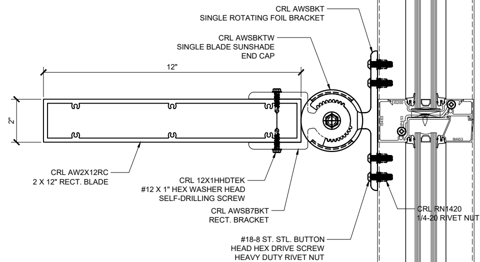
A SECTION VIEW DETAIL (451 INT. GLAZING STOREFRONT) 6"=1'-0"
