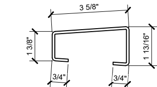
⑪ CRL AWSB6CSM ALUMINUM 6"=1'-0"
