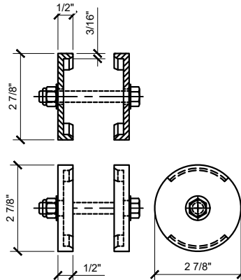
⑩ CRL AWSBKTW ALUMINUM 6"=1'-0"
