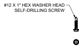
⑭ CRL 12X1HHDTEK STAINLESS STEEL 6"=1'-0"
