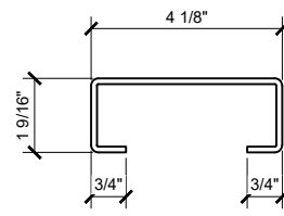
⑫ CRL AWSB7CSM ALUMINUM 6"=1'-0"
