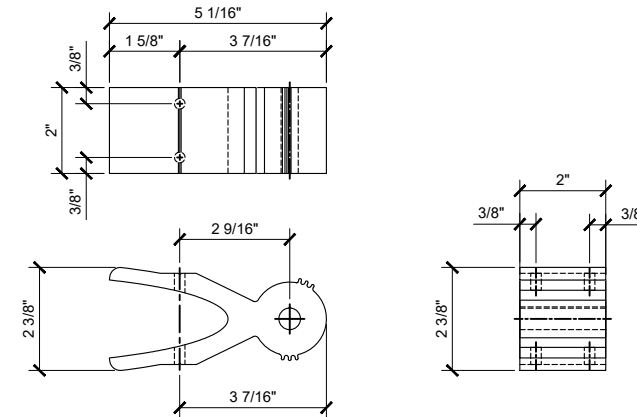
⑤ CRL AWSB6BKT ALUMINUM 6"=1'-0"
