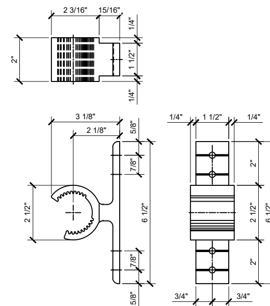
⑦ CRL AWSBKT ALUMINUM 6"=1'-0"
