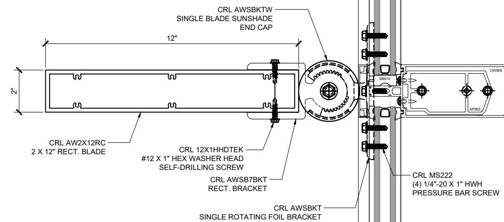
B SECTION VIEW DETAIL (3252HP CURTAINWALL) 6"=1'-0"
