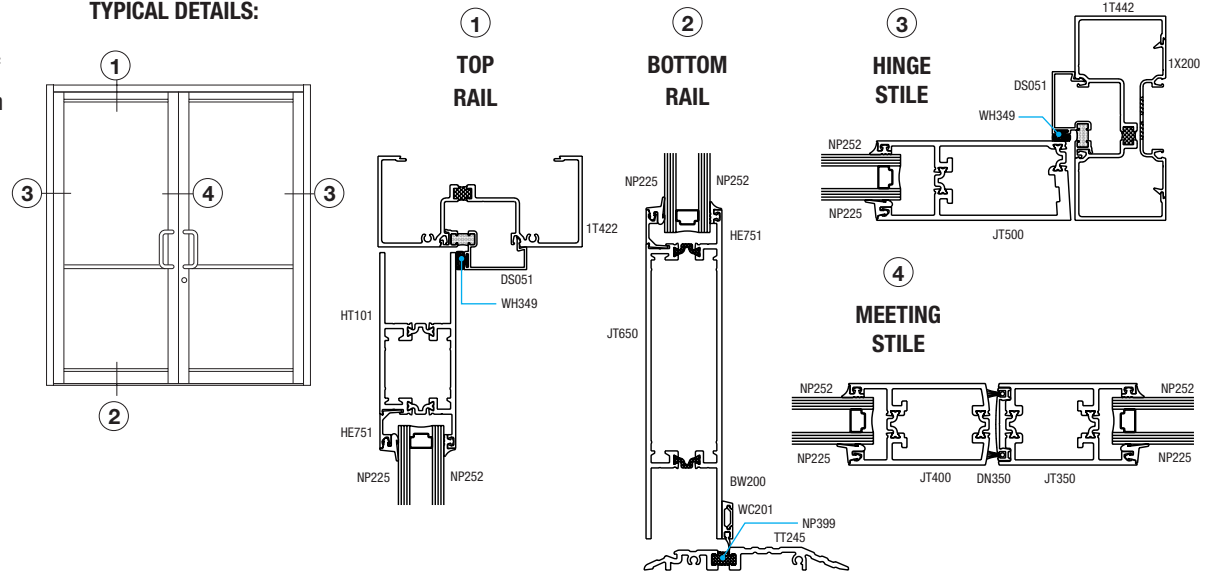
TYPICAL DETAILS:
