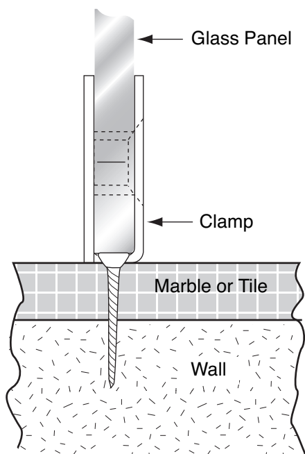
END VIEW
