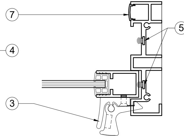
PLAN @ HANDLE
