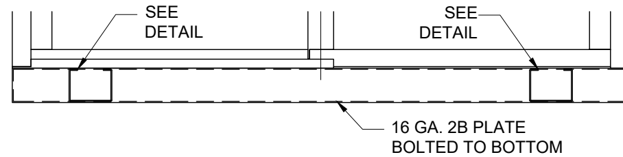
ELEVATION: INTERNAL 16 GA. SHELF SUPPORTS
