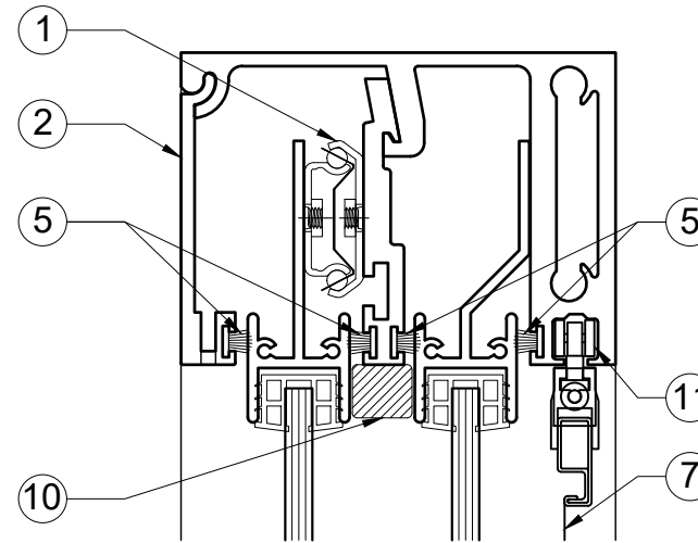
PLAN @ HANDLE
