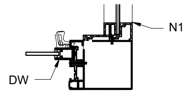
BRAKE METAL INSERT FOR 90 DEG. RETURNS
