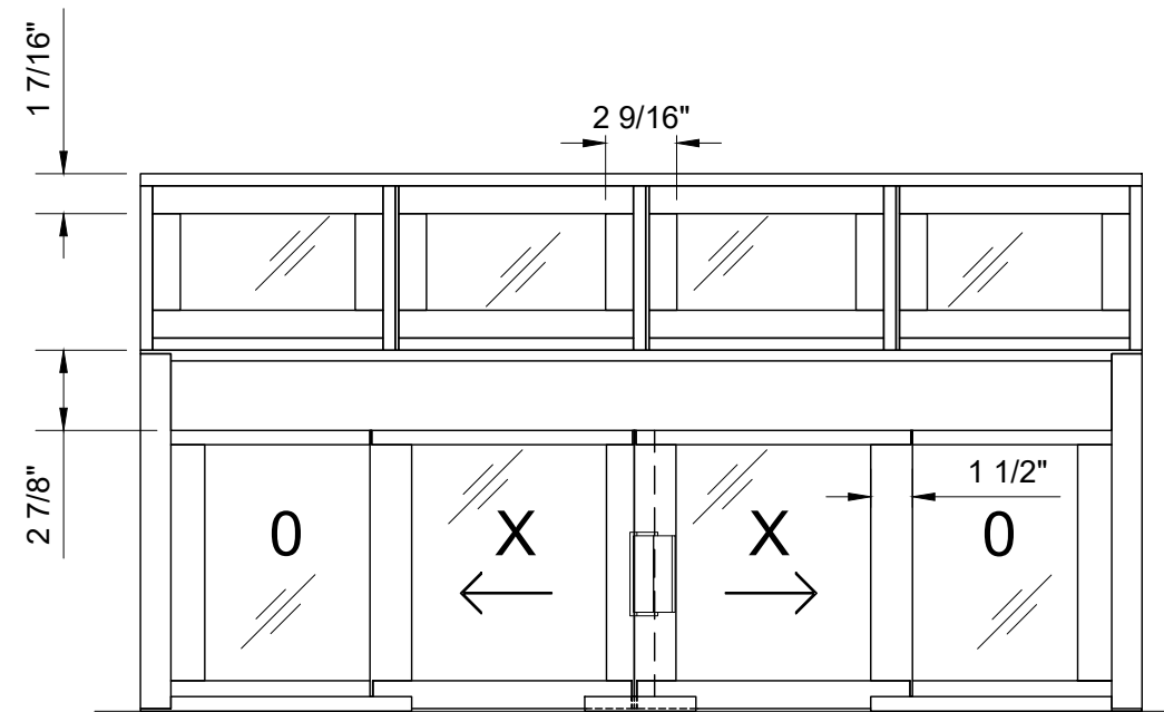
DW3400 MULTI-LITE TRANSOM
