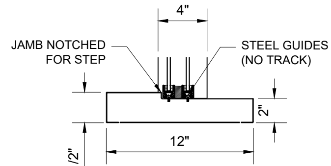
STAINLESS STEEL SHELF WITH 1/2" STEP FOR WATER DAM
