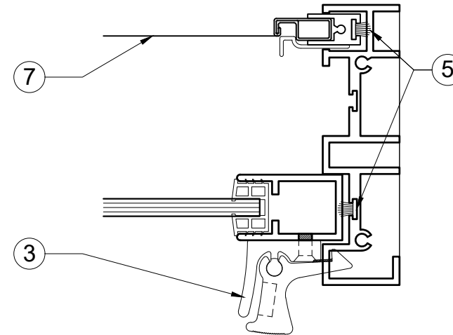
PLAN @ HANDLE
