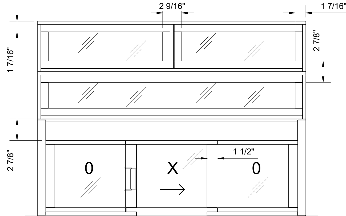
DW2600 CUSTOM TRANSOM
