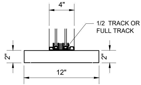
FLAT STAINLESS STEEL SHELF 16 GA. BRUSHED # 4 FINISH
