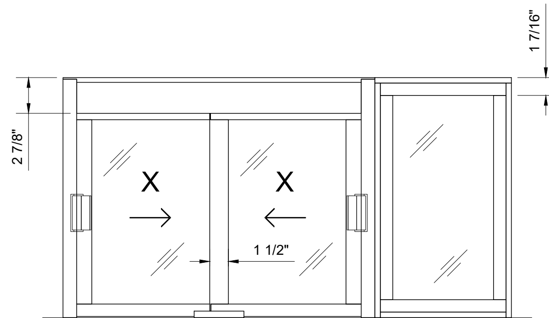
DW4200 180 DEG. SIDE LITE
