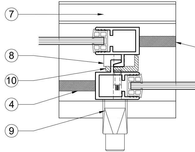
* KEYED LOCK PLAN
