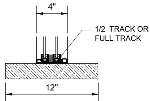
PLASTIC LAMINATE SHELF STANDARD BLACK OR SPECIFY WILSONART COLOR #
