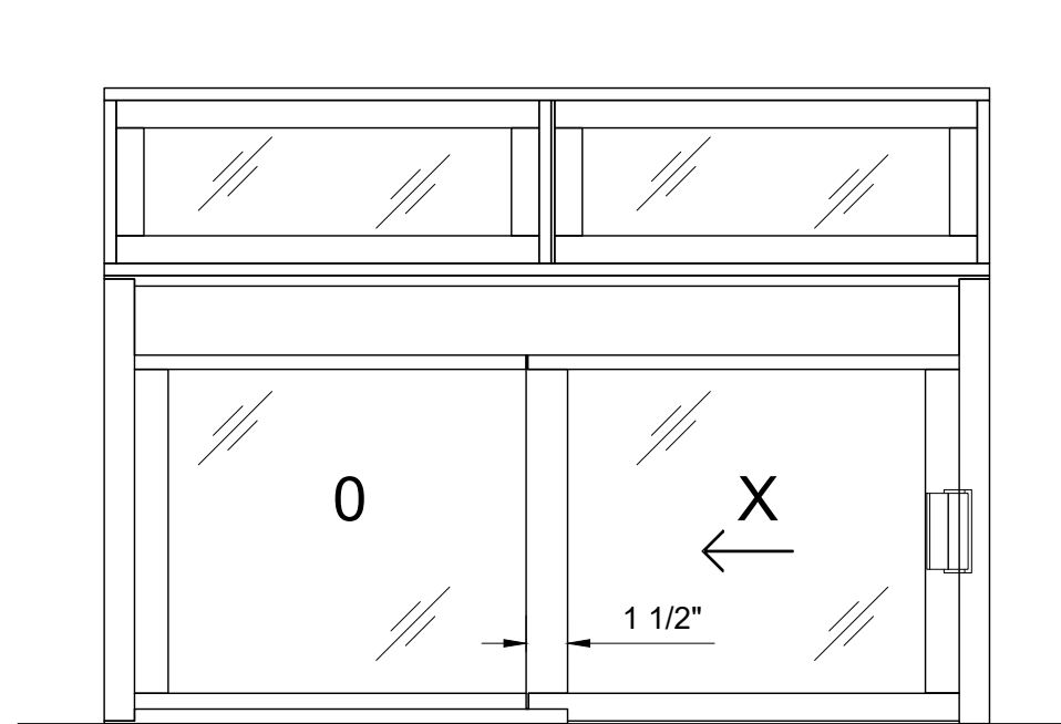
ELEVATION: DW1800 2-LITE TRANSOM
