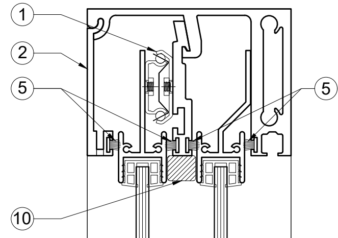
MEETING STILE PLAN
