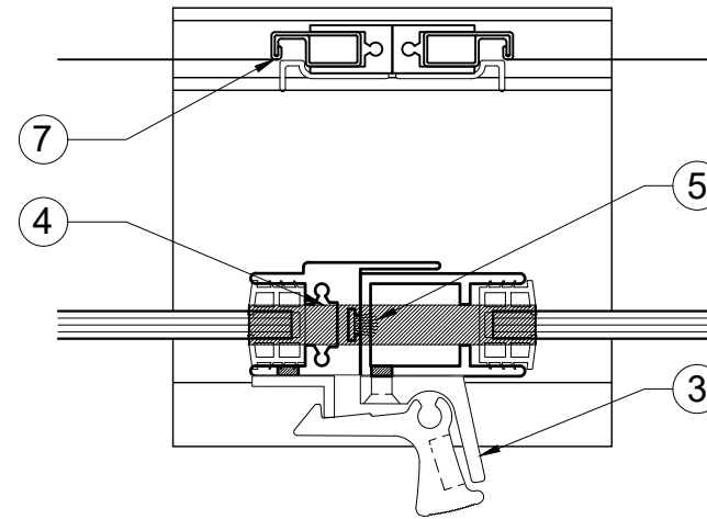
MEETING STILE PLAN
