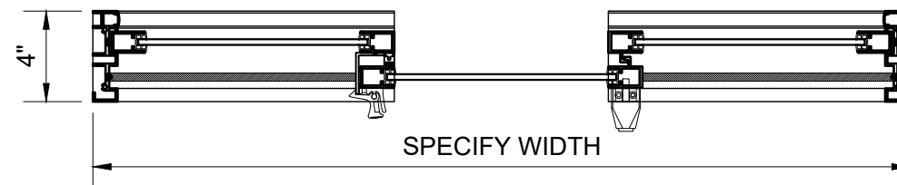
PLAN
