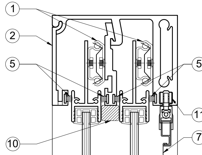
PLAN @ HANDLE
