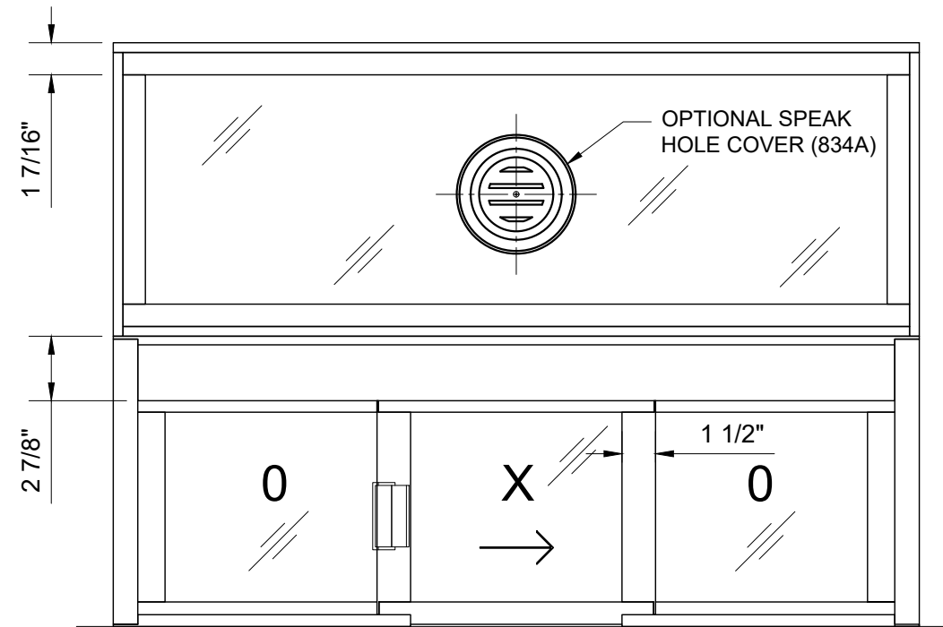
DW2600 SINGLE-LITE TRANSOM
