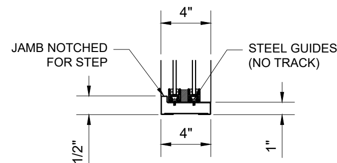
STAINLESS STEEL SILL WITH 1/2" STEP FOR WATER DAM
