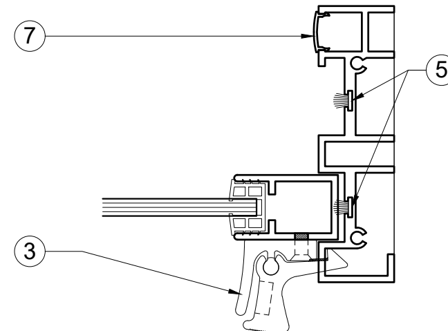
PLAN @ HANDLE
