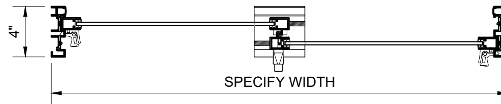
PLAN
