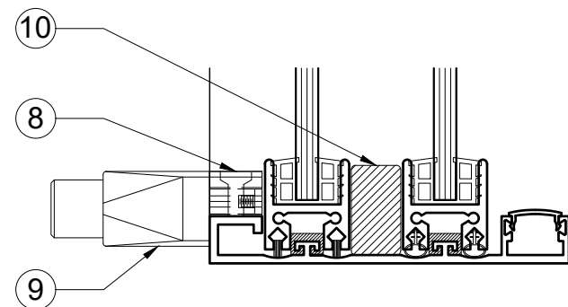
* KEYED LOCK SECTION
