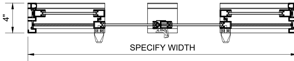
PLAN
