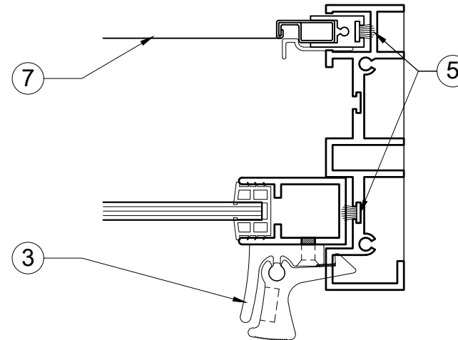
PLAN @ HANDLE
