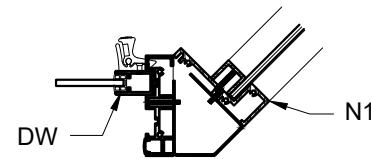
BRAKE METAL INSERT FOR CUSTOM ANGLE RETURNS
