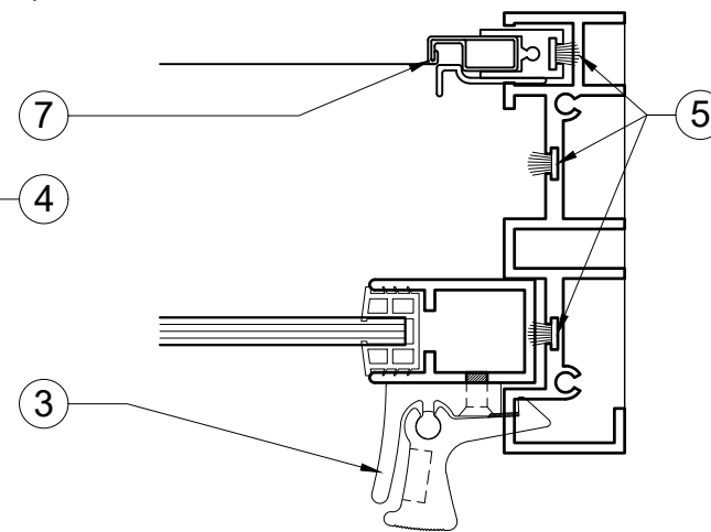
PLAN @ HANDLE
