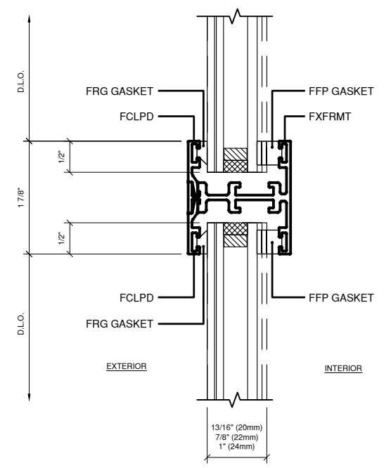
5 HORIZONTAL DETAIL @ FRAME XL 20-24.76 1'-0" = 1'-0" ARCH. REF.: -/-
