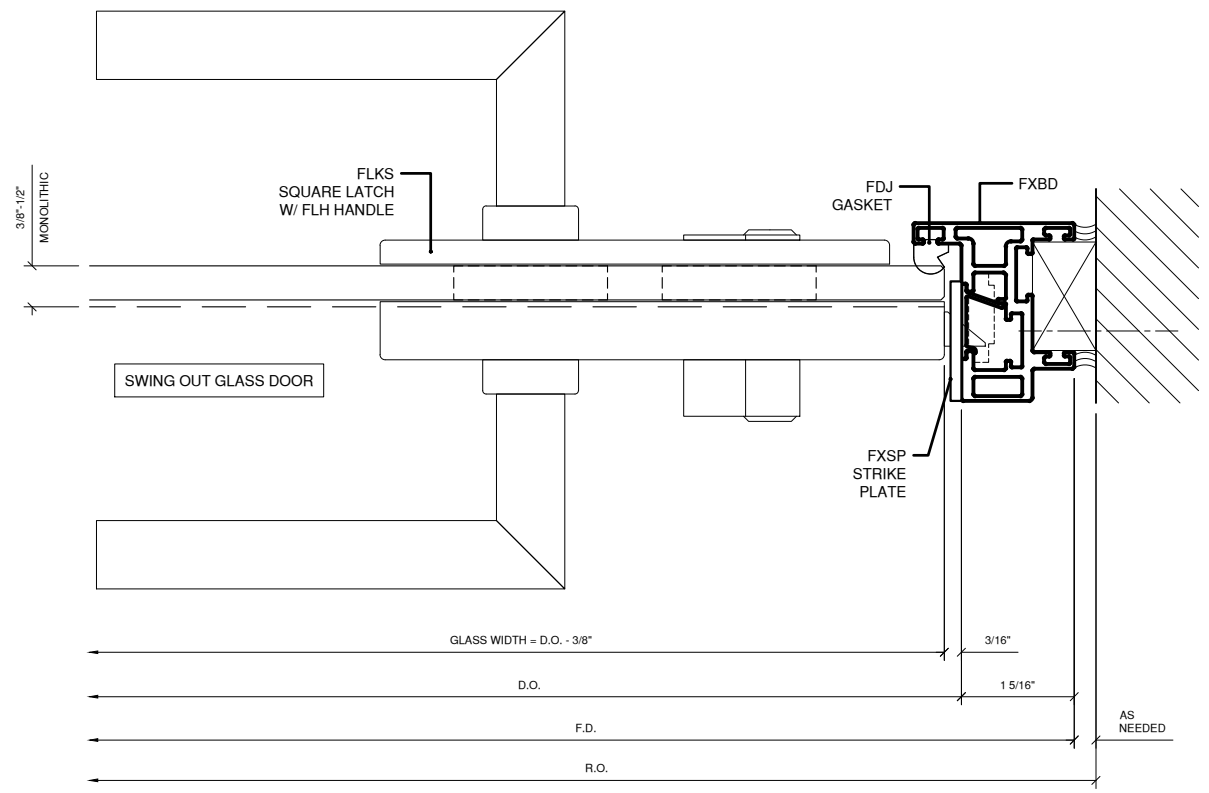
4 DOOR JAMB DETAIL @ LOCK 1'-0" = 1'-0" ARCH. REF.: -/-
