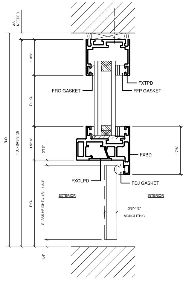
4 DOOR HEAD DETAIL W/ TRANSOM 1'-0" = 1'-0" ARCH. REF.: -/-
