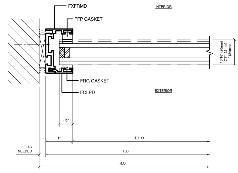
1 JAMB DETAIL @ FRAME XL 20-24.76 1'-0" = 1'-0" ARCH. REF.: -/-
