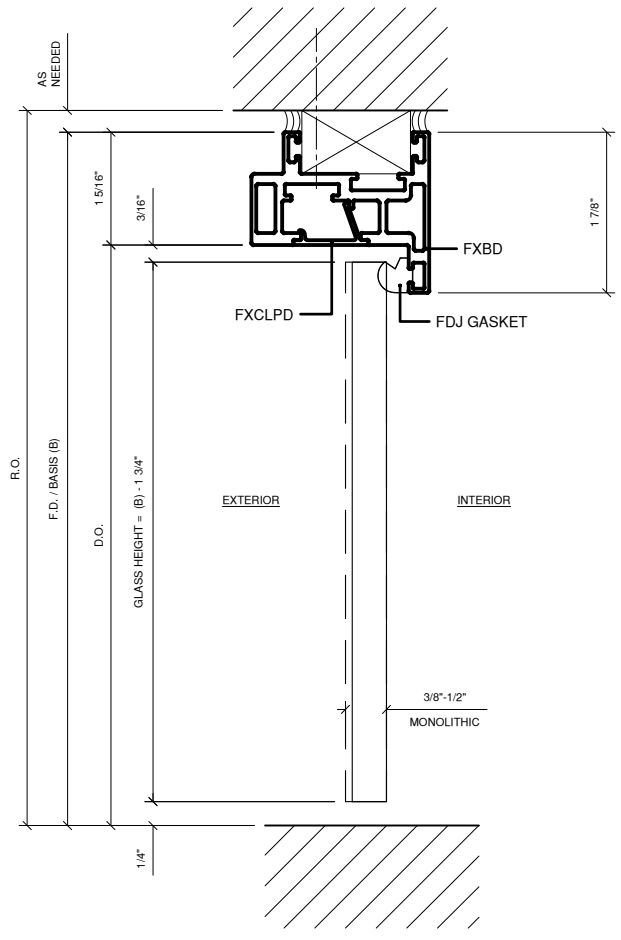
3 DOOR HEAD DETAIL W/O TRANSOM 1'-0" = 1'-0" ARCH. REF.: -/-
