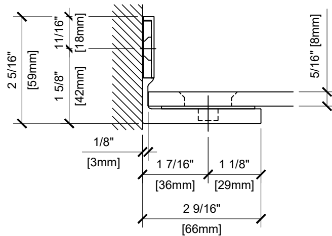
WALL BRACKET (5/16" GLASS)
