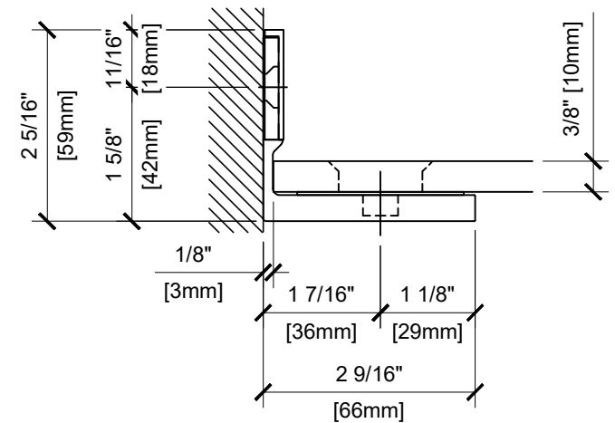
WALL BRACKET (3/8" GLASS)
