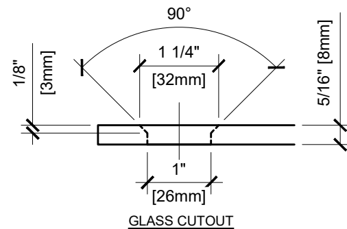
GLASS CUTOUT
